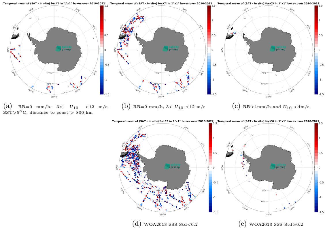
Figure 12: Temporal mean gridded over spatial boxes of size 1^{\circ}\times 1^{\circ} of \Delta\text{SSS} (SMOS SSS L2Q v331 - With FLAG (CMEMS-CATDS-CPDC) - TSG (SAMOS)) for 5 different subdatasets corresponding to: \text{RR}=0 mm/h, 3 < U_{10} < 12 m/s, \text{SST}>5^{\circ}\text{C} , distance to coast > 800 km (a), \text{RR}=0 mm/h, 3 < U_{10} < 12 m/s (b), \text{RR}>1 mm/h and U_{10} < 4 m/s (c), WOA2013 SSS Std < 0.2 (d), WOA2013 SSS Std > 0.2 (e).
