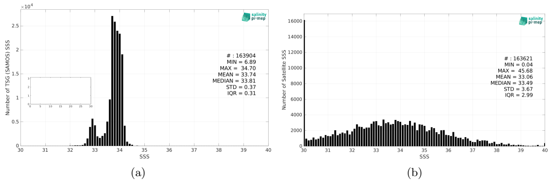
Figure 2: Histograms of SSS from TSG (SAMOS) (a) and SMOS SSS L2Q v331 - With FLAG (CMEMS-CATDS-CPDC) (b) considering all match-up pairs per bins of 0.1 over the Southern Ocean Pi-MEP region and for the full satellite product period.
