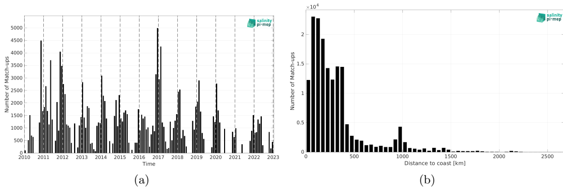
Figure 1: Number of match-ups between TSG (SAMOS) and SMOS SSS L2Q v331 - With FLAG (CMEMS-CATDS-CPDC) SSS as a function of time (a) and as function of the distance to coast (b) over the Southern Ocean Pi-MEP region and for the full satellite product period.
