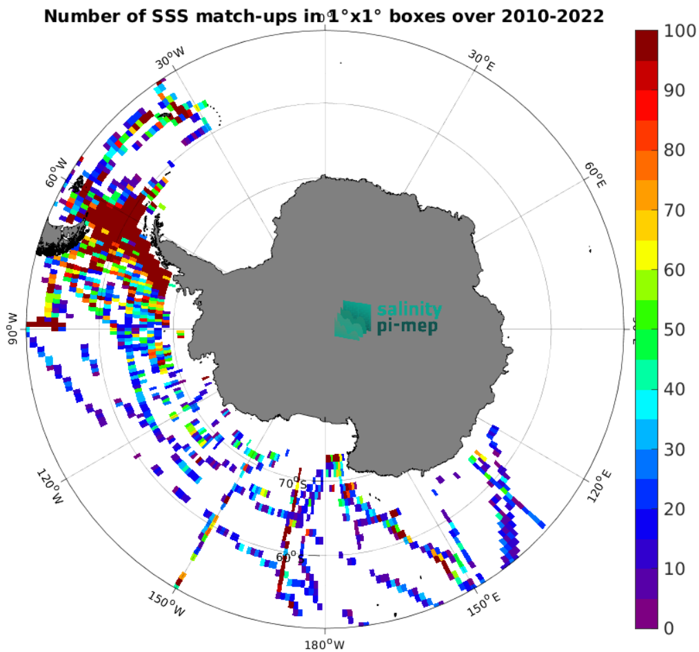
Figure 4: Number of SSS match-ups between TSG (SAMOS) SSS and the SMOS SSS L2Q v331 - With FLAG (CMEMS-CATDS-CPDC) SSS product for the Southern Ocean Pi-MEP region over 1^{\circ} \times 1^{\circ} boxes and for the full satellite product period.
