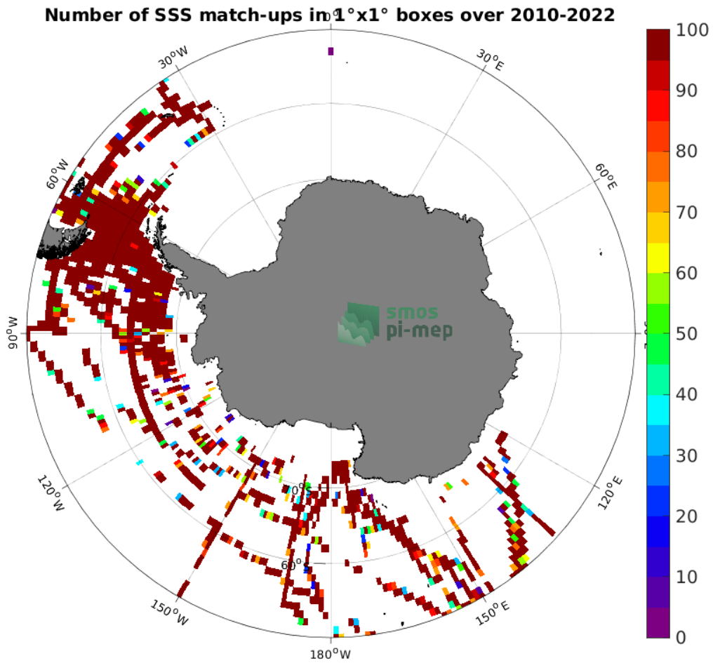
Figure 4: Number of SSS match-ups between TSG (SAMOS) SSS and the SMOS SSS L2Q v331 - With FLAG (CMEMS-CATDS-CPDC) SSS product for the Southern Ocean Pi-MEP region over 1°x1° boxes and for the full satellite product period.
