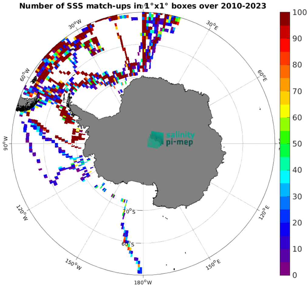
Figure 5: Number of SSS match-ups between TSG (Polarstern) SSS and the SMOS SSS L2Q v331 - With FLAG (CMEMS-CATDS-CPDC) SSS product for the Southern Ocean Pi-MEP region over 1^\circ \times 1^\circ boxes and for the full satellite product period.
