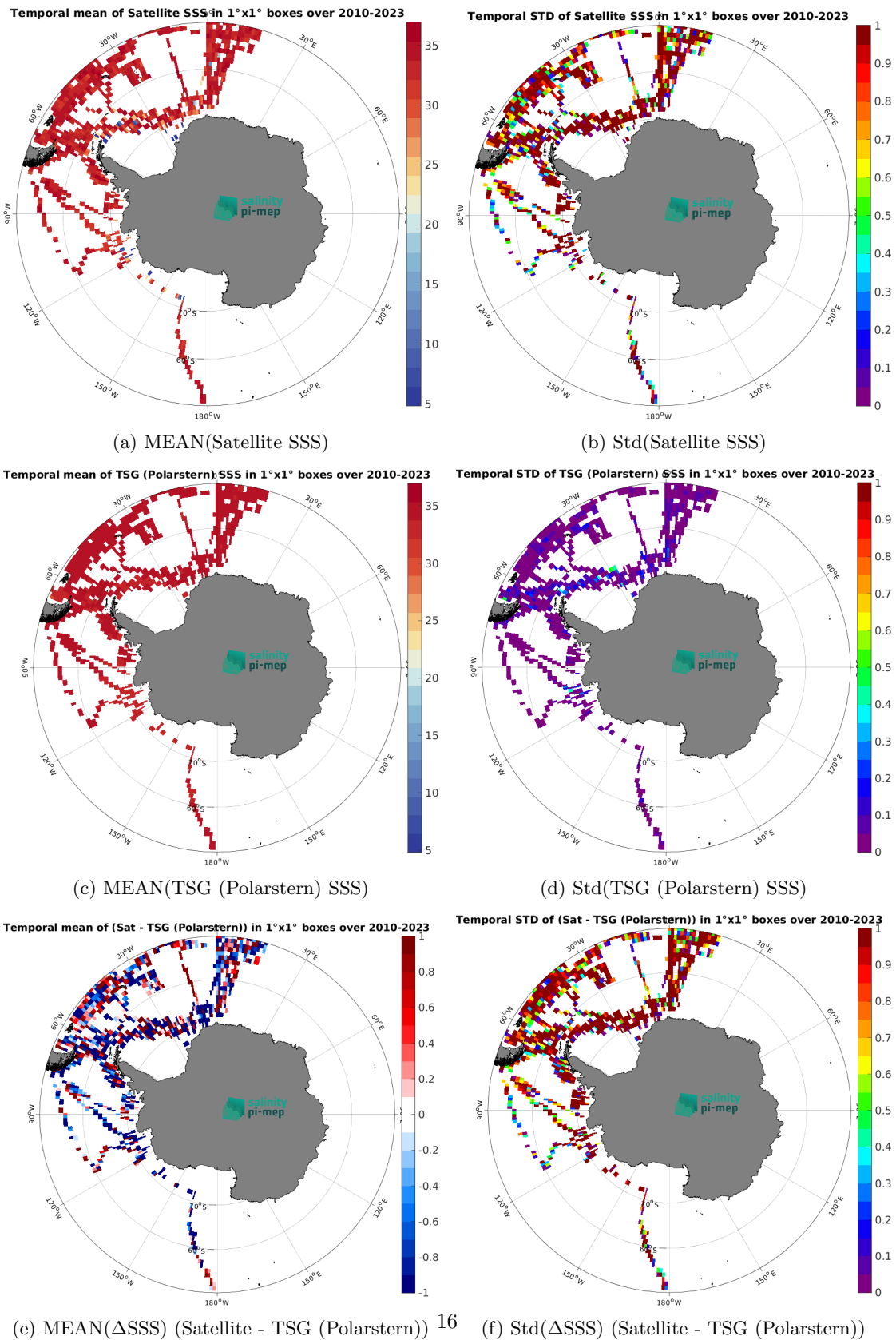
Figure 7: Temporal mean (left) and Std (right) of SSS from SMOS SSS L2Q v331 - With FLAG (CMEMS-CATDS-CPDC) (top), TSG (Polarstern) (middle), and of \Delta SSS (Satellite - TSG (Polarstern)). Only match-up pairs are used to generate these maps.
