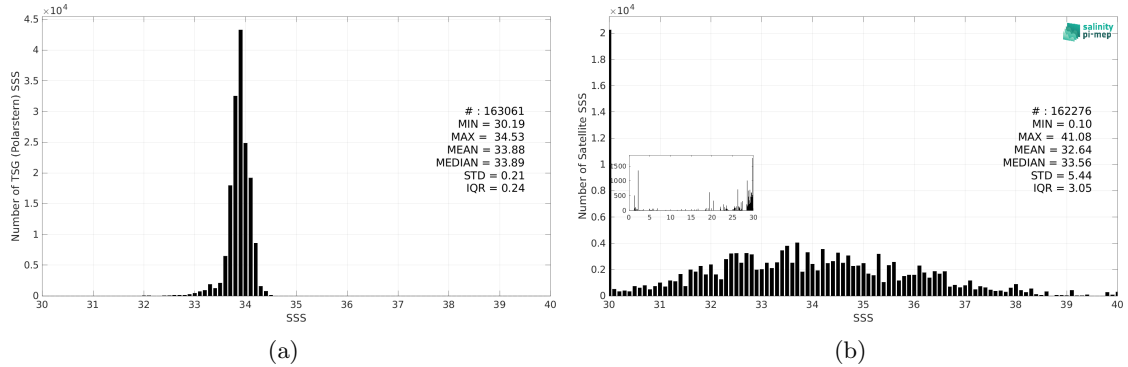
Figure 3: Histograms of SSS from TSG (Polarstern) (a) and SMOS SSS L2Q v331 - With FLAG (CMEMS-CATDS-CPDC) (b) considering all match-up pairs per bins of 0.1 over the Southern Ocean Pi-MEP region and for the full satellite product period.
