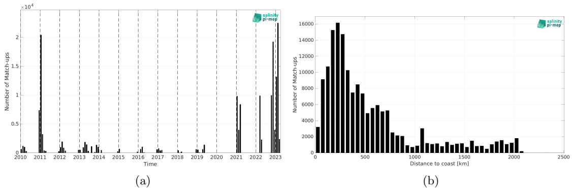
Figure 2: Number of match-ups between TSG (Polarstern) and SMOS SSS L2Q v331 - With FLAG (CMEMS-CATDS-CPDC) SSS as a function of time (a) and as function of the distance to coast (b) over the Southern Ocean Pi-MEP region and for the full satellite product period.
