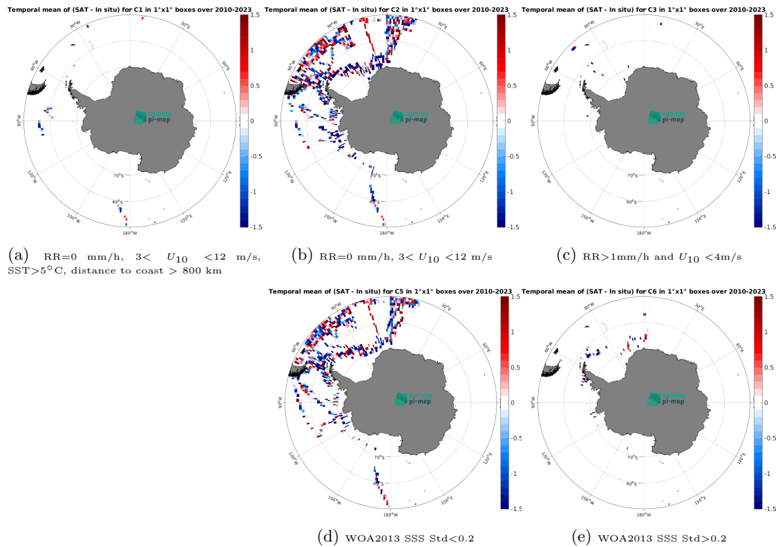
Figure 14: Temporal mean gridded over spatial boxes of size 1^\circ \times 1^\circ of \Delta\text{SSS} (SMOS SSS L2Q v331 - With FLAG (CMEMS-CATDS-CPDC) - TSG (Polarstern)) for 5 different subdatasets corresponding to:RR=0 mm/h, 3 < U_{10} < 12 m/s, SST>5°C, distance to coast > 800 km (a), RR=0 mm/h, 3 < U_{10} < 12 m/s (b), RR>1mm/h and U_{10} < 4 m/s (c), WOA2013 SSS Std<0.2 (d), WOA2013 SSS Std>0.2 (e).
