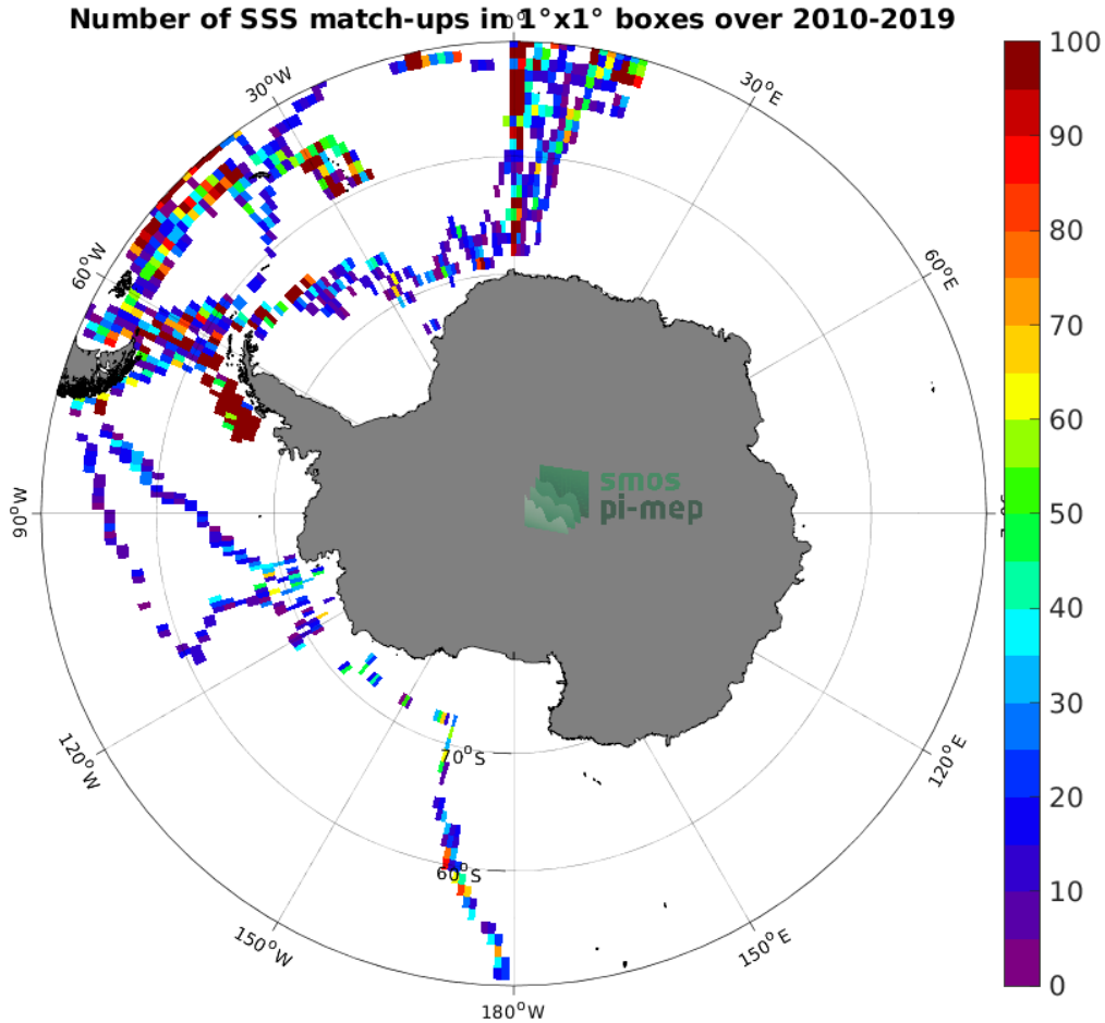
Figure 4: Number of SSS match-ups between TSG (Polarstern) SSS and the SMOS SSS L2Q v331 - With FLAG (CMEMS-CATDS-CPDC) SSS product for the Southern Ocean Pi-MEP region over 1^\circ \times 1^\circ boxes and for the full satellite product period.
