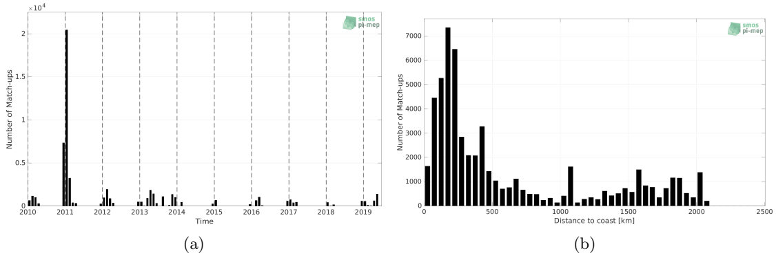
Figure 1: Number of match-ups between TSG (Polarstern) and SMOS SSS L2Q v331 - With FLAG (CMEMS-CATDS-CPDC) SSS as a function of time (a) and as function of the distance to coast (b) over the Southern Ocean Pi-MEP region and for the full satellite product period.
