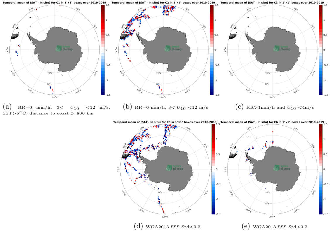
Figure 12: Temporal mean gridded over spatial boxes of size 1^{\circ}\times 1^{\circ} of \Delta\text{SSS} (SMOS SSS L2Q v331 - With FLAG (CMEMS-CATDS-CPDC) - TSG (Polarstern)) for 5 different subdatasets corresponding to:RR=0 mm/h, 3 < U_{10} < 12 m/s, SST >5^{\circ}\text{C} , distance to coast > 800 km (a), RR=0 mm/h, 3 < U_{10} < 12 m/s (b), RR >1 mm/h and U_{10} < 4 m/s (c), WOA2013 SSS Std <0.2 (d), WOA2013 SSS Std >0.2 (e).
