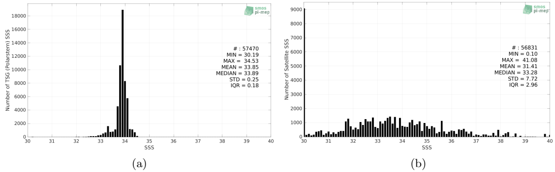
Figure 2: Histograms of SSS from TSG (Polarstern) (a) and SMOS SSS L2Q v331 - With FLAG (CMEMS-CATDS-CPDC) (b) considering all match-up pairs per bins of 0.1 over the Southern Ocean Pi-MEP region and for the full satellite product period.
