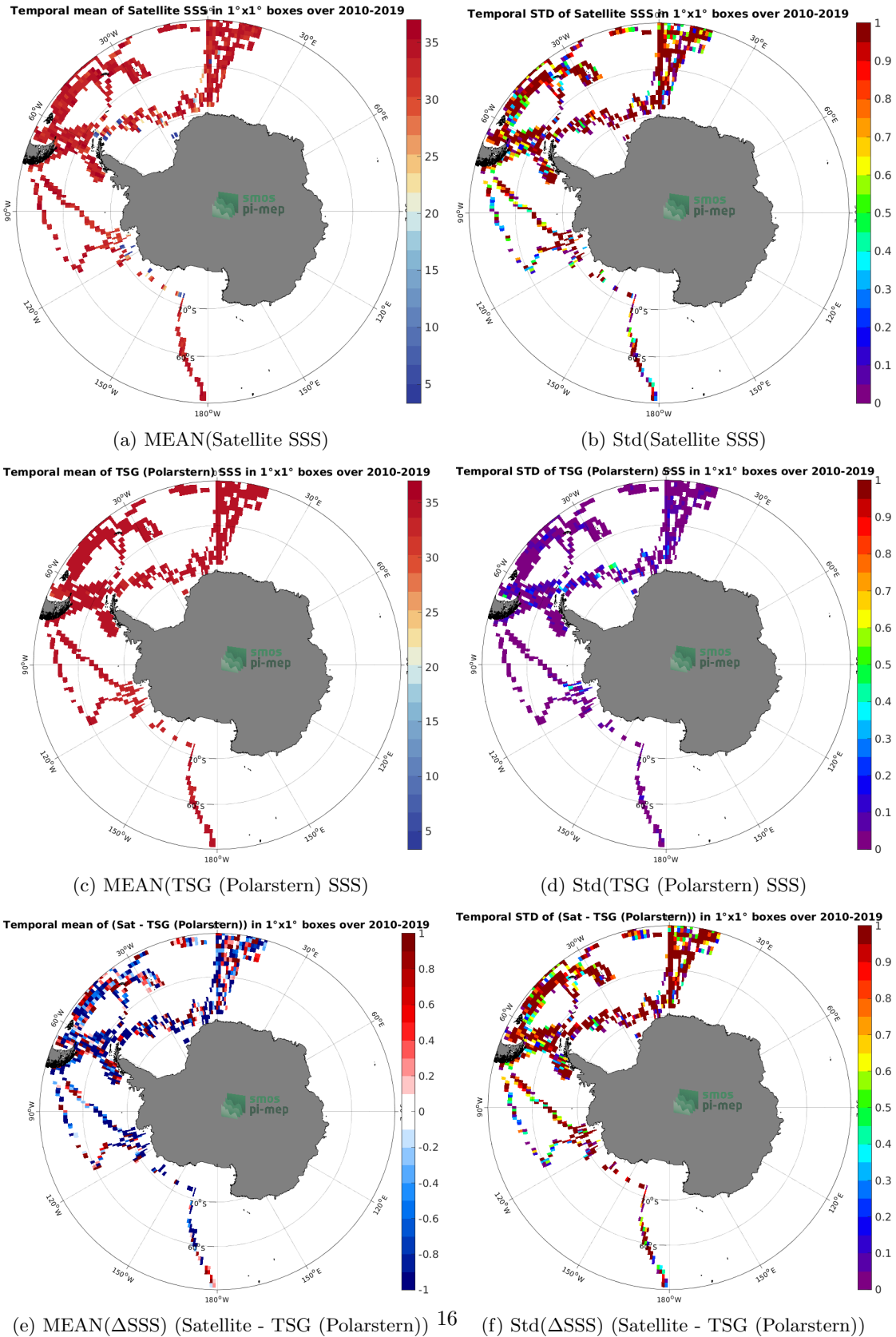
Figure 6: Temporal mean (left) and Std (right) of SSS from SMOS SSS L2Q v331 - With FLAG (CMEMS-CATDS-CPDC) (top), TSG (Polarstern) (middle), and of \Delta SSS (Satellite - TSG (Polarstern)). Only match-up pairs are used to generate these maps.
