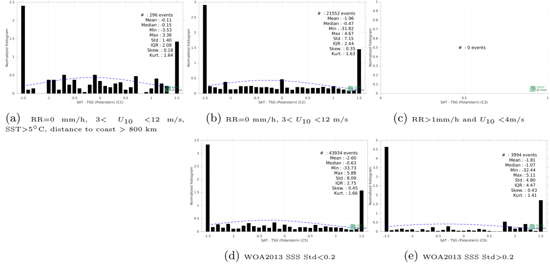
Figure 13: Normalized histogram of \Delta SSS (SMOS SSS L2Q v331 - With FLAG (CMEMS-CATDS-CPDC) - TSG (Polarstern)) for 5 different subdatasets corresponding to: RR=0 mm/h, 3 < U_{10} < 12 m/s, SST > 5°C, distance to coast > 800 km (a), RR=0 mm/h, 3 < U_{10} < 12 m/s (b), RR > 1mm/h and U_{10} < 4 m/s (c), WOA2013 SSS Std < 0.2 (d), WOA2013 SSS Std > 0.2 (e).
