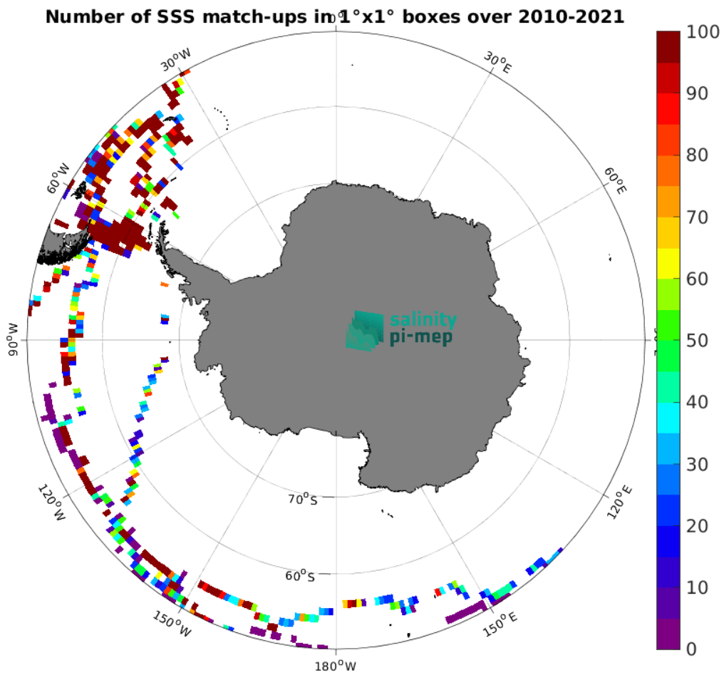
Figure 5: Number of SSS match-ups between TSG (GOSUD-Sailing-ship) SSS and the SMOS SSS L2Q v331 - With FLAG (CMEMS-CATDS-CPDC) SSS product for the Southern Ocean Pi-MEP region over 1^\circ \times 1^\circ boxes and for the full satellite product period.
