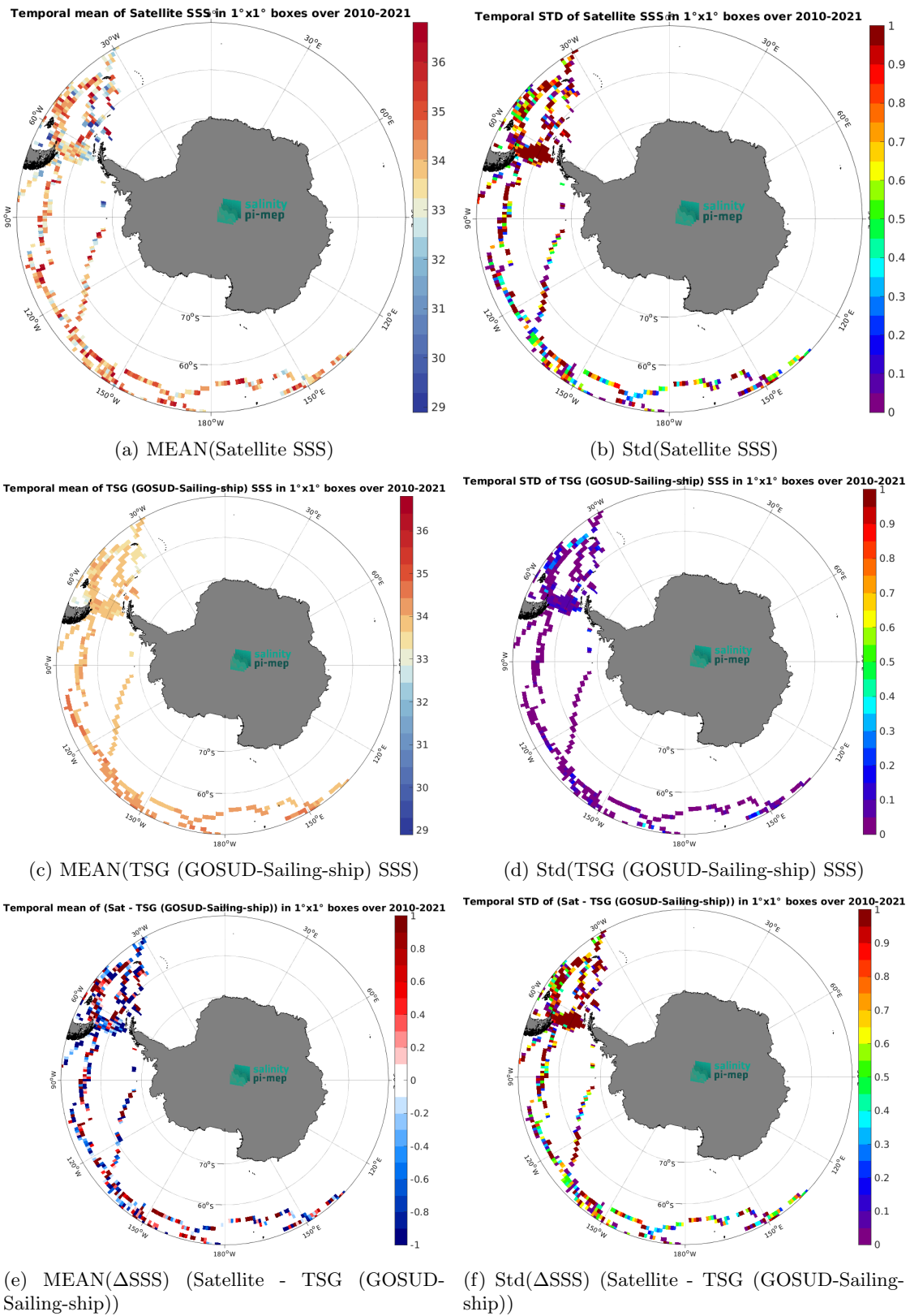
Figure 7: Temporal mean (left) and Std (right) of SSS from SMOS SSS L2Q v331 - With FLAG (CMEMS-CATDS-CPDC) (top), TSG (GOSUD-Sailing-ship) (middle), and of \Delta SSS (Satellite - TSG (GOSUD-Sailing-ship)). Only match-up pairs are used to generate these maps.
