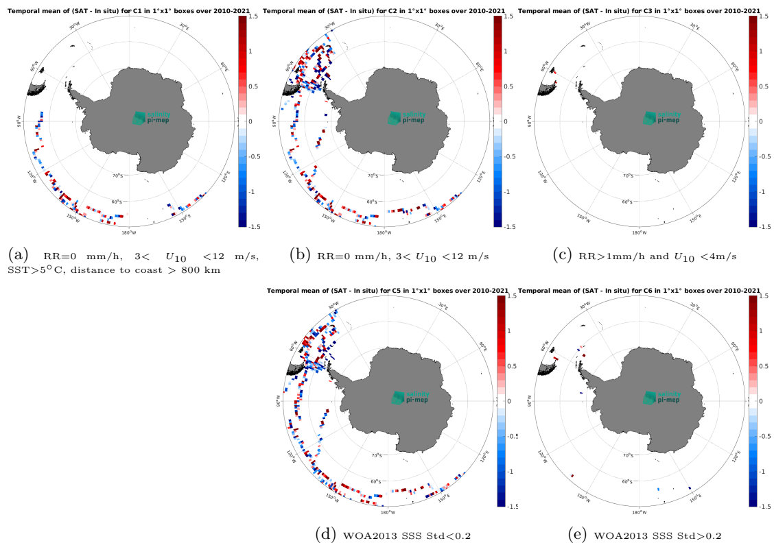
Figure 14: Temporal mean gridded over spatial boxes of size 1^\circ \times 1^\circ of \Delta SSS (SMOS SSS L2Q v331 - With FLAG (CMEMS-CATDS-CPDC) - TSG (GOSUD-Sailing-ship)) for 5 different subdatasets corresponding to:RR=0 mm/h, 3 < U_{10} < 12 m/s, SST > 5^\circ\text{C} , distance to coast > 800 km (a), RR=0 mm/h, 3 < U_{10} < 12 m/s (b), RR > 1 mm/h and U_{10} < 4 m/s (c), WOA2013 SSS Std < 0.2 (d), WOA2013 SSS Std > 0.2 (e).
