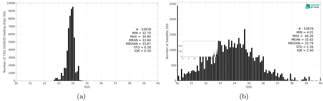
Figure 3: Histograms of SSS from TSG (GOSUD-Sailing-ship) (a) and SMOS SSS L2Q v331 - With FLAG (CMEMS-CATDS-CPDC) (b) considering all match-up pairs per bins of 0.1 over the Southern Ocean Pi-MEP region and for the full satellite product period.
