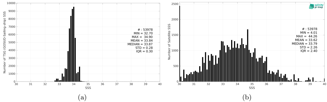
Figure 2: Histograms of SSS from TSG (GOSUD-Sailing-ship) (a) and SMOS SSS L2Q v331 - With FLAG (CMEMS-CATDS-CPDC) (b) considering all match-up pairs per bins of 0.1 over the Southern Ocean Pi-MEP region and for the full satellite product period.
