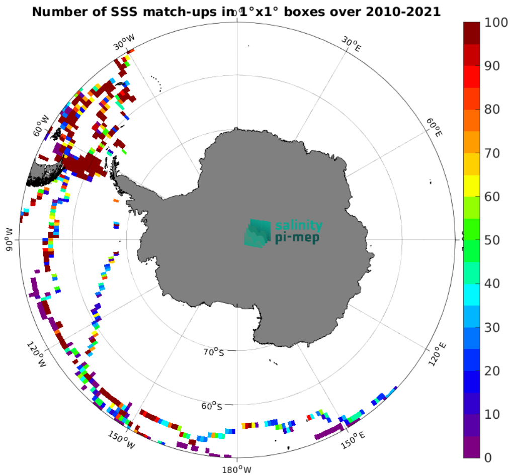
Figure 4: Number of SSS match-ups between TSG (GOSUD-Sailing-ship) SSS and the SMOS SSS L2Q v331 - With FLAG (CMEMS-CATDS-CPDC) SSS product for the Southern Ocean Pi-MEP region over 1^\circ \times 1^\circ boxes and for the full satellite product period.
