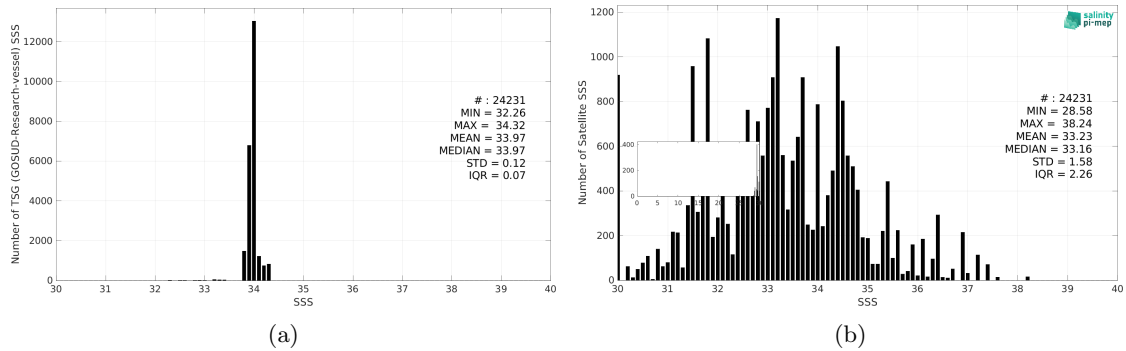
Figure 3: Histograms of SSS from TSG (GOSUD-Research-vessel) (a) and SMOS SSS L2Q v331 - With FLAG (CMEMS-CATDS-CPDC) (b) considering all match-up pairs per bins of 0.1 over the Southern Ocean Pi-MEP region and for the full satellite product period.
