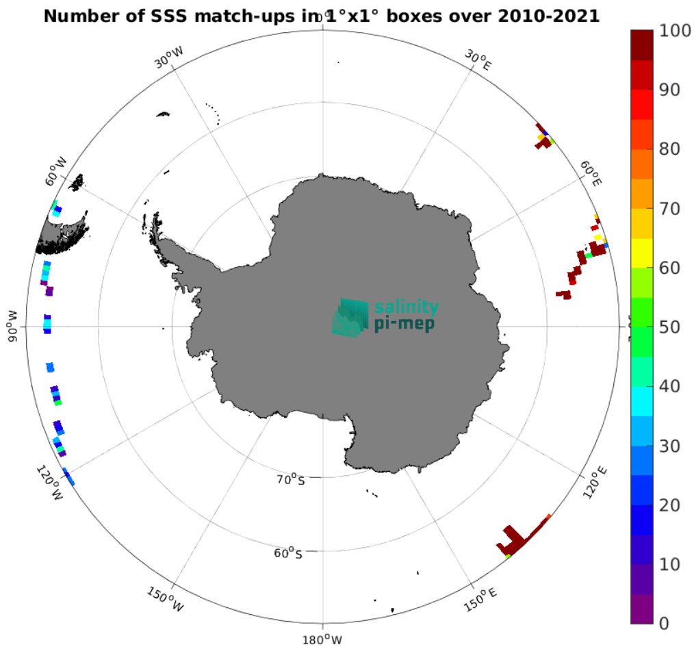
Figure 5: Number of SSS match-ups between TSG (GOSUD-Research-vessel) SSS and the SMOS SSS L2Q v331 - With FLAG (CMEMS-CATDS-CPDC) SSS product for the Southern Ocean Pi-MEP region over 1^\circ \times 1^\circ boxes and for the full satellite product period.
