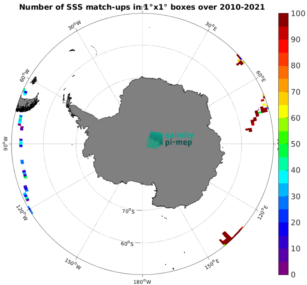
Figure 4: Number of SSS match-ups between TSG (GOSUD-Research-vessel) SSS and the SMOS SSS L2Q v331 - With FLAG (CMEMS-CATDS-CPDC) SSS product for the Southern Ocean Pi-MEP region over 1^{\circ} \times 1^{\circ} boxes and for the full satellite product period.
