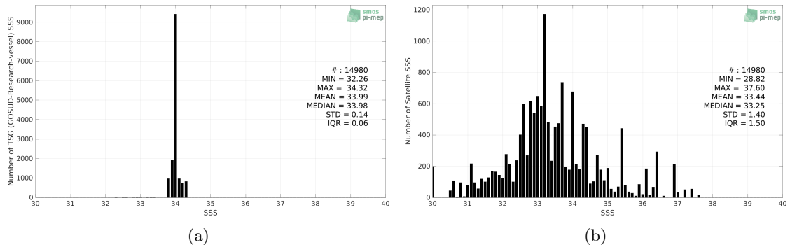
Figure 2: Histograms of SSS from TSG (GOSUD-Research-vessel) (a) and SMOS SSS L2Q v331 - With FLAG (CMEMS-CATDS-CPDC) (b) considering all match-up pairs per bins of 0.1 over the Southern Ocean Pi-MEP region and for the full satellite product period.
