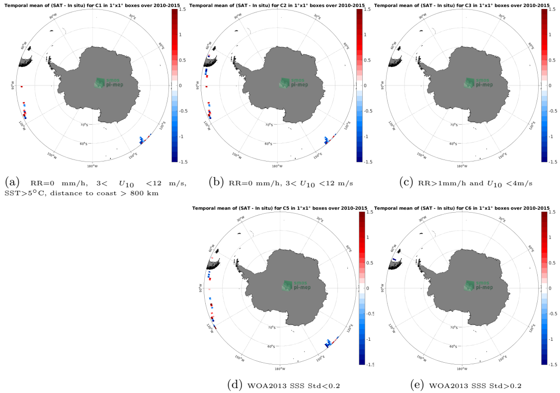
Figure 12: Temporal mean gridded over spatial boxes of size 1^\circ \times 1^\circ of \Delta SSS (SMOS SSS L2Q v331 - With FLAG (CMEMS-CATDS-CPDC) - TSG (GOSUD-Research-vessel)) for 5 different subdatasets corresponding to: RR=0 mm/h, 3 < U_{10} < 12 m/s, SST>5°C, distance to coast > 800 km (a), RR=0 mm/h, 3 < U_{10} < 12 m/s (b), RR>1mm/h and U_{10} < 4 m/s (c), WOA2013 SSS Std<0.2 (d), WOA2013 SSS Std>0.2 (e).
