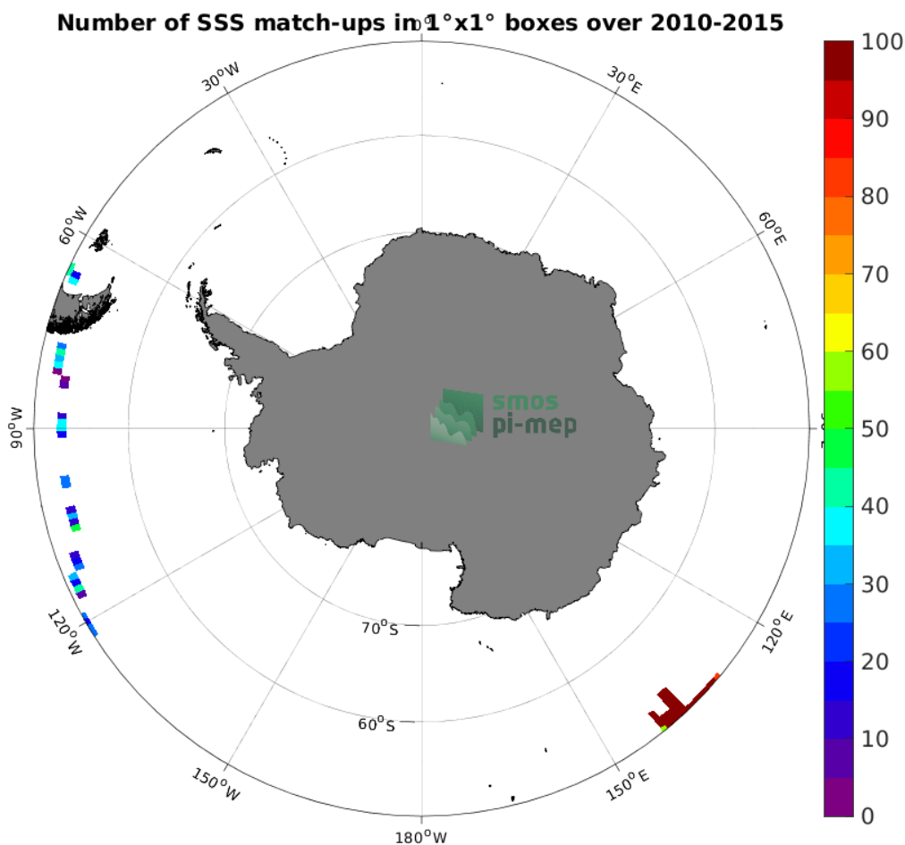
Figure 4: Number of SSS match-ups between TSG (GOSUD-Research-vessel) SSS and the SMOS SSS L2Q v331 - With FLAG (CMEMS-CATDS-CPDC) SSS product for the Southern Ocean Pi-MEP region over 1^\circ \times 1^\circ boxes and for the full satellite product period.
