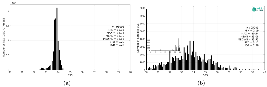
Figure 3: Histograms of SSS from TSG (CSIC-UTM) (a) and SMOS SSS L2Q v331 - With FLAG (CMEMS-CATDS-CPDC) (b) considering all match-up pairs per bins of 0.1 over the Southern Ocean Pi-MEP region and for the full satellite product period.
