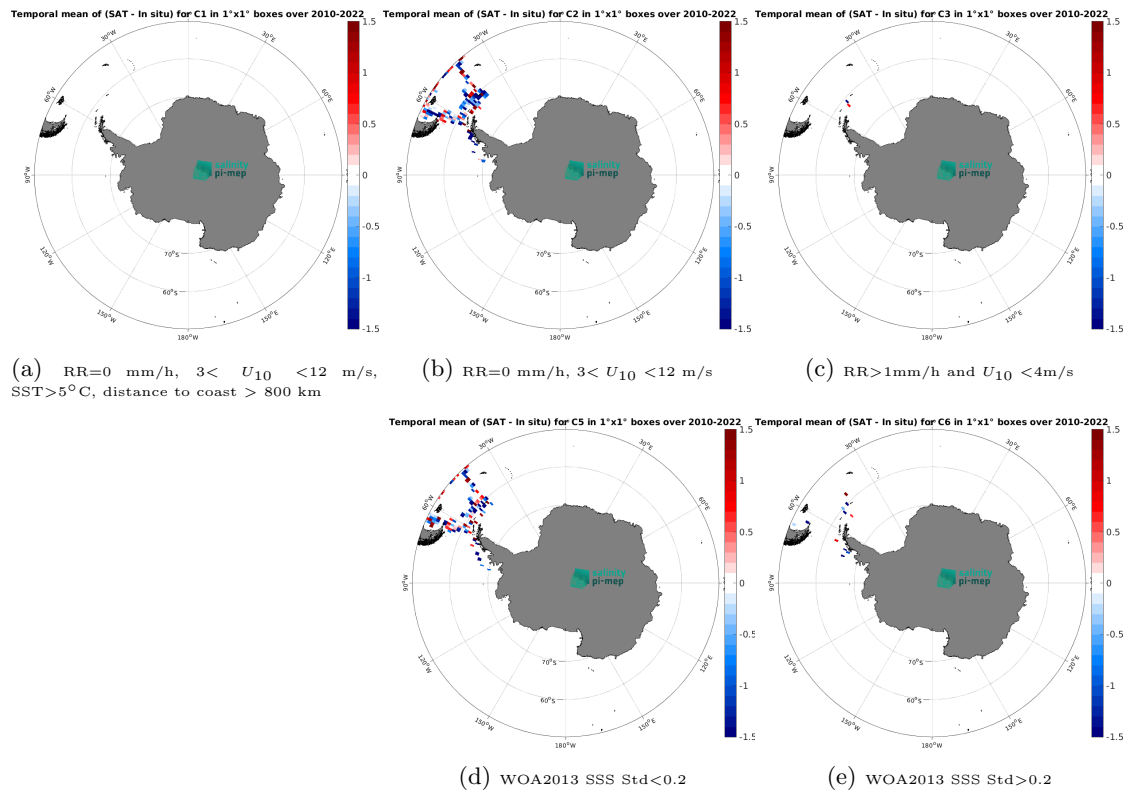
Figure 14: Temporal mean gridded over spatial boxes of size 1^\circ \times 1^\circ of \Delta\text{SSS} (SMOS SSS L2Q v331 - With FLAG (CMEMS-CATDS-CPDC) - TSG (CSIC-UTM)) for 5 different subdatasets corresponding to:RR=0 mm/h, 3 < U_{10} < 12 m/s, SST>5°C, distance to coast > 800 km (a), RR=0 mm/h, 3 < U_{10} < 12 m/s (b), RR>1mm/h and U_{10} < 4 m/s (c), WOA2013 SSS Std<0.2 (d), WOA2013 SSS Std>0.2 (e).
