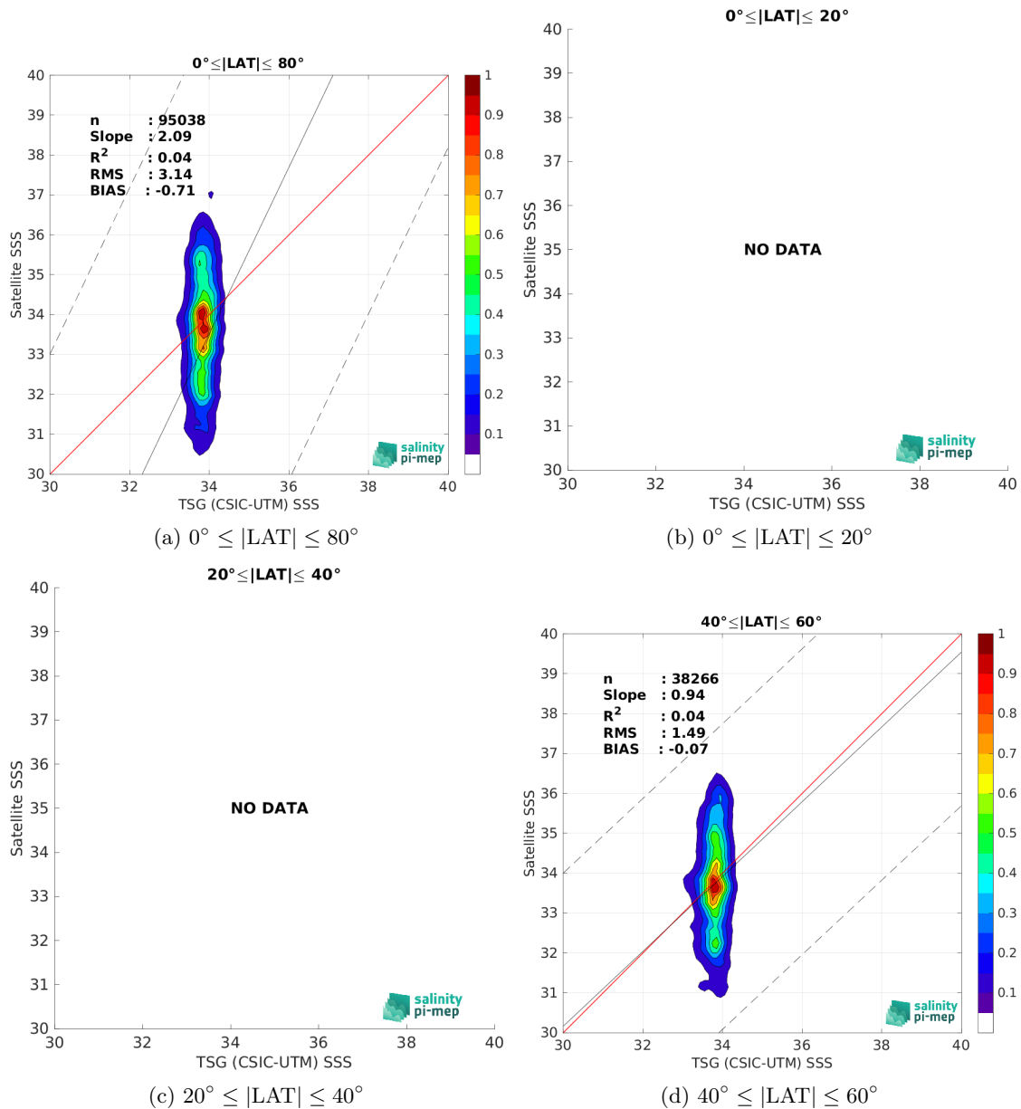
Figure 10: Contour maps of the concentration of SMOS SSS L2Q v331 - With FLAG (CMEMS-CATDS-CPDC) SSS (y-axis) versus TSG (CSIC-UTM) SSS (x-axis) at match-up pairs for different latitude bands. For each plot, the red line shows x=y . The black thin and dashed lines indicate a linear fit through the data cloud and the \pm 95\% confidence levels, respectively. The number match-up pairs n , the slope and R^2 coefficient of the linear fit, the root mean square (RMS) and the mean bias between satellite and in situ data are indicated for each latitude band in each plots.
