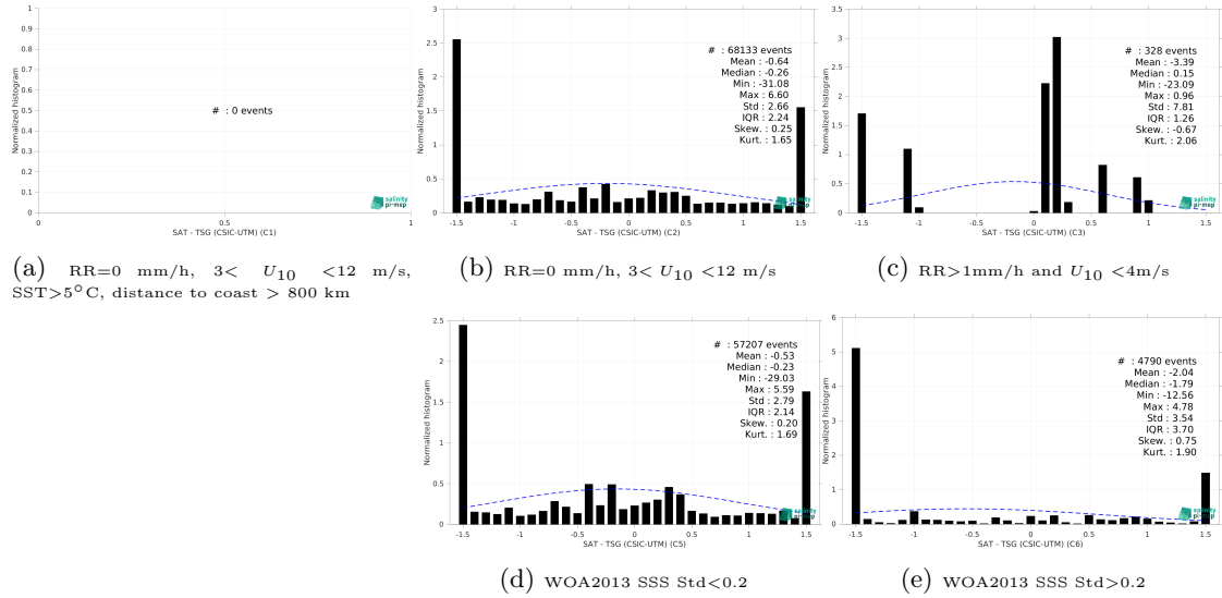
Figure 15: Normalized histogram of \Delta SSS (SMOS SSS L2Q v331 - With FLAG (CMEMS-CATDS-CPDC) - TSG (CSIC-UTM)) for 5 different subdatasets corresponding to: RR=0 mm/h, 3 < U_{10} < 12 m/s, SST > 5°C, distance to coast > 800 km (a), RR=0 mm/h, 3 < U_{10} < 12 m/s (b), RR > 1mm/h and U_{10} < 4 m/s (c), WOA2013 SSS Std < 0.2 (d), WOA2013 SSS Std > 0.2 (e).
