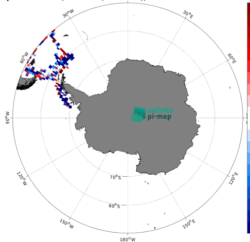
(e) MEAN( \Delta SSS) (Satellite - TSG (CSIC-UTM)) 16
