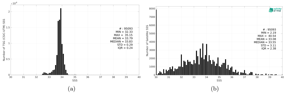
Figure 2: Histograms of SSS from TSG (CSIC-UTM) (a) and SMOS SSS L2Q v331 - With FLAG (CMEMS-CATDS-CPDC) (b) considering all match-up pairs per bins of 0.1 over the Southern Ocean Pi-MEP region and for the full satellite product period.
