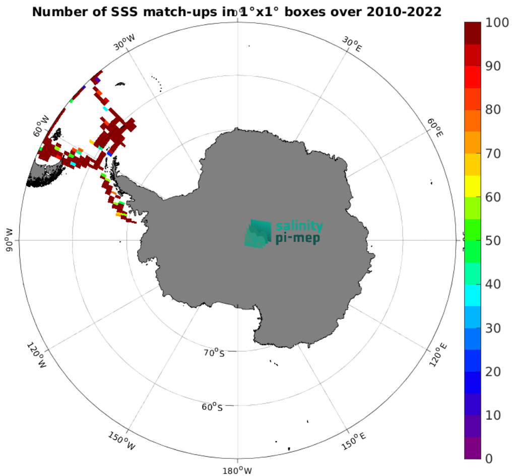
Figure 4: Number of SSS match-ups between TSG (CSIC-UTM) SSS and the SMOS SSS L2Q v331 - With FLAG (CMEMS-CATDS-CPDC) SSS product for the Southern Ocean Pi-MEP region over 1^{\circ} \times 1^{\circ} boxes and for the full satellite product period.
