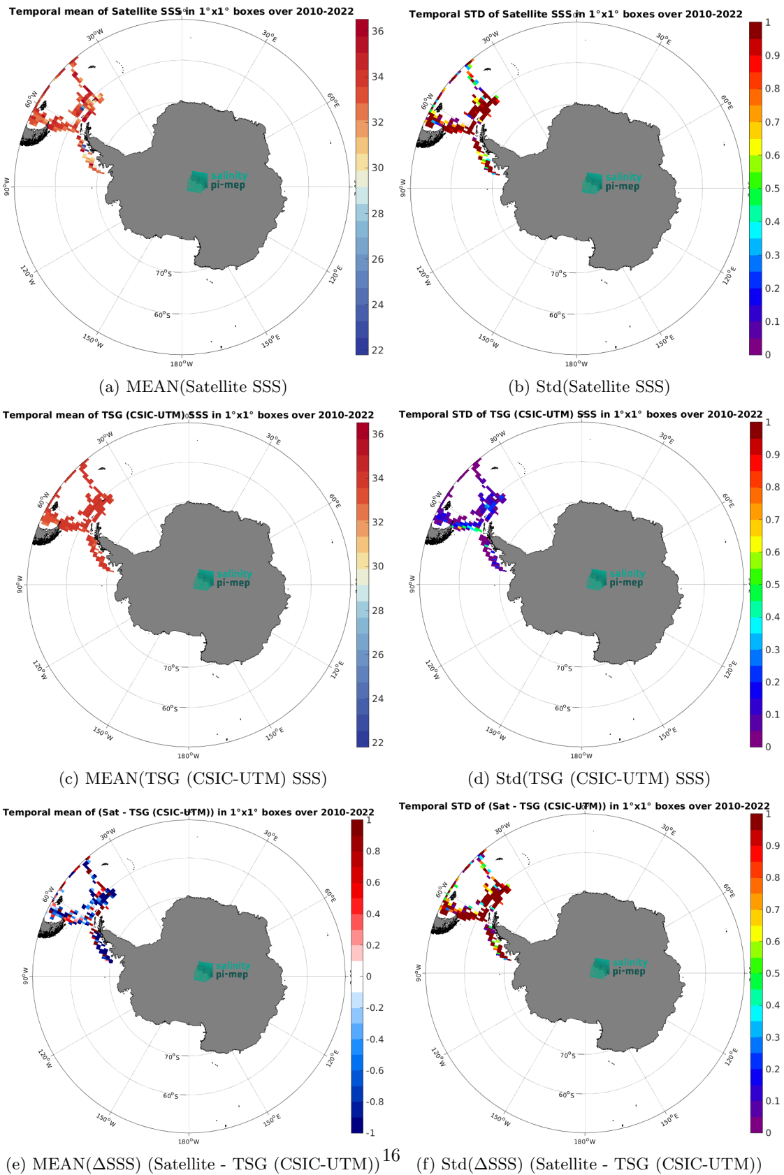
Figure 6: Temporal mean (left) and Std (right) of SSS from SMOS SSS L2Q v331 - With FLAG (CMEMS-CATDS-CPDC) (top), TSG (CSIC-UTM) (middle), and of \Delta SSS (Satellite - TSG (CSIC-UTM)). Only match-up pairs are used to generate these maps.
