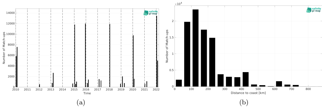
Figure 1: Number of match-ups between TSG (CSIC-UTM) and SMOS SSS L2Q v331 - With FLAG (CMEMS-CATDS-CPDC) SSS as a function of time (a) and as function of the distance to coast (b) over the Southern Ocean Pi-MEP region and for the full satellite product period.
