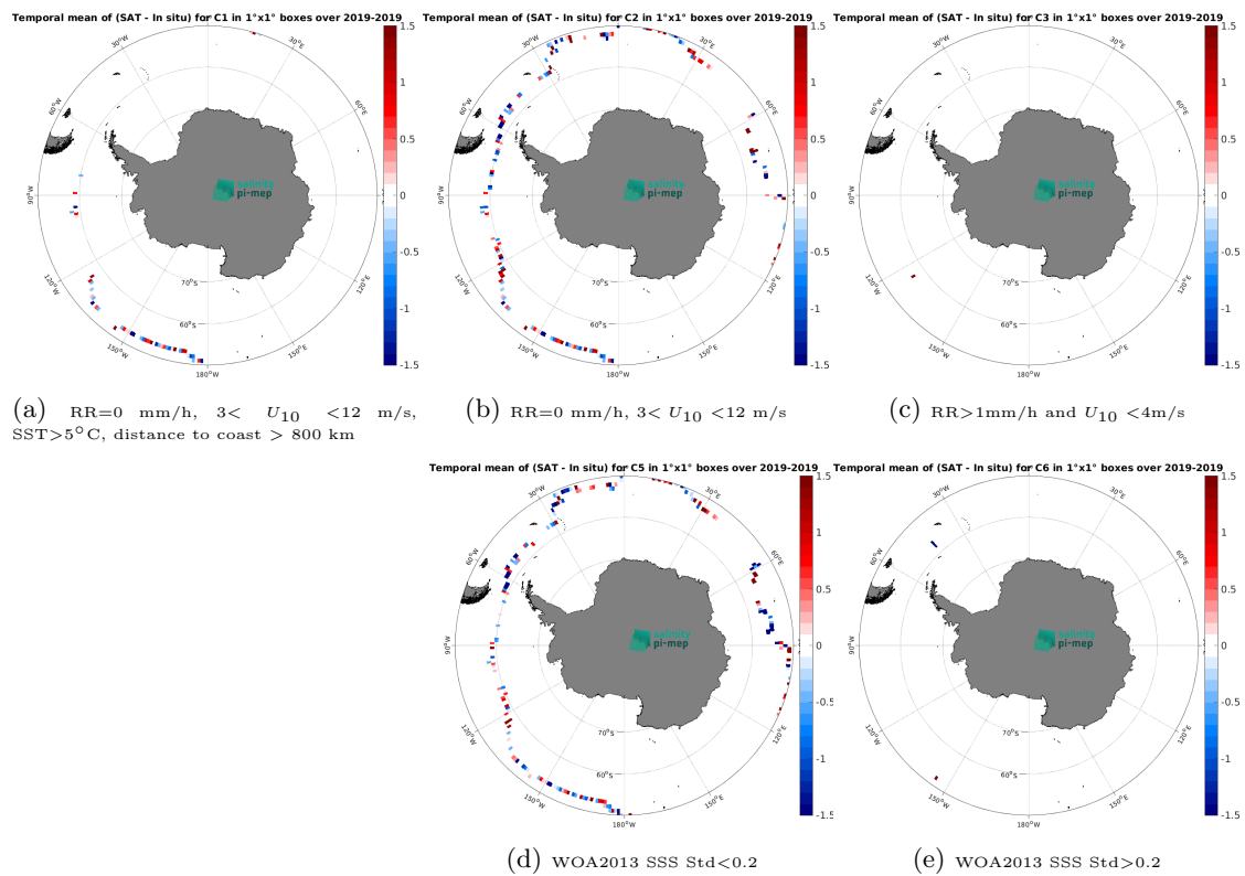
Figure 14: Temporal mean gridded over spatial boxes of size 1^\circ \times 1^\circ of \Delta\text{SSS} (SMOS SSS L2Q v331 - With FLAG (CMEMS-CATDS-CPDC) - Sailerone) for 5 different subdatasets corresponding to:RR=0 mm/h, 3 < U_{10} < 12 m/s, SST>5°C, distance to coast > 800 km (a), RR=0 mm/h, 3 < U_{10} < 12 m/s (b), RR>1mm/h and U_{10} < 4 m/s (c), WOA2013 SSS Std<0.2 (d), WOA2013 SSS Std>0.2 (e).
