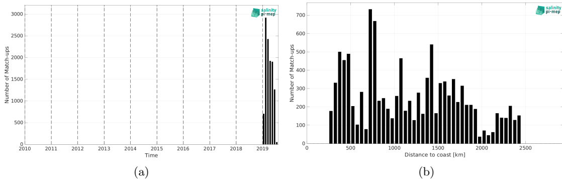
Figure 2: Number of match-ups between Saildrone and SMOS SSS L2Q v331 - With FLAG (CMEMS-CATDS-CPDC) SSS as a function of time (a) and as function of the distance to coast (b) over the Southern Ocean Pi-MEP region and for the full satellite product period.
