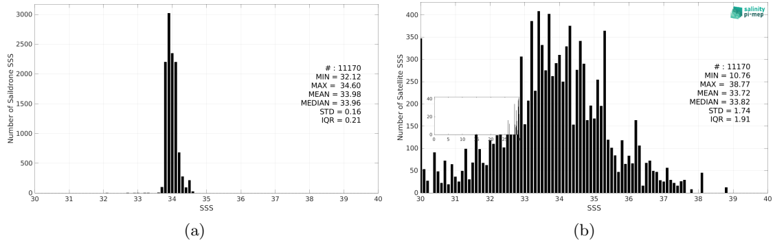
Figure 3: Histograms of SSS from Sairdrone (a) and SMOS SSS L2Q v331 - With FLAG (CMEMS-CATDS-CPDC) (b) considering all match-up pairs per bins of 0.1 over the Southern Ocean Pi-MEP region and for the full satellite product period.
