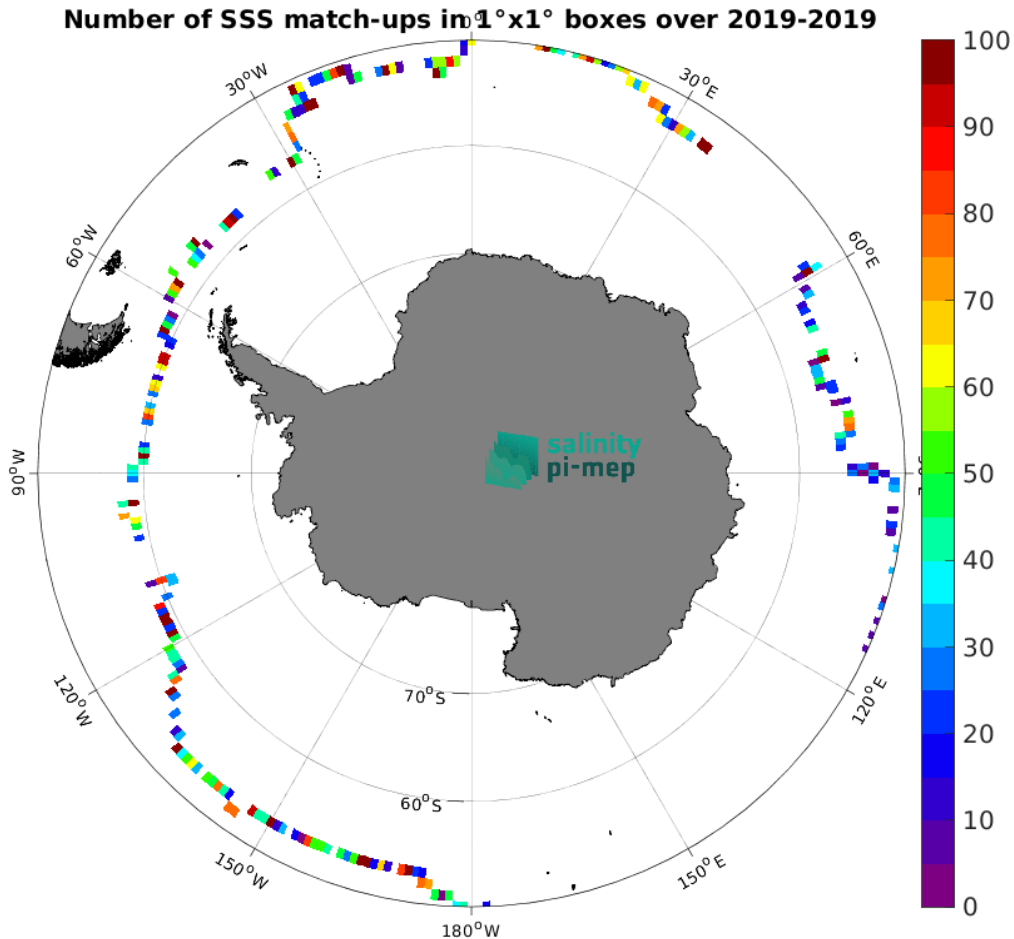
Figure 5: Number of SSS match-ups between Saildrone SSS and the SMOS SSS L2Q v331 - With FLAG (CMEMS-CATDS-CPDC) SSS product for the Southern Ocean Pi-MEP region over 1^\circ \times 1^\circ boxes and for the full satellite product period.
