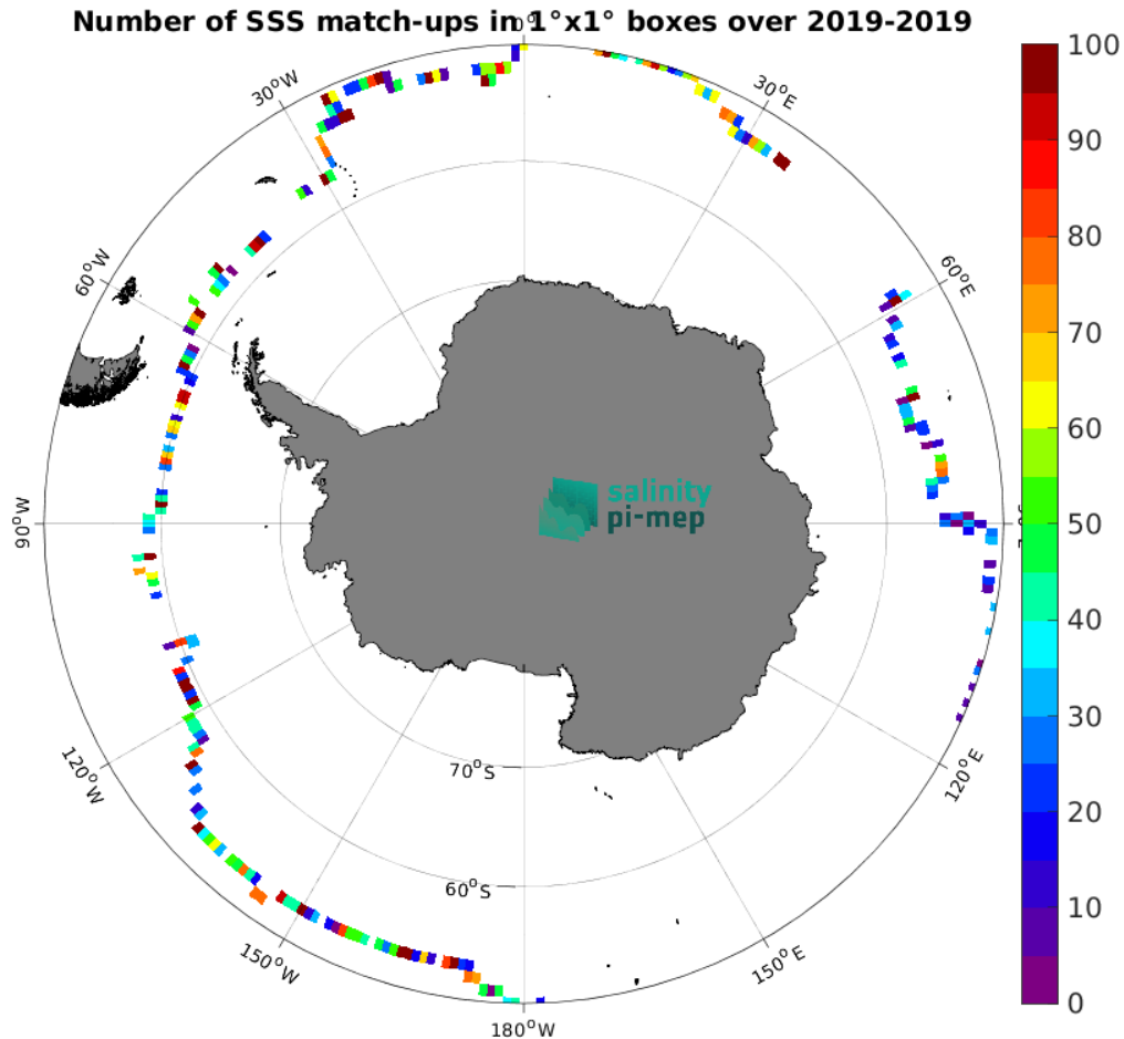
Figure 4: Number of SSS match-ups between Saildrone SSS and the SMOS SSS L2Q v331 - With FLAG (CMEMS-CATDS-CPDC) SSS product for the Southern Ocean Pi-MEP region over 1^\circ \times 1^\circ boxes and for the full satellite product period.
