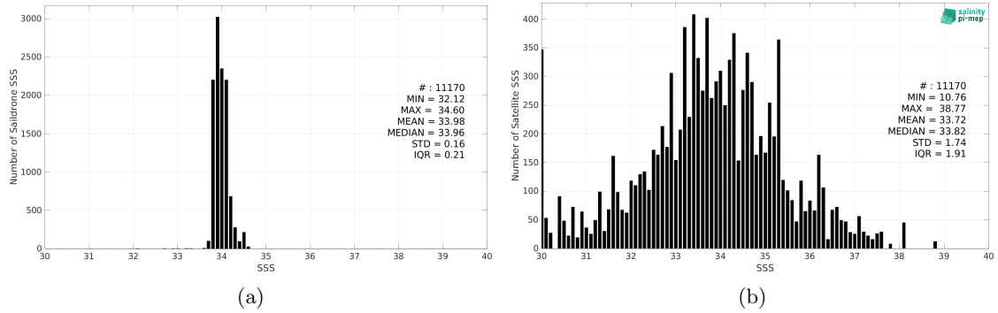
Figure 2: Histograms of SSS from Sairdrone (a) and SMOS SSS L2Q v331 - With FLAG (CMEMS-CATDS-CPDC) (b) considering all match-up pairs per bins of 0.1 over the Southern Ocean Pi-MEP region and for the full satellite product period.
