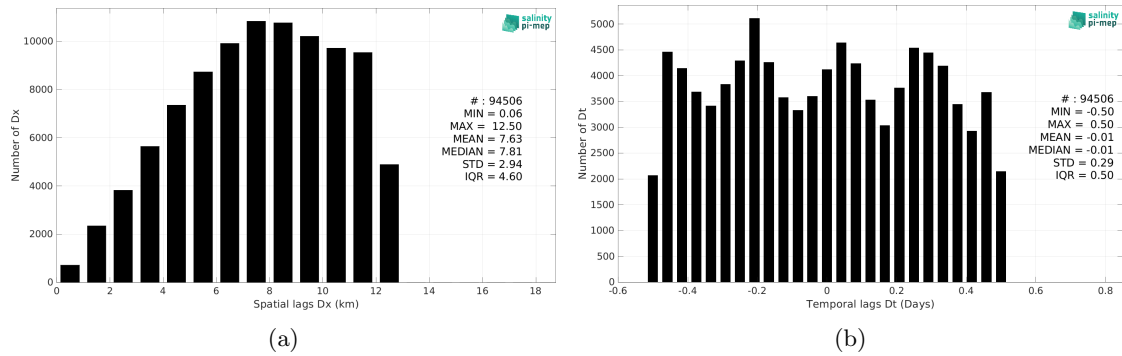
Figure 6: Histograms of the spatial (a) and temporal (b) lags between the location/time of the Marine mammals measurement and the date of the corresponding SMOS SSS L2Q v331 - With FLAG (CMEMS-CATDS-CPDC) SSS pixel.
