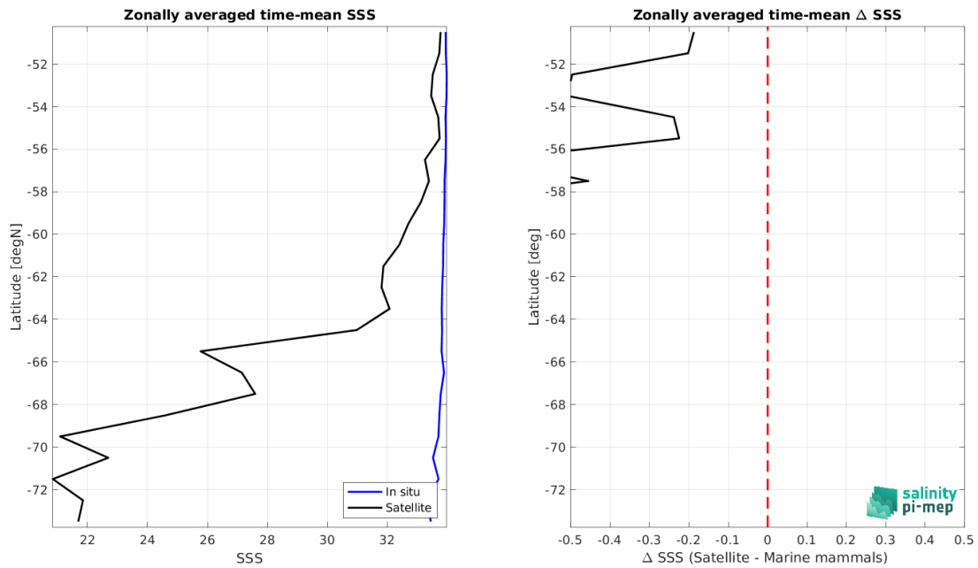
Figure 9: Left panel: Zonal mean SSS from SMOS SSS L2Q v331 - With FLAG (CMEMS-CATDS-CPDC) satellite product (black) and from Marine mammals (blue). Right panel: Zonal mean of \Delta SSS (Satellite - Marine mammals) for all the collected Pi-MEP match-up pairs estimated over the full satellite product period.
