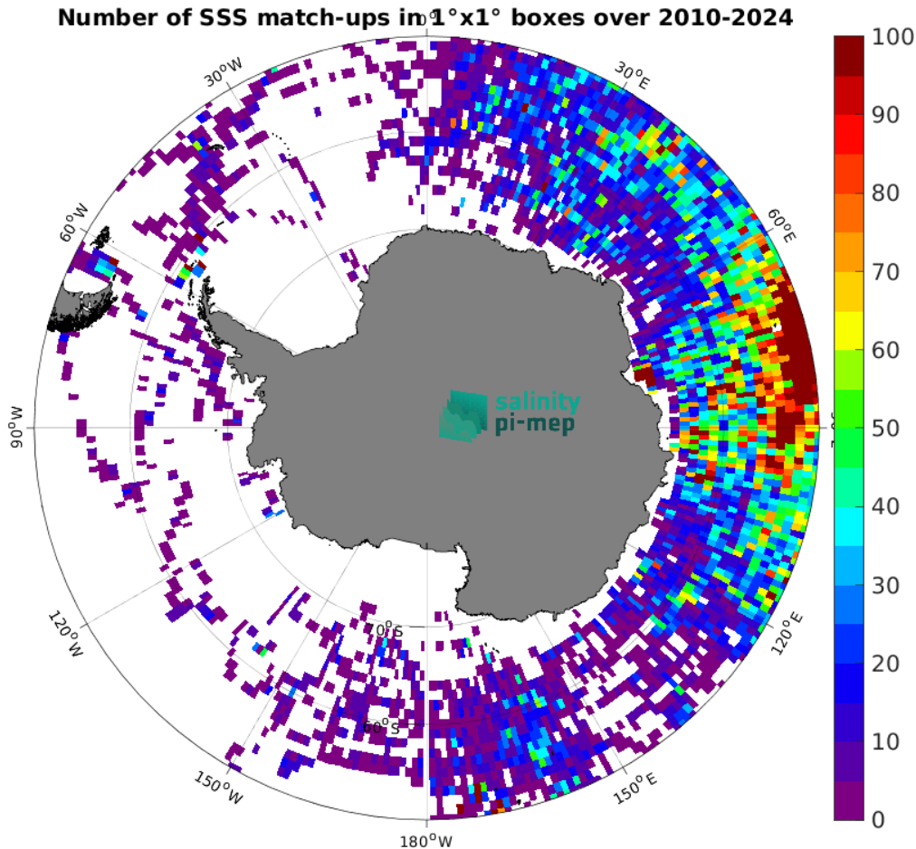
Figure 5: Number of SSS match-ups between Marine mammals SSS and the SMOS SSS L2Q v331 - With FLAG (CMEMS-CATDS-CPDC) SSS product for the Southern Ocean Pi-MEP region over 1^\circ \times 1^\circ boxes and for the full satellite product period.
