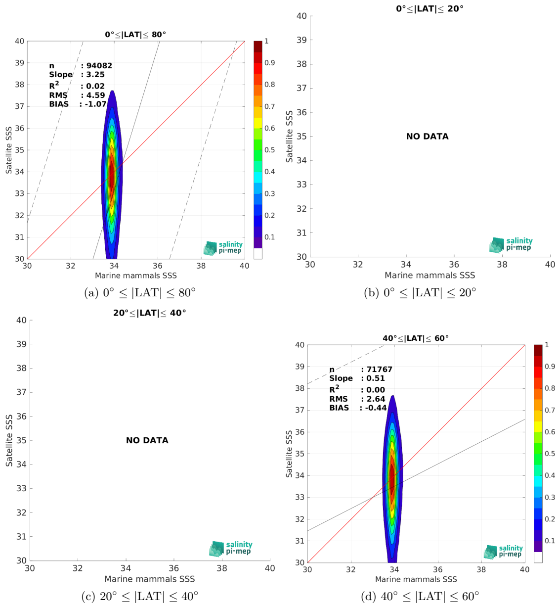
Figure 10: Contour maps of the concentration of SMOS SSS L2Q v331 - With FLAG (CMEMS-CATDS-CPDC) SSS (y-axis) versus Marine mammals SSS (x-axis) at match-up pairs for different latitude bands. For each plot, the red line shows x=y . The black thin and dashed lines indicate a linear fit through the data cloud and the \pm 95\% confidence levels, respectively. The number match-up pairs n , the slope and R^2 coefficient of the linear fit, the root mean square (RMS) and the mean bias between satellite and in situ data are indicated for each latitude band in each plots.
