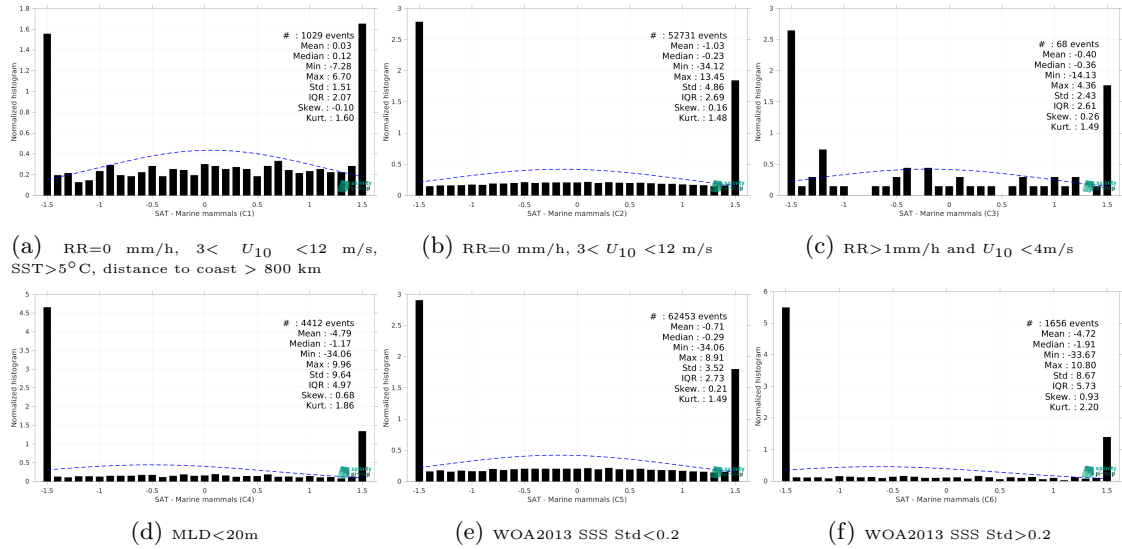
Figure 15: Normalized histogram of \Delta SSS (SMOS SSS L2Q v331 - With FLAG (CMEMS-CATDS-CPDC) - Marine mammals) for 6 different subdatasets corresponding to: RR=0 mm/h, 3 < U_{10} < 12 m/s, SST>5°C, distance to coast > 800 km (a), RR=0 mm/h, 3 < U_{10} < 12 m/s (b), RR>1mm/h and U_{10} < 4 m/s (c), MLD<20m (d), WOA2013 SSS Std<0.2 (e), WOA2013 SSS Std>0.2 (f).
