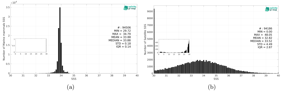
Figure 3: Histograms of SSS from Marine mammals (a) and SMOS SSS L2Q v331 - With FLAG (CMEMS-CATDS-CPDC) (b) considering all match-up pairs per bins of 0.1 over the Southern Ocean Pi-MEP region and for the full satellite product period.
