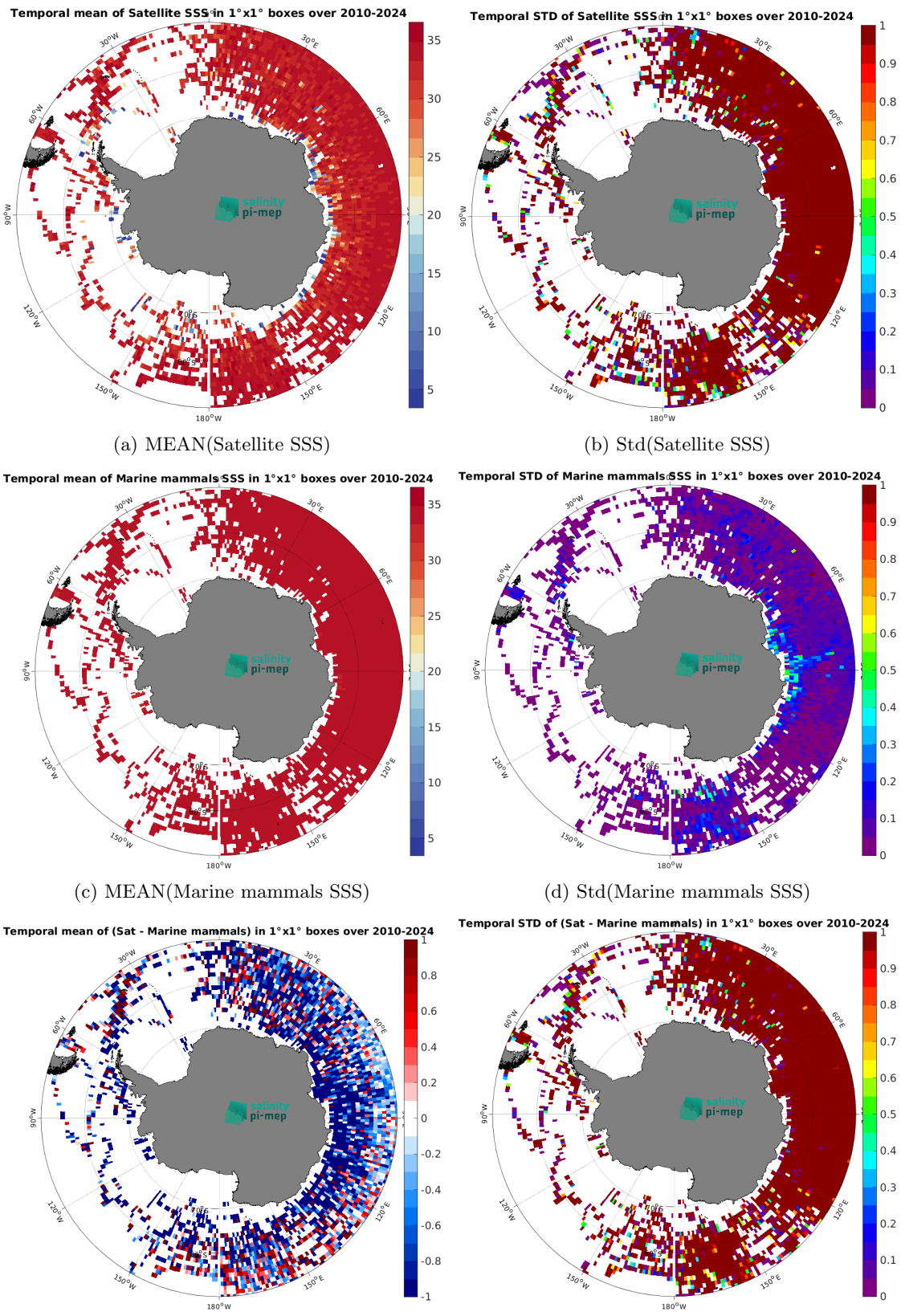
Figure 7: Temporal mean (left) and Std (right) of SSS from SMOS SSS L2Q v331 - With FLAG (CMEMS-CATDS-CPDC) (top), Marine mammals (middle), and of \Delta SSS (Satellite - Marine mammals). Only match-up pairs are used to generate these maps.
