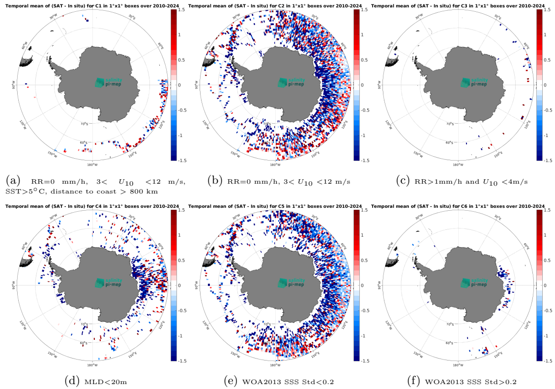
Figure 14: Temporal mean gridded over spatial boxes of size 1^\circ \times 1^\circ of \Delta\text{SSS} (SMOS SSS L2Q v331 - With FLAG (CMEMS-CATDS-CPDC) - Marine mammals) for 6 different subdatasets corresponding to:RR=0 mm/h, 3 < U_{10} < 12 m/s, SST>5°C, distance to coast > 800 km (a), RR=0 mm/h, 3 < U_{10} < 12 m/s (b), RR>1mm/h and U_{10} < 4 m/s (c),MLD<20m (d),WOA2013 SSS Std<0.2 (e),WOA2013 SSS Std>0.2 (f).
