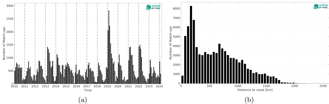
Figure 2: Number of match-ups between Marine mammals and SMOS SSS L2Q v331 - With FLAG (CMEMS-CATDS-CPDC) SSS as a function of time (a) and as function of the distance to coast (b) over the Southern Ocean Pi-MEP region and for the full satellite product period.
