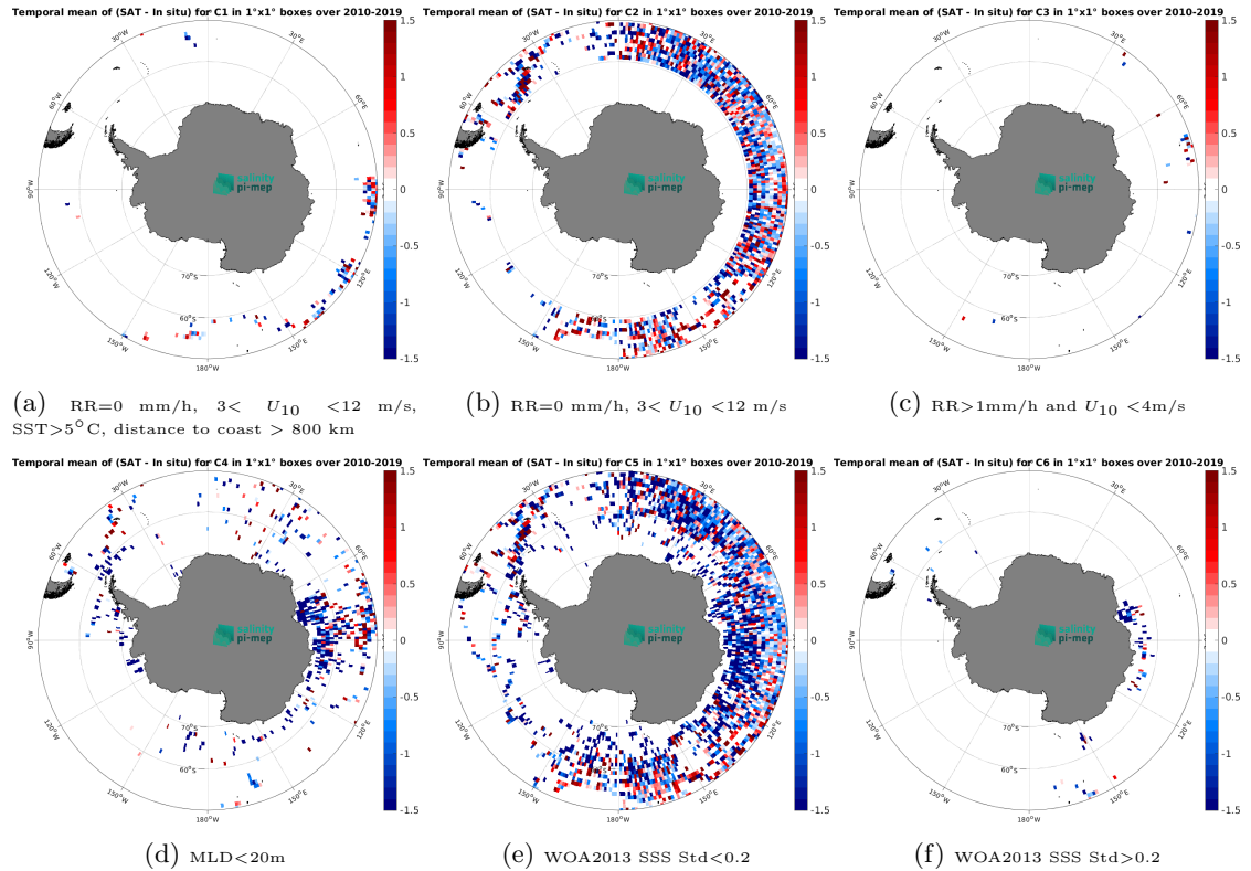
Figure 12: Temporal mean gridded over spatial boxes of size 1^{\circ}\times 1^{\circ} of \Delta\text{SSS} (SMOS SSS L2Q v331 - With FLAG (CMEMS-CATDS-CPDC) - Marine mammals) for 6 different subdatasets corresponding to:RR=0 mm/h, 3 < U_{10} < 12 m/s, SST >5^{\circ}\text{C} , distance to coast > 800 km (a), RR=0 mm/h, 3 < U_{10} < 12 m/s (b), RR >1 mm/h and U_{10} < 4 m/s (c),MLD <20 m (d),WOA2013 SSS Std <0.2 (e),WOA2013 SSS Std >0.2 (f).
