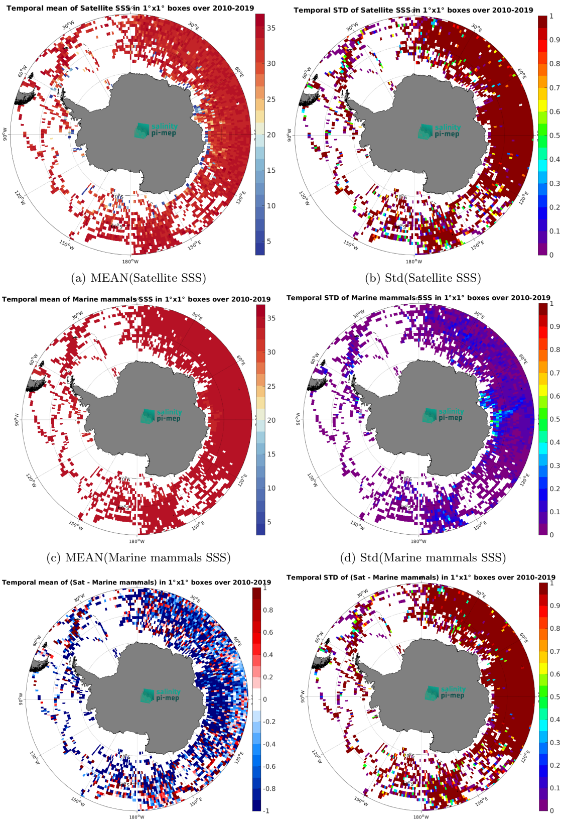
Figure 6: Temporal mean (left) and Std (right) of SSS from SMOS SSS L2Q v331 - With FLAG (CMEMS-CATDS-CPDC) (top), Marine mammals (middle), and of \Delta SSS (Satellite - Marine mammals). Only match-up pairs are used to generate these maps.
