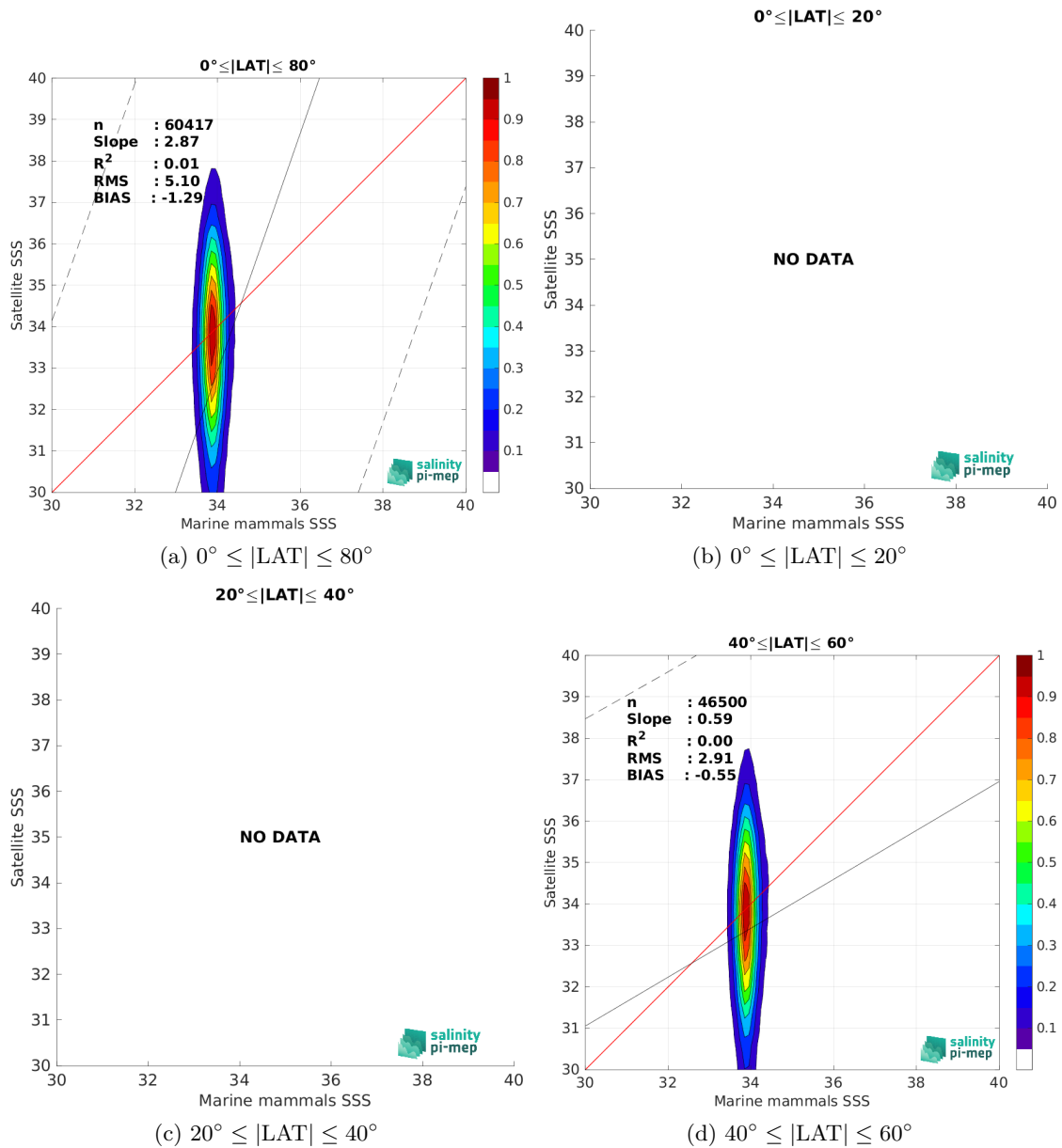
Figure 9: Contour maps of the concentration of SMOS SSS L2Q v331 - With FLAG (CMEMS-CATDS-CPDC) SSS (y-axis) versus Marine mammals SSS (x-axis) at match-up pairs for different latitude bands. For each plot, the red line shows x=y . The black thin and dashed lines indicate a linear fit through the data cloud and the \pm 95\% confidence levels, respectively. The number match-up pairs n , the slope and R^2 coefficient of the linear fit, the root mean square (RMS) and the mean bias between satellite and in situ data are indicated for each latitude band in each plots.
