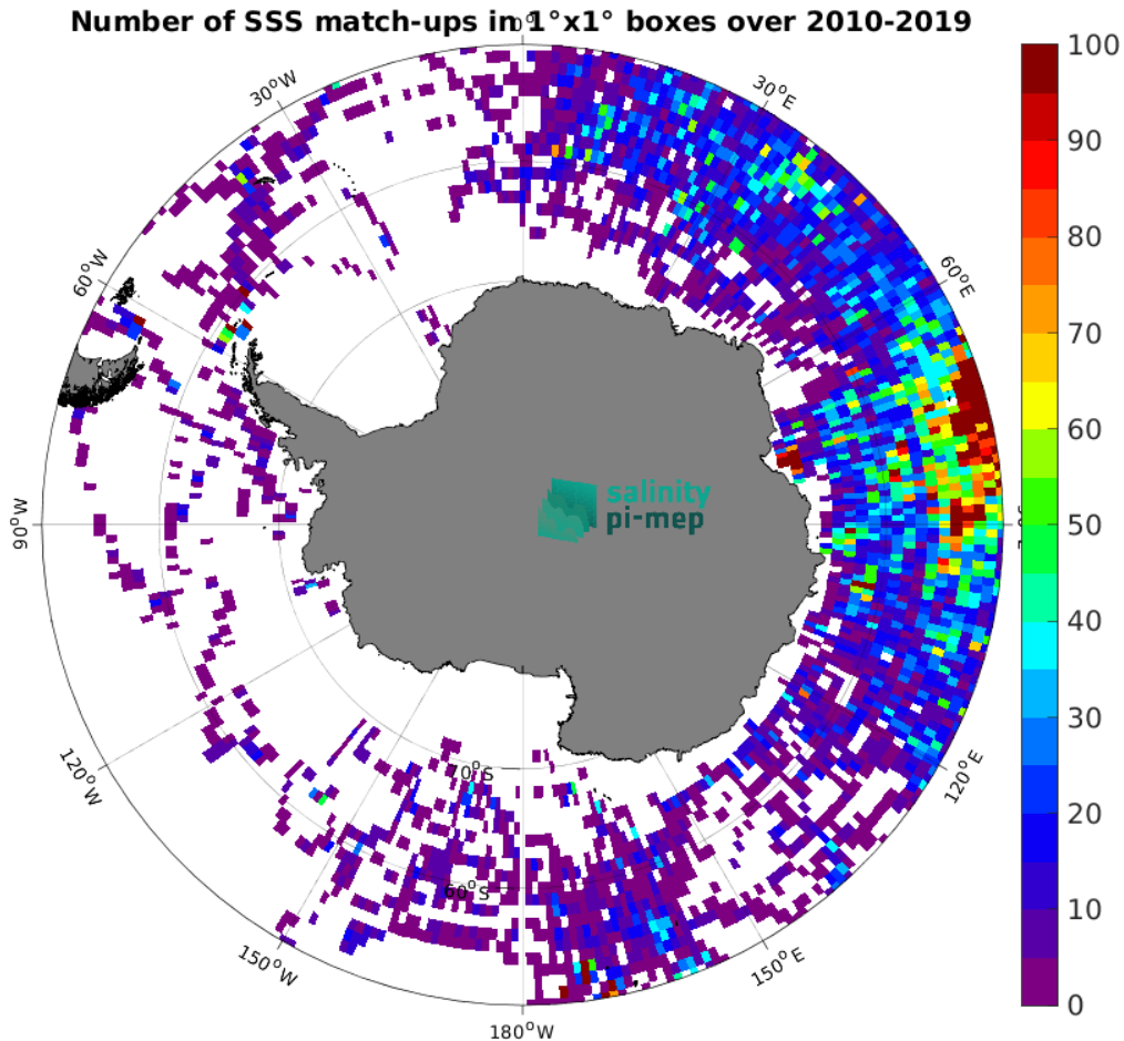
Figure 4: Number of SSS match-ups between Marine mammals SSS and the SMOS SSS L2Q v331 - With FLAG (CMEMS-CATDS-CPDC) SSS product for the Southern Ocean Pi-MEP region over 1^\circ \times 1^\circ boxes and for the full satellite product period.
