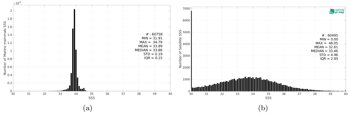
Figure 2: Histograms of SSS from Marine mammals (a) and SMOS SSS L2Q v331 - With FLAG (CMEMS-CATDS-CPDC) (b) considering all match-up pairs per bins of 0.1 over the Southern Ocean Pi-MEP region and for the full satellite product period.
