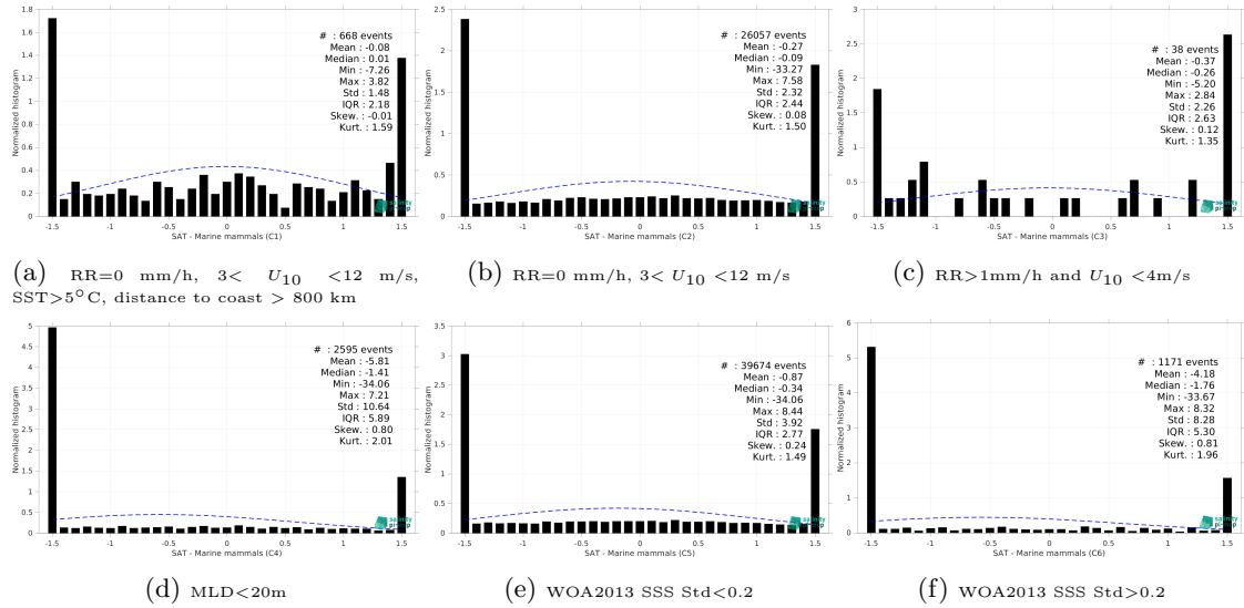
Figure 13: Normalized histogram of \Delta SSS (SMOS SSS L2Q v331 - With FLAG (CMEMS-CATDS-CPDC) - Marine mammals) for 6 different subdatasets corresponding to: RR=0 mm/h, 3 < U_{10} < 12 m/s, SST>5°C, distance to coast > 800 km (a), RR=0 mm/h, 3 < U_{10} < 12 m/s (b), RR>1mm/h and U_{10} < 4 m/s (c), MLD<20m (d), WOA2013 SSS Std<0.2 (e), WOA2013 SSS Std>0.2 (f).
