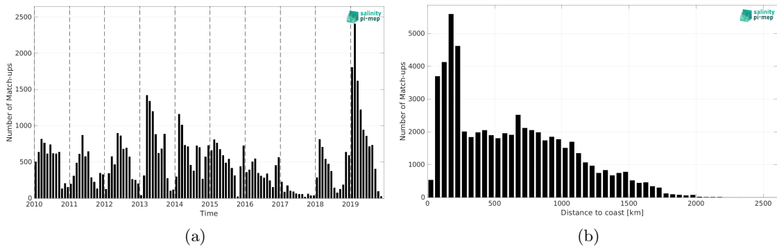
Figure 1: Number of match-ups between Marine mammals and SMOS SSS L2Q v331 - With FLAG (CMEMS-CATDS-CPDC) SSS as a function of time (a) and as function of the distance to coast (b) over the Southern Ocean Pi-MEP region and for the full satellite product period.
