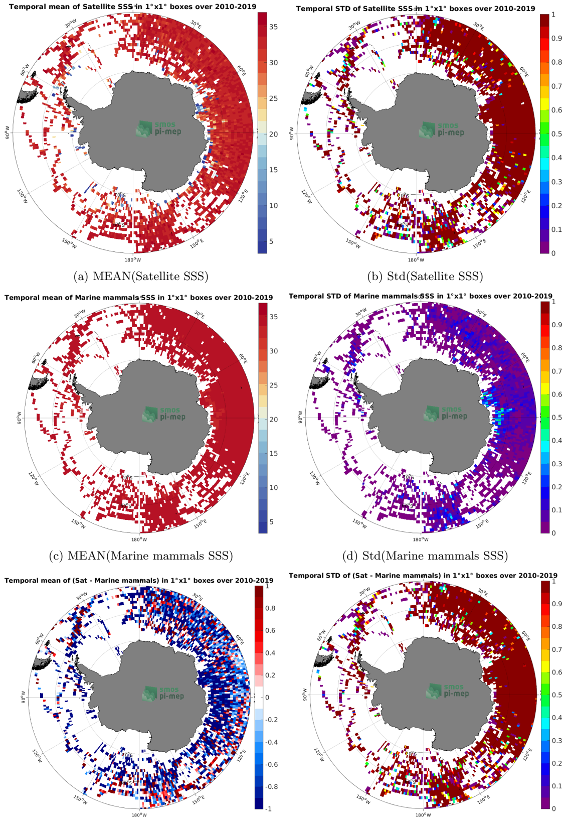
Figure 6: Temporal mean (left) and Std (right) of SSS from SMOS SSS L2Q v331 - With FLAG (CMEMS-CATDS-CPDC) (top), Marine mammals (middle), and of \Delta SSS (Satellite - Marine mammals). Only match-up pairs are used to generate these maps.
