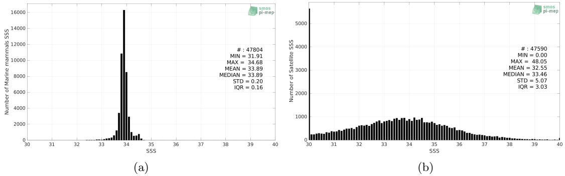
Figure 2: Histograms of SSS from Marine mammals (a) and SMOS SSS L2Q v331 - With FLAG (CMEMS-CATDS-CPDC) (b) considering all match-up pairs per bins of 0.1 over the Southern Ocean Pi-MEP region and for the full satellite product period.
