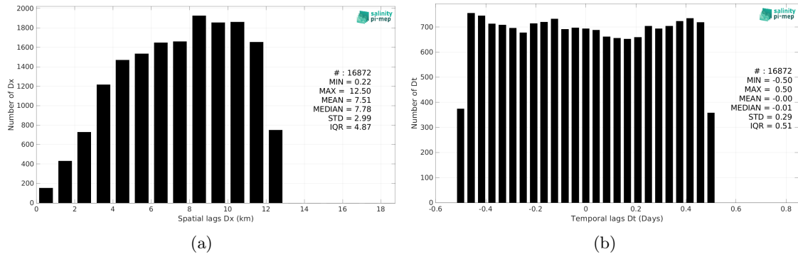
Figure 5: Histograms of the spatial (a) and temporal (b) lags between the location/time of the Surface drifters measurement and the date of the corresponding SMOS SSS L2Q v331 - With FLAG (CMEMS-CATDS-CPDC) SSS pixel.
