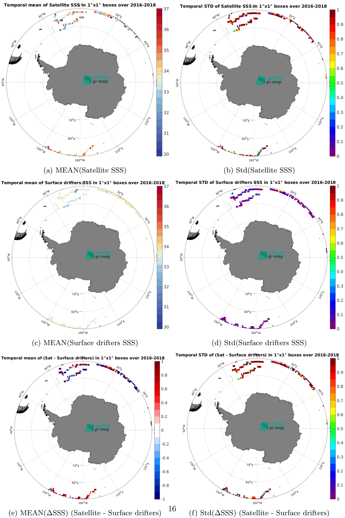
Figure 6: Temporal mean (left) and Std (right) of SSS from SMOS SSS L2Q v331 - With FLAG (CMEMS-CATDS-CPDC) (top), Surface drifters (middle), and of \Delta SSS (Satellite - Surface drifters). Only match-up pairs are used to generate these maps.
