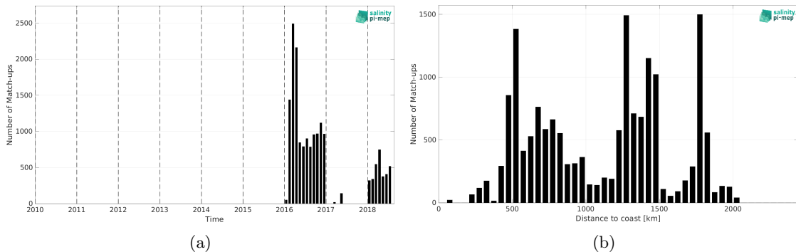
Figure 2: Number of match-ups between Surface drifters and SMOS SSS L2Q v331 - With FLAG (CMEMS-CATDS-CPDC) SSS as a function of time (a) and as function of the distance to coast (b) over the Southern Ocean Pi-MEP region and for the full satellite product period.
