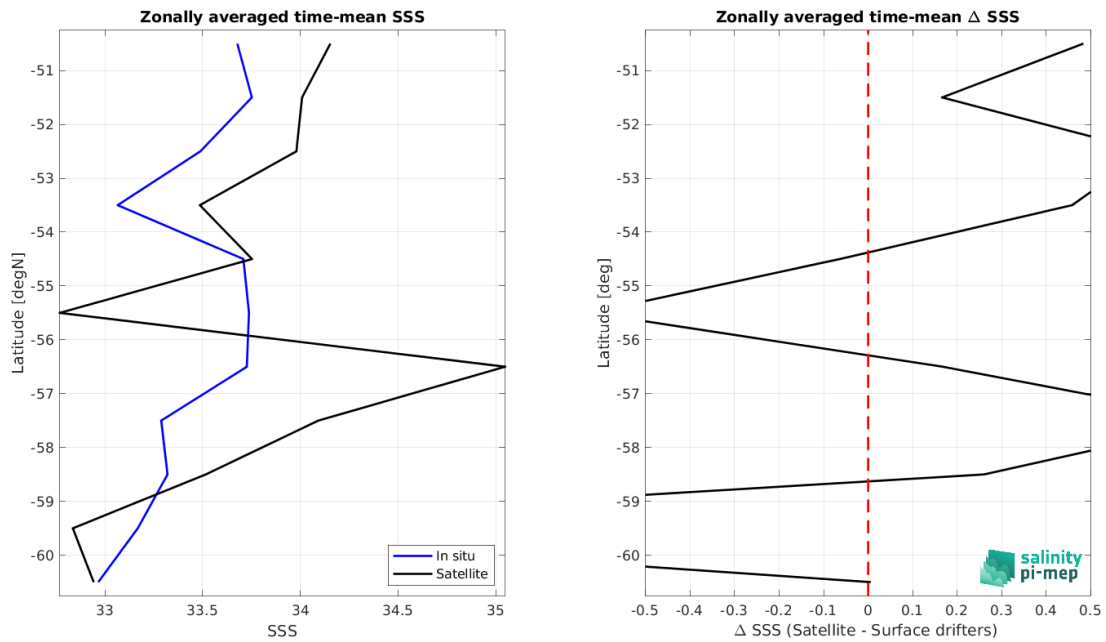
Figure 8: Left panel: Zonal mean SSS from SMOS SSS L2Q v331 - With FLAG (CMEMS-CATDS-CPDC) satellite product (black) and from Surface drifters (blue). Right panel: Zonal mean of \Delta SSS (Satellite - Surface drifters) for all the collected Pi-MEP match-up pairs estimated over the full satellite product period.
