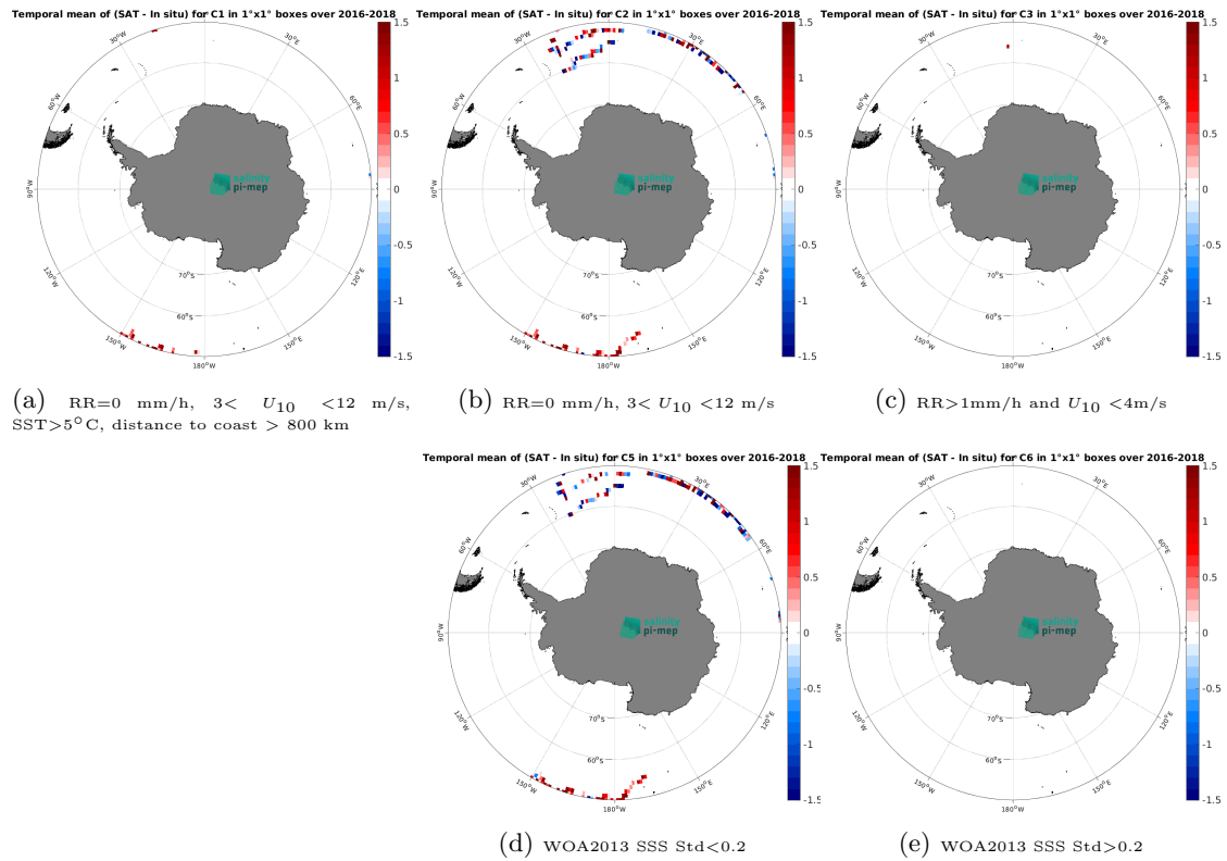
Figure 13: Temporal mean gridded over spatial boxes of size 1^\circ \times 1^\circ of \Delta SSS (SMOS SSS L2Q v331 - With FLAG (CMEMS-CATDS-CPDC) - Surface drifters) for 5 different subdatasets corresponding to:RR=0 mm/h, 3 < U_{10} < 12 m/s, SST >5^\circ\text{C} , distance to coast > 800 km (a), RR=0 mm/h, 3 < U_{10} < 12 m/s (b), RR >1 mm/h and U_{10} < 4 m/s (c), WOA2013 SSS Std <0.2 (d), WOA2013 SSS Std >0.2 (e).
