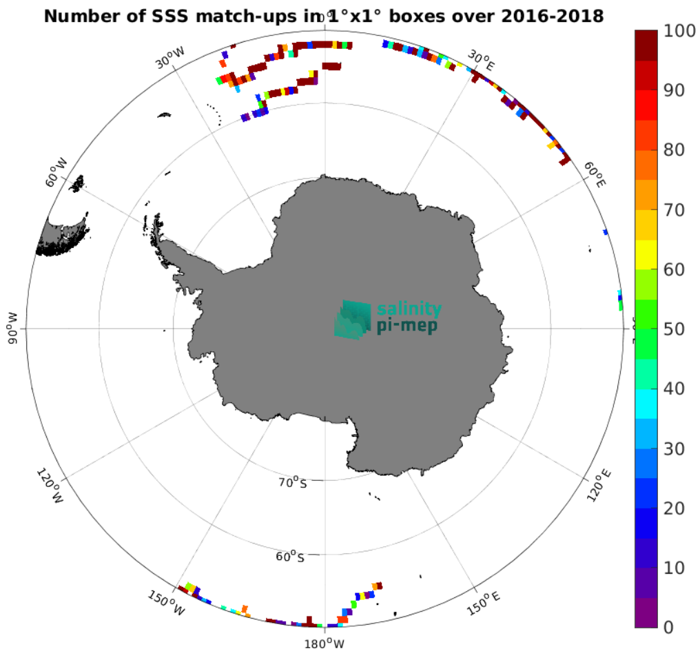
Figure 4: Number of SSS match-ups between Surface drifters SSS and the SMOS SSS L2Q v331 - With FLAG (CMEMS-CATDS-CPDC) SSS product for the Southern Ocean Pi-MEP region over 1^\circ \times 1^\circ boxes and for the full satellite product period.
