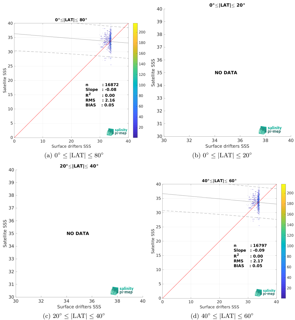
Figure 9: Contour maps of the concentration of SMOS SSS L2Q v331 - With FLAG (CMEMS-CATDS-CPDC) SSS (y-axis) versus Surface drifters SSS (x-axis) at match-up pairs for different latitude bands. For each plot, the red line shows x=y . The black thin and dashed lines indicate a linear fit through the data cloud and the \pm 95\% confidence levels, respectively. The number match-up pairs n , the slope and R^2 coefficient of the linear fit, the root mean square (RMS) and the mean bias between satellite and in situ data are indicated for each latitude band in each plots.
