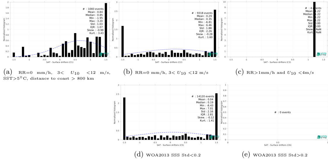
Figure 14: Normalized histogram of \Delta SSS (SMOS SSS L2Q v331 - With FLAG (CMEMS-CATDS-CPDC) - Surface drifters) for 5 different subdatasets corresponding to: RR=0 mm/h, 3 < U_{10} < 12 m/s, SST > 5°C, distance to coast > 800 km (a), RR=0 mm/h, 3 < U_{10} < 12 m/s (b), RR > 1mm/h and U_{10} < 4 m/s (c), WOA2013 SSS Std < 0.2 (d), WOA2013 SSS Std > 0.2 (e).
