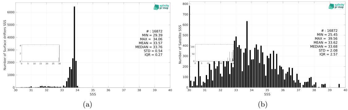
Figure 3: Histograms of SSS from Surface drifters (a) and SMOS SSS L2Q v331 - With FLAG (CMEMS-CATDS-CPDC) (b) considering all match-up pairs per bins of 0.1 over the Southern Ocean Pi-MEP region and for the full satellite product period.
