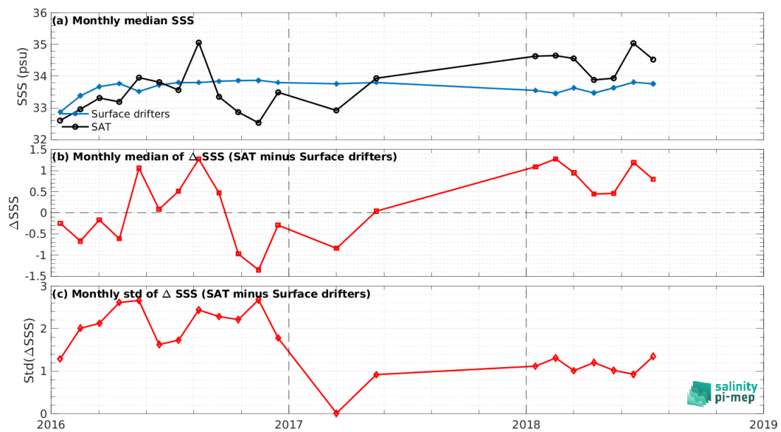
Figure 7: Time series of the monthly median SSS (top), median of \Delta SSS (Satellite - Surface drifters) and Std of \Delta SSS (Satellite - Surface drifters) over the Southern Ocean Pi-MEP region considering all match-ups collected by the Pi-MEP.
