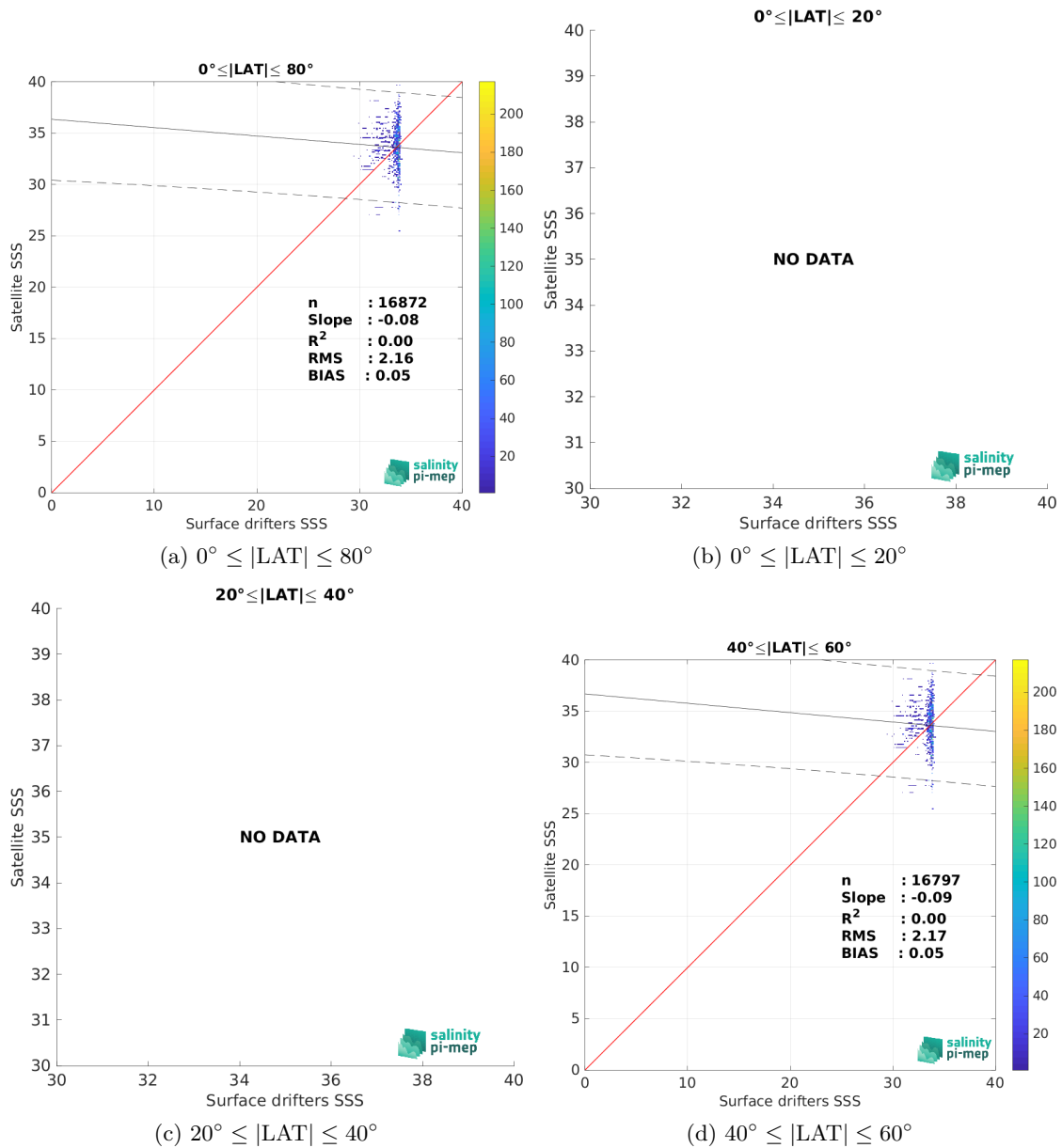
Figure 8: Contour maps of the concentration of SMOS SSS L2Q v331 - With FLAG (CMEMS-CATDS-CPDC) SSS (y-axis) versus Surface drifters SSS (x-axis) at match-up pairs for different latitude bands. For each plot, the red line shows x=y . The black thin and dashed lines indicate a linear fit through the data cloud and the \pm 95\% confidence levels, respectively. The number match-up pairs n , the slope and R^2 coefficient of the linear fit, the root mean square (RMS) and the mean bias between satellite and in situ data are indicated for each latitude band in each plots.
