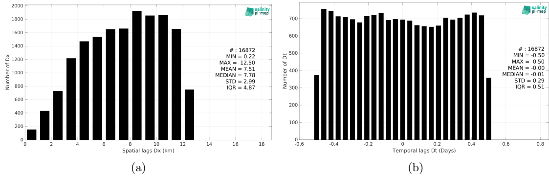
Figure 4: Histograms of the spatial (a) and temporal (b) lags between the location/time of the Surface drifters measurement and the date of the corresponding SMOS SSS L2Q v331 - With FLAG (CMEMS-CATDS-CPDC) SSS pixel.
