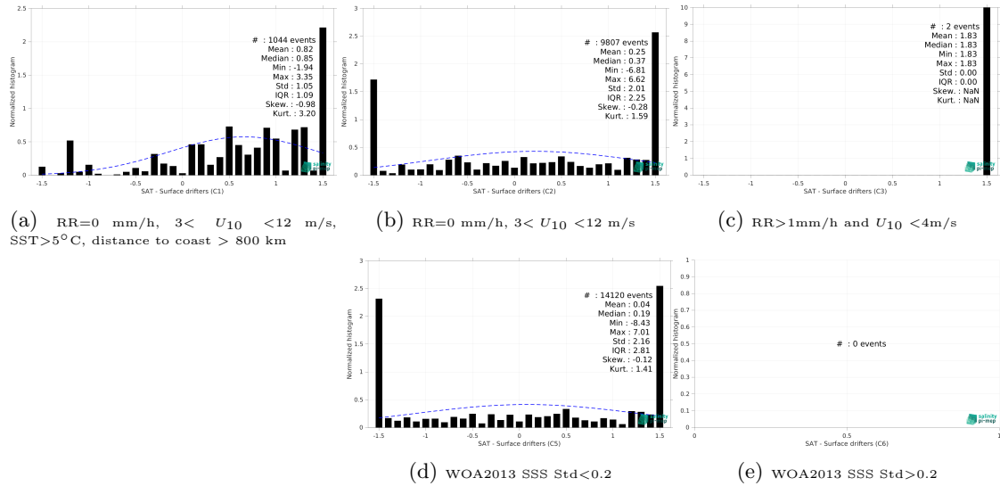
Figure 12: Normalized histogram of \Delta SSS (SMOS SSS L2Q v331 - With FLAG (CMEMS-CATDS-CPDC) - Surface drifters) for 5 different subdatasets corresponding to: RR=0 mm/h, 3 < U_{10} < 12 m/s, SST>5°C, distance to coast > 800 km (a), RR=0 mm/h, 3 < U_{10} < 12 m/s (b), RR>1mm/h and U_{10} < 4 m/s (c), WOA2013 SSS Std<0.2 (d), WOA2013 SSS Std>0.2 (e).
