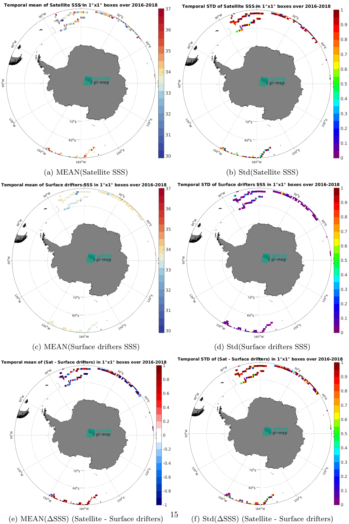
Figure 5: Temporal mean (left) and Std (right) of SSS from SMOS SSS L2Q v331 - With FLAG (CMEMS-CATDS-CPDC) (top), Surface drifters (middle), and of \Delta SSS (Satellite - Surface drifters). Only match-up pairs are used to generate these maps.
