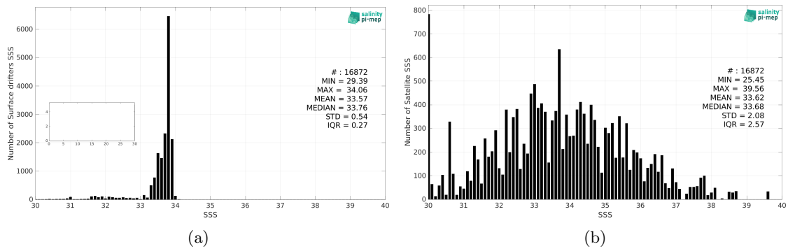
Figure 2: Histograms of SSS from Surface drifters (a) and SMOS SSS L2Q v331 - With FLAG (CMEMS-CATDS-CPDC) (b) considering all match-up pairs per bins of 0.1 over the Southern Ocean Pi-MEP region and for the full satellite product period.
