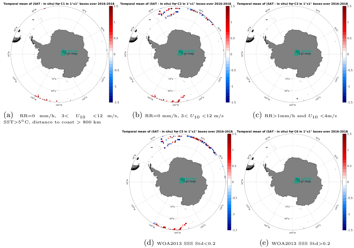
Figure 11: Temporal mean gridded over spatial boxes of size 1^{\circ}\times 1^{\circ} of \Delta\text{SSS} (SMOS SSS L2Q v331 - With FLAG (CMEMS-CATDS-CPDC) - Surface drifters) for 5 different subdatasets corresponding to:RR=0 mm/h, 3 < U_{10} < 12 m/s, SST >5^{\circ}\text{C} , distance to coast > 800 km (a), RR=0 mm/h, 3 < U_{10} < 12 m/s (b), RR >1 mm/h and U_{10} < 4 m/s (c), WOA2013 SSS Std <0.2 (d), WOA2013 SSS Std >0.2 (e).
