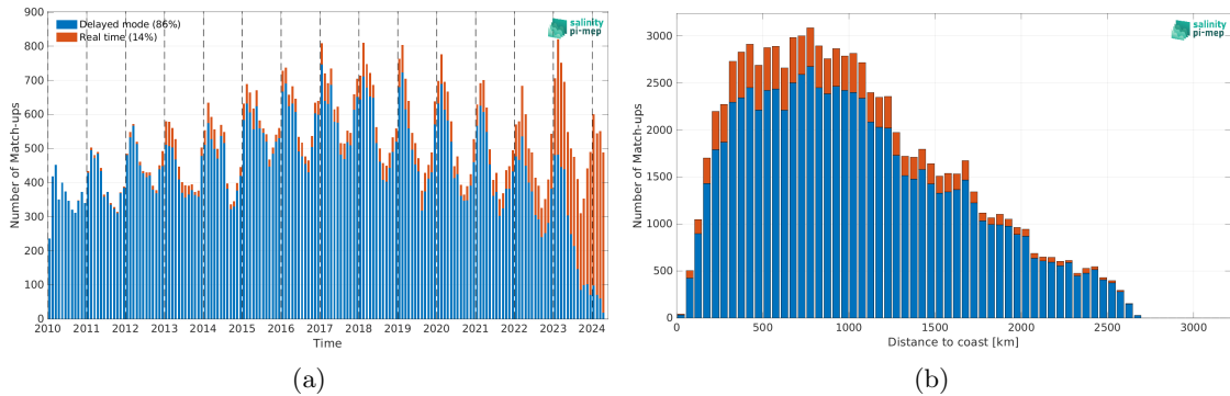
Figure 2: Number of match-ups between Argo and SMOS SSS L2Q v331 - With FLAG (CMEMS-CATDS-CPDC) SSS as a function of time (a) and as function of the distance to coast (b) over the Southern Ocean Pi-MEP region and for the full satellite product period.
