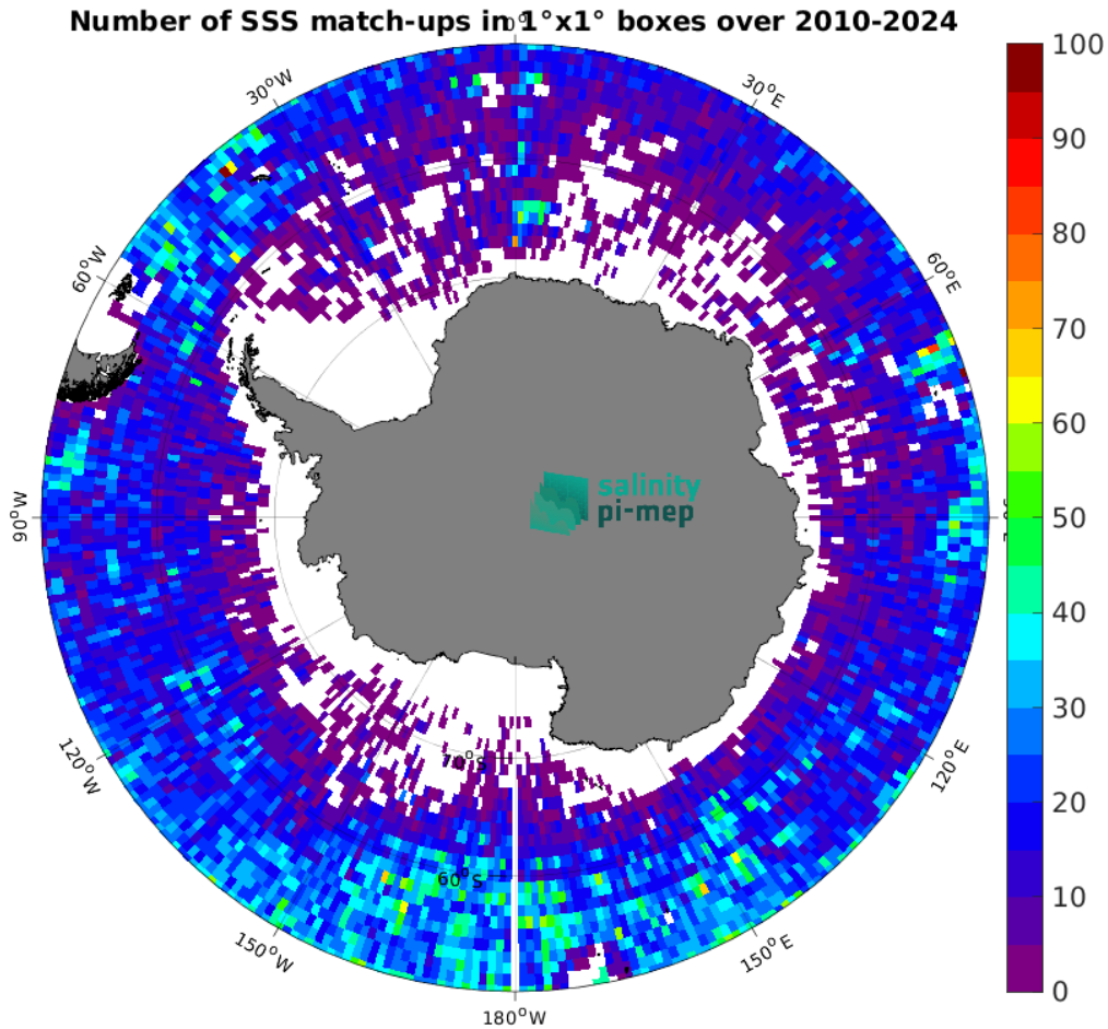
Figure 5: Number of SSS match-ups between Argo SSS and the SMOS SSS L2Q v331 - With FLAG (CMEMS-CATDS-CPDC) SSS product for the Southern Ocean Pi-MEP region over 1^\circ \times 1^\circ boxes and for the full satellite product period.
