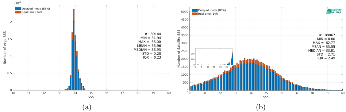
Figure 3: Histograms of SSS from Argo (a) and SMOS SSS L2Q v331 - With FLAG (CMEMS-CATDS-CPDC) (b) considering all match-up pairs per bins of 0.1 over the Southern Ocean Pi-MEP region and for the full satellite product period.
