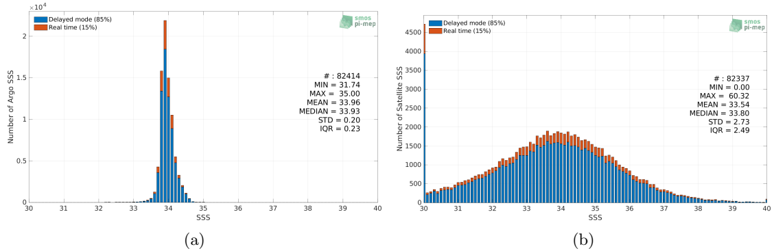
Figure 2: Histograms of SSS from Argo (a) and SMOS SSS L2Q v331 - With FLAG (CMEMS-CATDS-CPDC) (b) considering all match-up pairs per bins of 0.1 over the Southern Ocean Pi-MEP region and for the full satellite product period.
