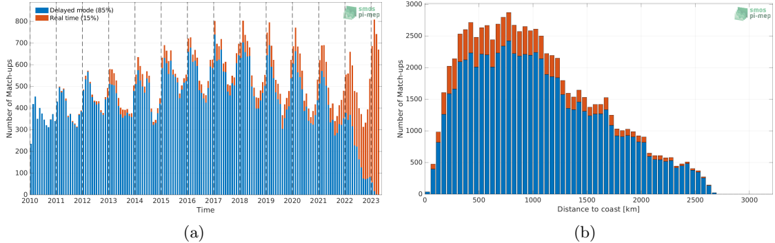
Figure 1: Number of match-ups between Argo and SMOS SSS L2Q v331 - With FLAG (CMEMS-CATDS-CPDC) SSS as a function of time (a) and as function of the distance to coast (b) over the Southern Ocean Pi-MEP region and for the full satellite product period.
