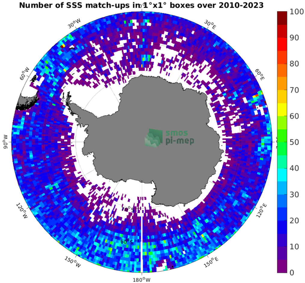
Figure 4: Number of SSS match-ups between Argo SSS and the SMOS SSS L2Q v331 - With FLAG (CMEMS-CATDS-CPDC) SSS product for the Southern Ocean Pi-MEP region over 1^\circ \times 1^\circ boxes and for the full satellite product period.
