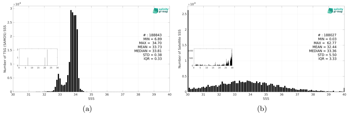
Figure 3: Histograms of SSS from TSG (SAMOS) (a) and SMOS SSS L2Q v331 - No FLAG (CMEMS-CATDS-CPDC) (b) considering all match-up pairs per bins of 0.1 over the Southern Ocean Pi-MEP region and for the full satellite product period.
