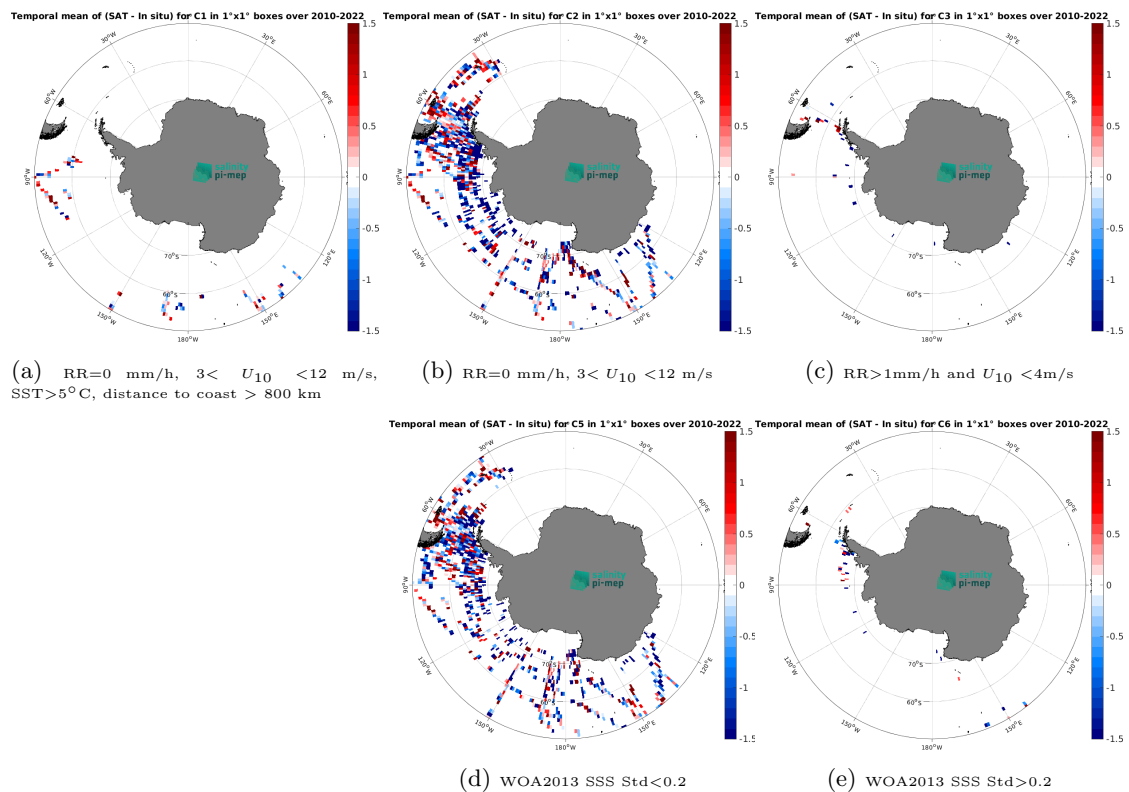
Figure 14: Temporal mean gridded over spatial boxes of size 1^\circ \times 1^\circ of \Delta\text{SSS} (SMOS SSS L2Q v331 - No FLAG (CMEMS-CATDS-CPDC) - TSG (SAMOS)) for 5 different subdatasets corresponding to:RR=0 mm/h, 3 < U_{10} < 12 m/s, SST>5°C, distance to coast > 800 km (a), RR=0 mm/h, 3 < U_{10} < 12 m/s (b), RR>1mm/h and U_{10} < 4 m/s (c), WOA2013 SSS Std<0.2 (d), WOA2013 SSS Std>0.2 (e).
