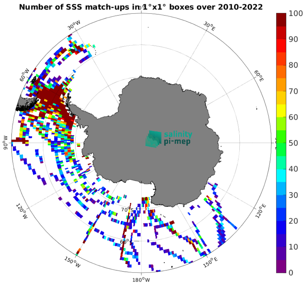
Figure 5: Number of SSS match-ups between TSG (SAMOS) SSS and the SMOS SSS L2Q v331 - No FLAG (CMEMS-CATDS-CPDC) SSS product for the Southern Ocean Pi-MEP region over 1^\circ \times 1^\circ boxes and for the full satellite product period.
