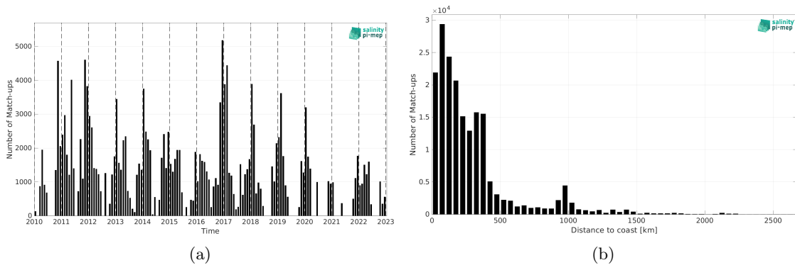
Figure 2: Number of match-ups between TSG (SAMOS) and SMOS SSS L2Q v331 - No FLAG (CMEMS-CATDS-CPDC) SSS as a function of time (a) and as function of the distance to coast (b) over the Southern Ocean Pi-MEP region and for the full satellite product period.
