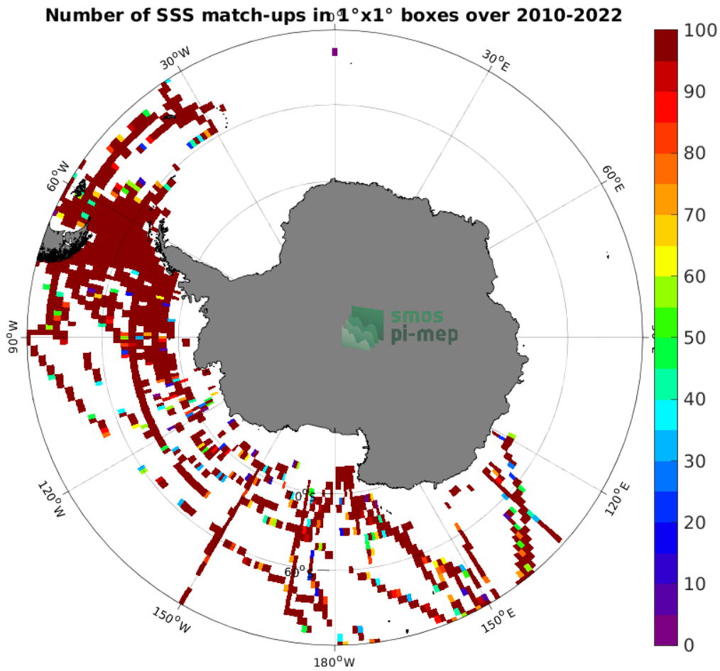
Figure 4: Number of SSS match-ups between TSG (SAMOS) SSS and the SMOS SSS L2Q v331 - No FLAG (CMEMS-CATDS-CPDC) SSS product for the Southern Ocean Pi-MEP region over 1^\circ \times 1^\circ boxes and for the full satellite product period.
