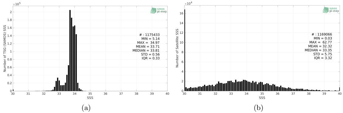
Figure 2: Histograms of SSS from TSG (SAMOS) (a) and SMOS SSS L2Q v331 - No FLAG (CMEMS-CATDS-CPDC) (b) considering all match-up pairs per bins of 0.1 over the Southern Ocean Pi-MEP region and for the full satellite product period.
