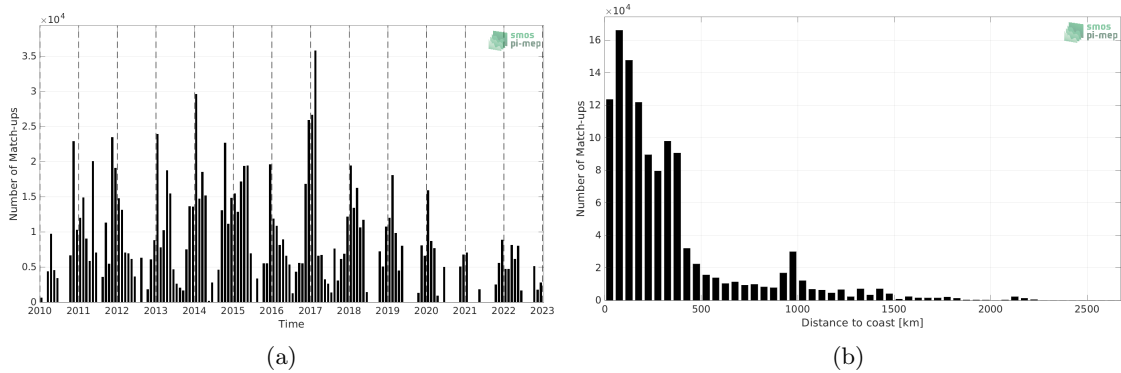
Figure 1: Number of match-ups between TSG (SAMOS) and SMOS SSS L2Q v331 - No FLAG (CMEMS-CATDS-CPDC) SSS as a function of time (a) and as function of the distance to coast (b) over the Southern Ocean Pi-MEP region and for the full satellite product period.
