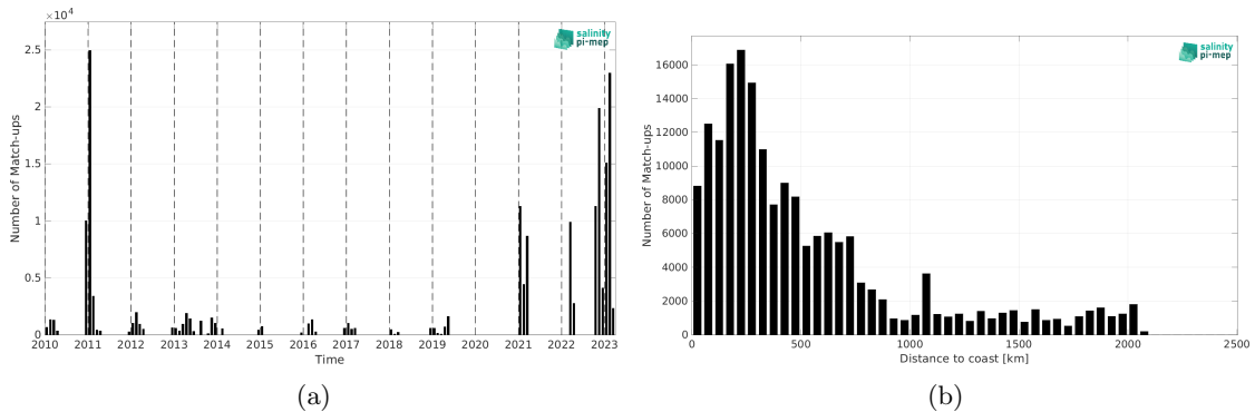
Figure 2: Number of match-ups between TSG (Polarstern) and SMOS SSS L2Q v331 - No FLAG (CMEMS-CATDS-CPDC) SSS as a function of time (a) and as function of the distance to coast (b) over the Southern Ocean Pi-MEP region and for the full satellite product period.
