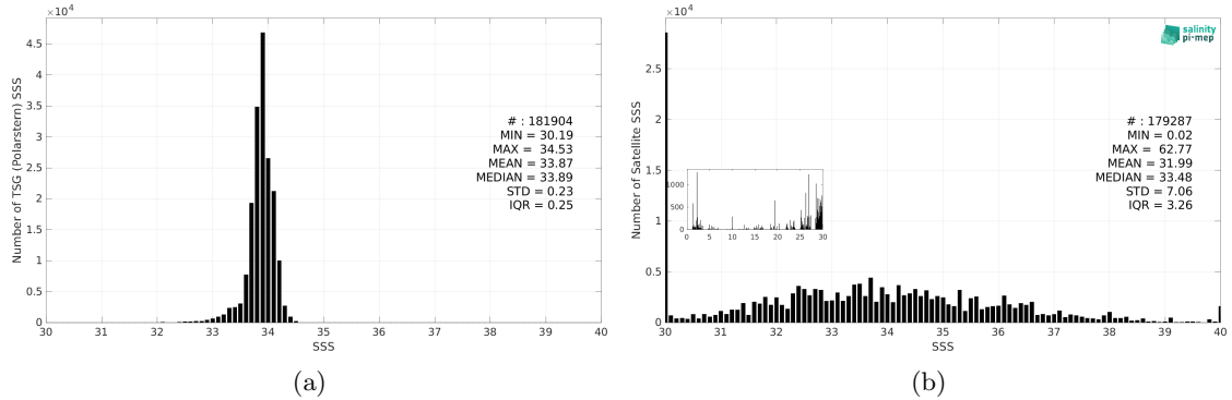
Figure 3: Histograms of SSS from TSG (Polarstern) (a) and SMOS SSS L2Q v331 - No FLAG (CMEMS-CATDS-CPDC) (b) considering all match-up pairs per bins of 0.1 over the Southern Ocean Pi-MEP region and for the full satellite product period.
