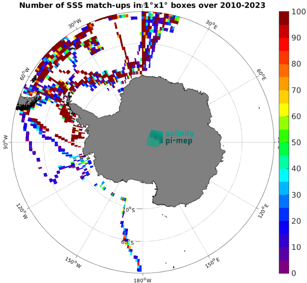
Figure 5: Number of SSS match-ups between TSG (Polarstern) SSS and the SMOS SSS L2Q v331 - No FLAG (CMEMS-CATDS-CPDC) SSS product for the Southern Ocean Pi-MEP region over 1^\circ \times 1^\circ boxes and for the full satellite product period.
