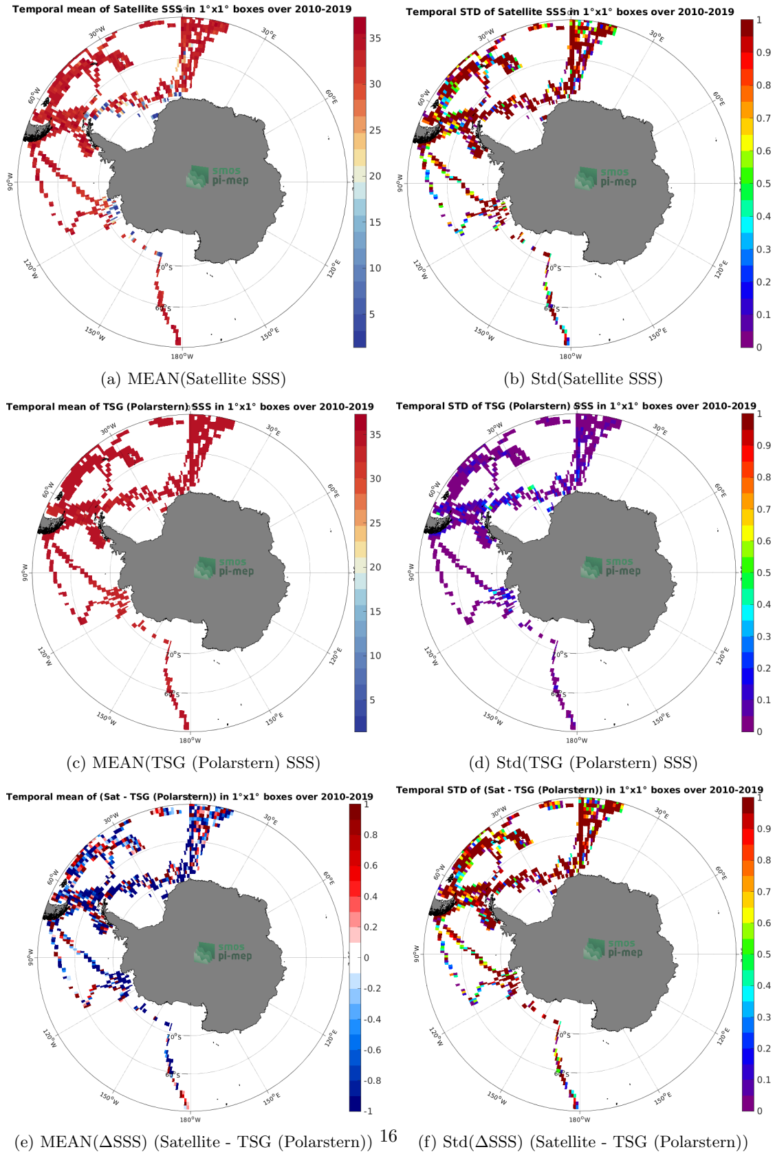
Figure 6: Temporal mean (left) and Std (right) of SSS from SMOS SSS L2Q v331 - No FLAG (CMEMS-CATDS-CPDC) (top), TSG (Polarstern) (middle), and of \Delta SSS (Satellite - TSG (Polarstern)). Only match-up pairs are used to generate these maps.
