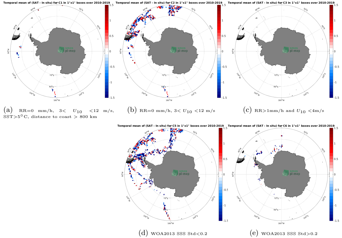
Figure 12: Temporal mean gridded over spatial boxes of size 1^{\circ}\times 1^{\circ} of \Delta\text{SSS} (SMOS SSS L2Q v331 - No FLAG (CMEMS-CATDS-CPDC) - TSG (Polarstern)) for 5 different subdatasets corresponding to:RR=0 mm/h, 3 < U_{10} < 12 m/s, SST >5^{\circ}\text{C} , distance to coast > 800 km (a), RR=0 mm/h, 3 < U_{10} < 12 m/s (b), RR >1 mm/h and U_{10} < 4 m/s (c), WOA2013 SSS Std <0.2 (d), WOA2013 SSS Std >0.2 (e).
