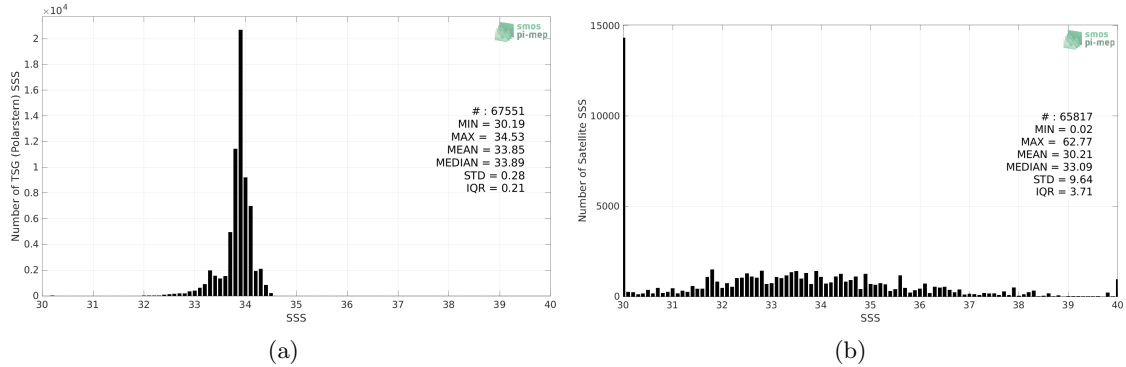
Figure 2: Histograms of SSS from TSG (Polarstern) (a) and SMOS SSS L2Q v331 - No FLAG (CMEMS-CATDS-CPDC) (b) considering all match-up pairs per bins of 0.1 over the Southern Ocean Pi-MEP region and for the full satellite product period.
