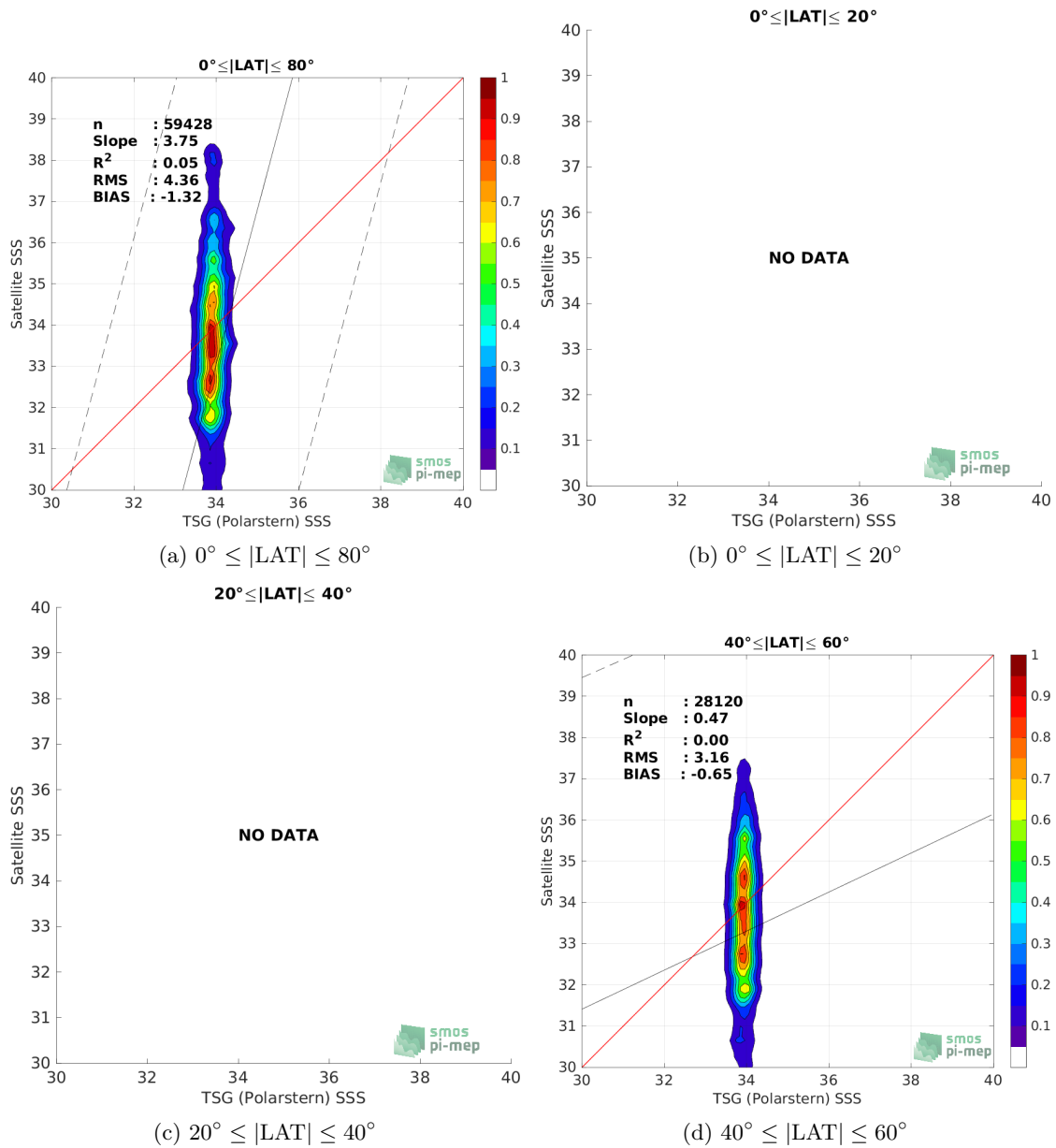
Figure 9: Contour maps of the concentration of SMOS SSS L2Q v331 - No FLAG (CMEMS-CATDS-CPDC) SSS (y-axis) versus TSG (Polarstern) SSS (x-axis) at match-up pairs for different latitude bands. For each plot, the red line shows x=y . The black thin and dashed lines indicate a linear fit through the data cloud and the \pm 95\% confidence levels, respectively. The number match-up pairs n , the slope and R^2 coefficient of the linear fit, the root mean square (RMS) and the mean bias between satellite and in situ data are indicated for each latitude band in each plots.
