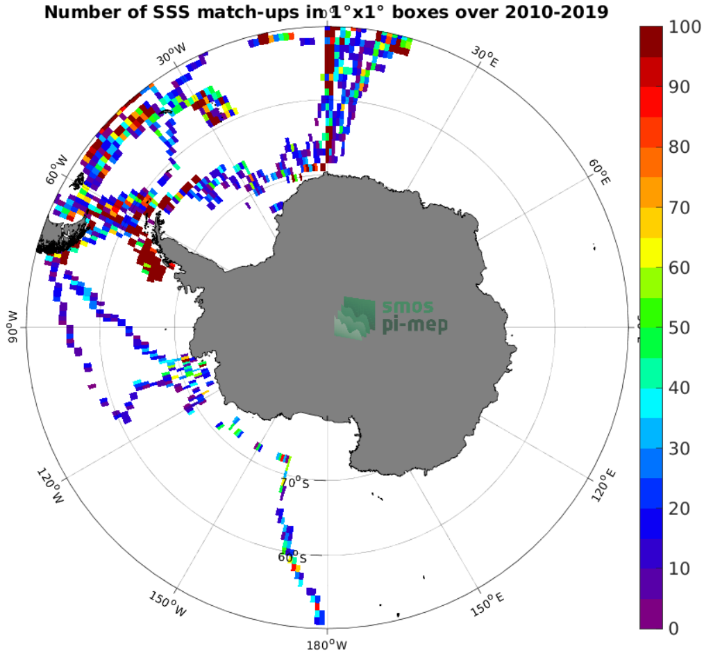
Figure 4: Number of SSS match-ups between TSG (Polarstern) SSS and the SMOS SSS L2Q v331 - No FLAG (CMEMS-CATDS-CPDC) SSS product for the Southern Ocean Pi-MEP region over 1^\circ \times 1^\circ boxes and for the full satellite product period.
