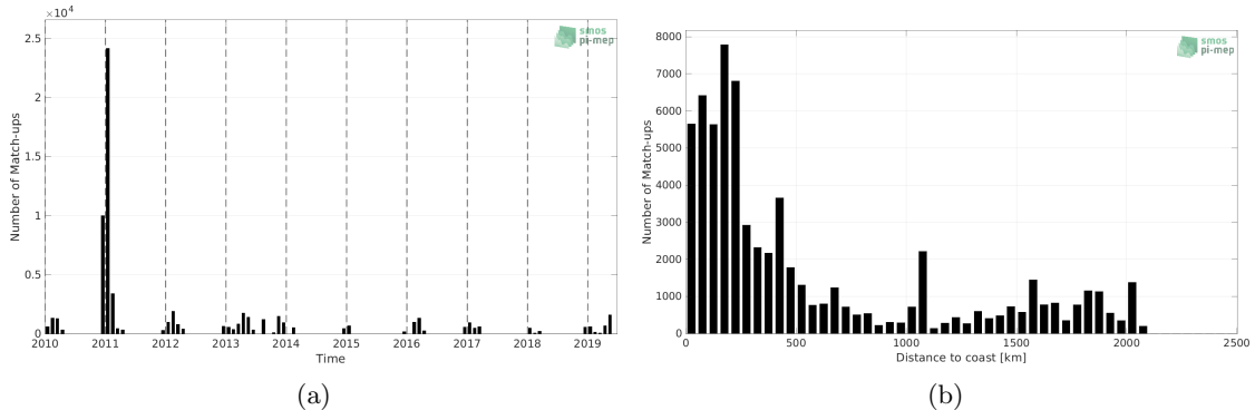
Figure 1: Number of match-ups between TSG (Polarstern) and SMOS SSS L2Q v331 - No FLAG (CMEMS-CATDS-CPDC) SSS as a function of time (a) and as function of the distance to coast (b) over the Southern Ocean Pi-MEP region and for the full satellite product period.
