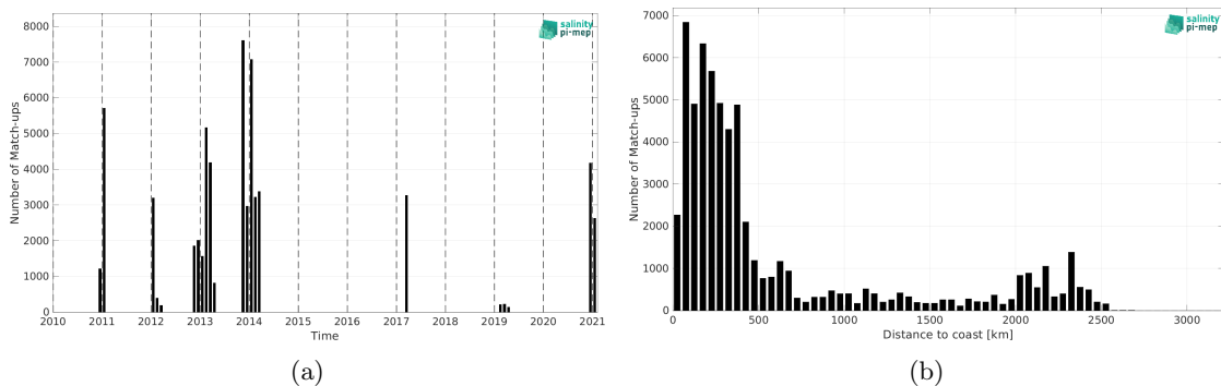
Figure 2: Number of match-ups between TSG (GOSUD-Sailing-ship) and SMOS SSS L2Q v331 - No FLAG (CMEMS-CATDS-CPDC) SSS as a function of time (a) and as function of the distance to coast (b) over the Southern Ocean Pi-MEP region and for the full satellite product period.
