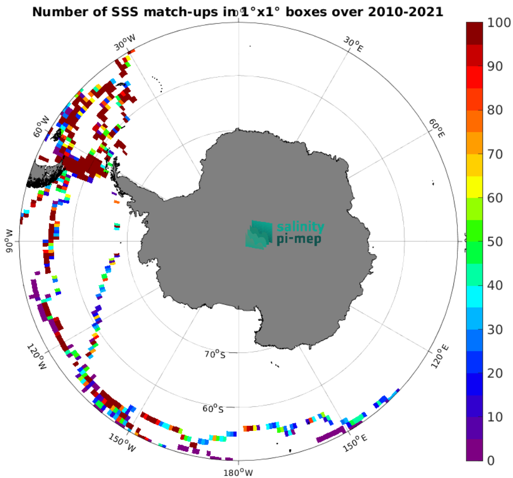
Figure 5: Number of SSS match-ups between TSG (GOSUD-Sailing-ship) SSS and the SMOS SSS L2Q v331 - No FLAG (CMEMS-CATDS-CPDC) SSS product for the Southern Ocean Pi-MEP region over 1^\circ \times 1^\circ boxes and for the full satellite product period.
