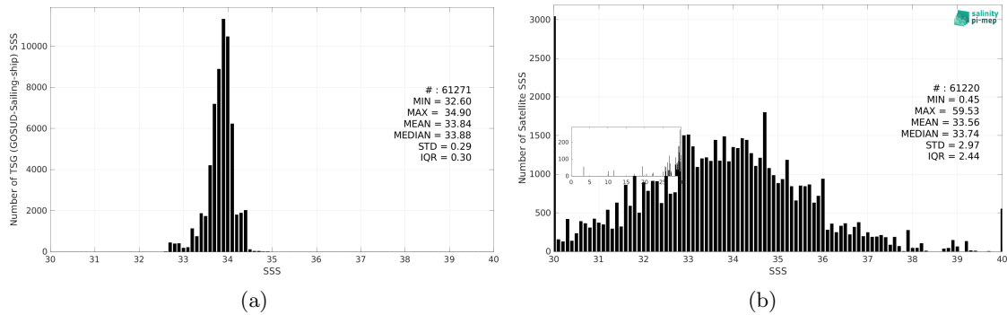
Figure 3: Histograms of SSS from TSG (GOSUD-Sailing-ship) (a) and SMOS SSS L2Q v331 - No FLAG (CMEMS-CATDS-CPDC) (b) considering all match-up pairs per bins of 0.1 over the Southern Ocean Pi-MEP region and for the full satellite product period.
