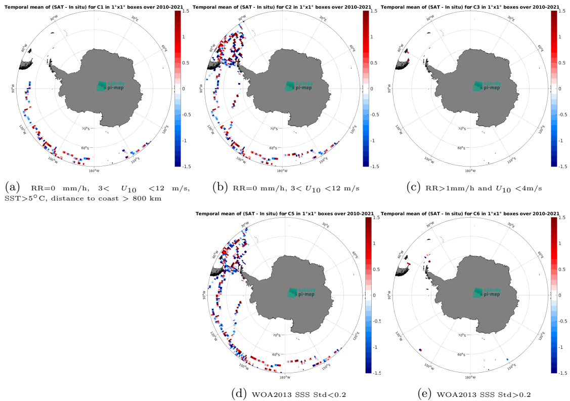
Figure 14: Temporal mean gridded over spatial boxes of size 1^\circ \times 1^\circ of \Delta\text{SSS} (SMOS SSS L2Q v331 - No FLAG (CMEMS-CATDS-CPDC) - TSG (GOSUD-Sailing-ship)) for 5 different sub-datasets corresponding to:RR=0 mm/h, 3 < U_{10} < 12 m/s, SST>5°C, distance to coast > 800 km (a), RR=0 mm/h, 3 < U_{10} < 12 m/s (b), RR>1mm/h and U_{10} < 4 m/s (c), WOA2013 SSS Std<0.2 (d), WOA2013 SSS Std>0.2 (e).
