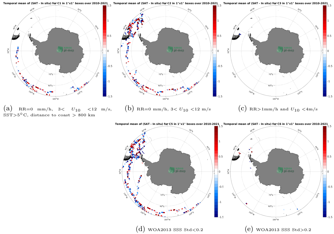
Figure 12: Temporal mean gridded over spatial boxes of size 1^\circ \times 1^\circ of \Delta SSS (SMOS SSS L2Q v331 - No FLAG (CMEMS-CATDS-CPDC) - TSG (GOSUD-Sailing-ship)) for 5 different sub-datasets corresponding to: RR=0 mm/h, 3 < U_{10} < 12 m/s, SST>5°C, distance to coast > 800 km (a), RR=0 mm/h, 3 < U_{10} < 12 m/s (b), RR>1mm/h and U_{10} < 4 m/s (c), WOA2013 SSS Std<0.2 (d), WOA2013 SSS Std>0.2 (e).
