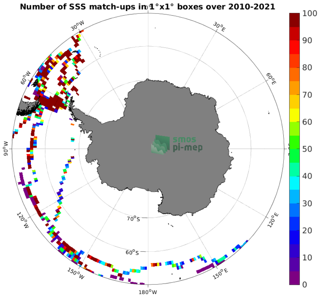
Figure 4: Number of SSS match-ups between TSG (GOSUD-Sailing-ship) SSS and the SMOS SSS L2Q v331 - No FLAG (CMEMS-CATDS-CPDC) SSS product for the Southern Ocean Pi-MEP region over 1^\circ \times 1^\circ boxes and for the full satellite product period.
