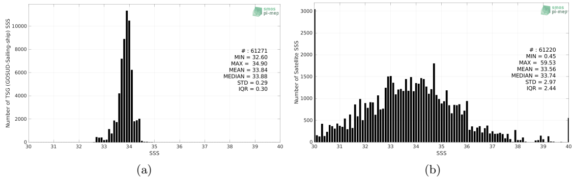
Figure 2: Histograms of SSS from TSG (GOSUD-Sailing-ship) (a) and SMOS SSS L2Q v331 - No FLAG (CMEMS-CATDS-CPDC) (b) considering all match-up pairs per bins of 0.1 over the Southern Ocean Pi-MEP region and for the full satellite product period.
