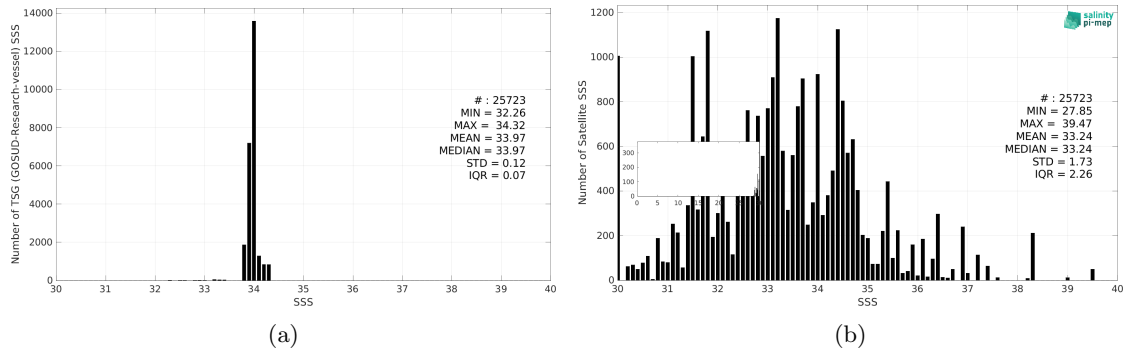
Figure 3: Histograms of SSS from TSG (GOSUD-Research-vessel) (a) and SMOS SSS L2Q v331 - No FLAG (CMEMS-CATDS-CPDC) (b) considering all match-up pairs per bins of 0.1 over the Southern Ocean Pi-MEP region and for the full satellite product period.
