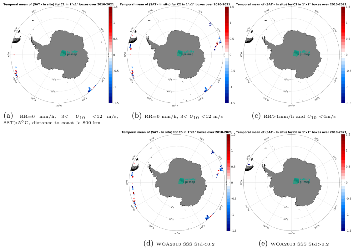
Figure 14: Temporal mean gridded over spatial boxes of size 1^\circ \times 1^\circ of \Delta\text{SSS} (SMOS SSS L2Q v331 - No FLAG (CMEMS-CATDS-CPDC) - TSG (GOSUD-Research-vessel)) for 5 different subdatasets corresponding to:RR=0 mm/h, 3 < U_{10} < 12 m/s, SST>5°C, distance to coast > 800 km (a), RR=0 mm/h, 3 < U_{10} < 12 m/s (b), RR>1mm/h and U_{10} < 4 m/s (c), WOA2013 SSS Std<0.2 (d), WOA2013 SSS Std>0.2 (e).
