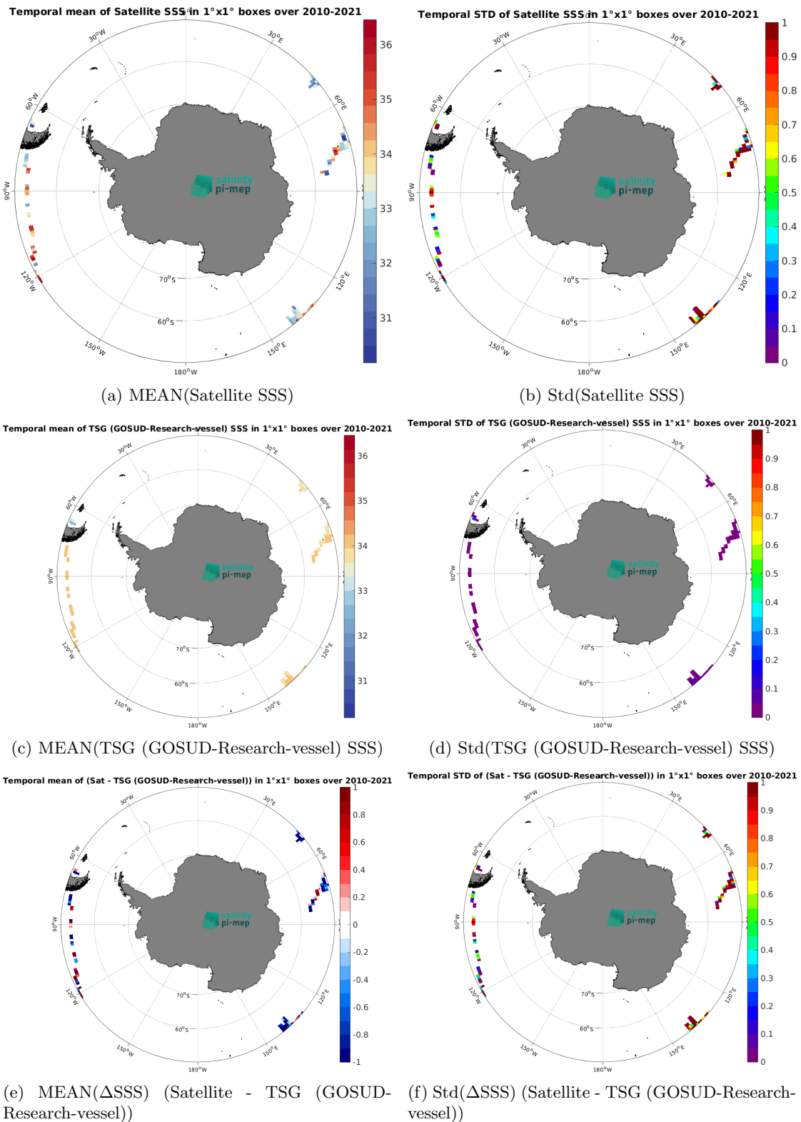
Figure 7: Temporal mean (left) and Std (right) of SSS from SMOS SSS L2Q v331 - No FLAG (CMEMS-CATDS-CPDC) (top), TSG (GOSUD-Research-vessel) (middle), and of \Delta SSS (Satellite - TSG (GOSUD-Research-vessel)). Only match-up pairs are used to generate these maps.
