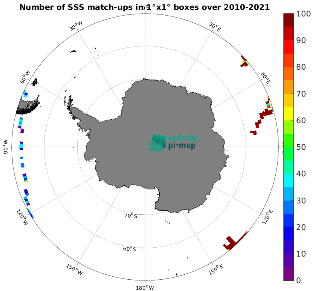
Figure 4: Number of SSS match-ups between TSG (GOSUD-Research-vessel) SSS and the SMOS SSS L2Q v331 - No FLAG (CMEMS-CATDS-CPDC) SSS product for the Southern Ocean Pi-MEP region over 1^\circ \times 1^\circ boxes and for the full satellite product period.
