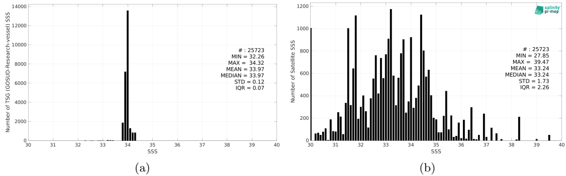
Figure 2: Histograms of SSS from TSG (GOSUD-Research-vessel) (a) and SMOS SSS L2Q v331 - No FLAG (CMEMS-CATDS-CPDC) (b) considering all match-up pairs per bins of 0.1 over the Southern Ocean Pi-MEP region and for the full satellite product period.
