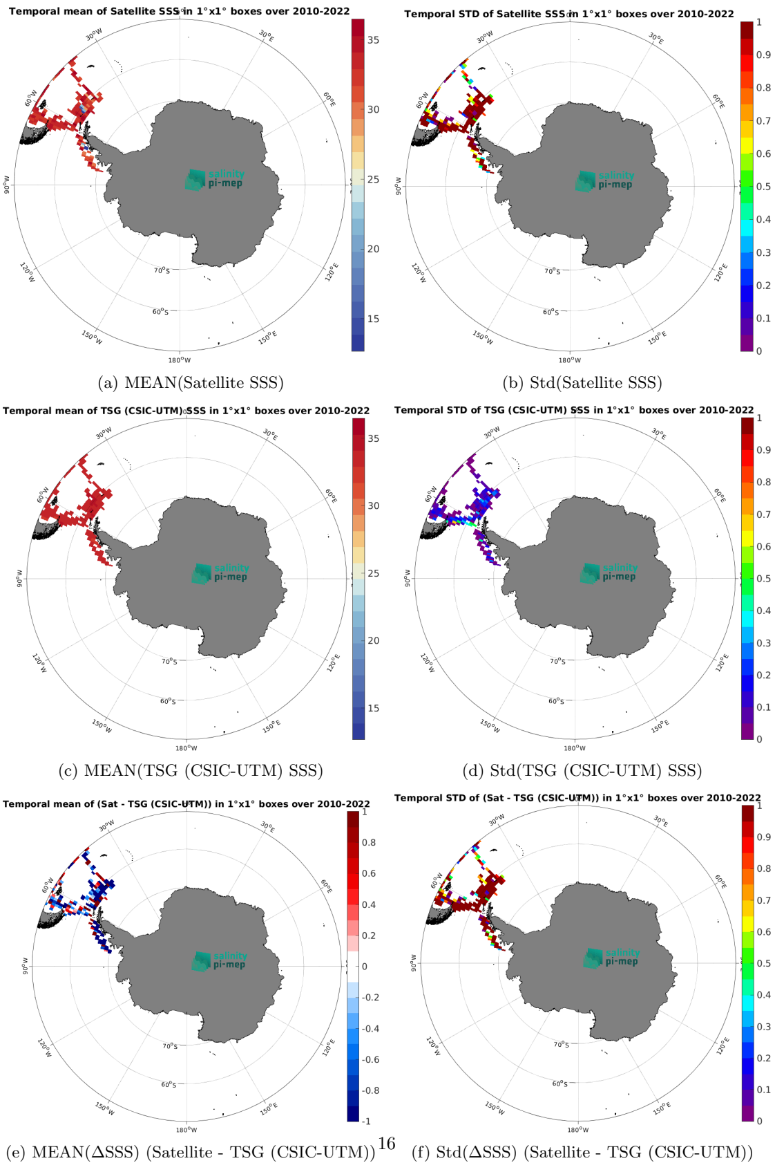
Figure 7: Temporal mean (left) and Std (right) of SSS from SMOS SSS L2Q v331 - No FLAG (CMEMS-CATDS-CPDC) (top), TSG (CSIC-UTM) (middle), and of \Delta SSS (Satellite - TSG (CSIC-UTM)). Only match-up pairs are used to generate these maps.
