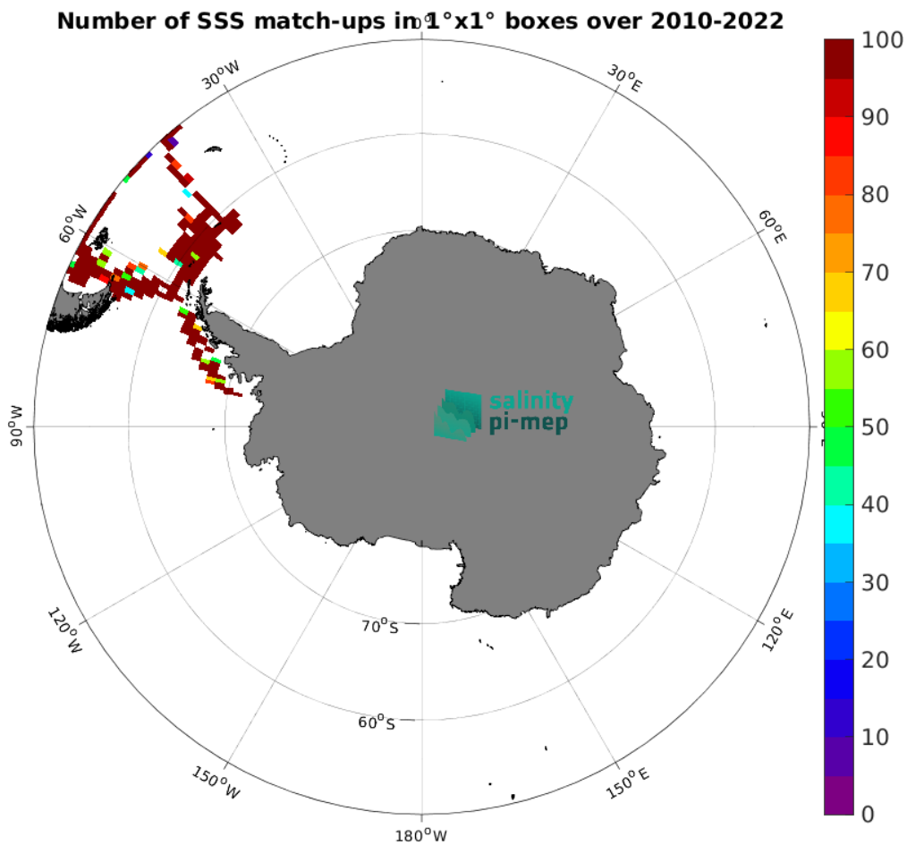
Figure 5: Number of SSS match-ups between TSG (CSIC-UTM) SSS and the SMOS SSS L2Q v331 - No FLAG (CMEMS-CATDS-CPDC) SSS product for the Southern Ocean Pi-MEP region over 1^{\circ} \times 1^{\circ} boxes and for the full satellite product period.
