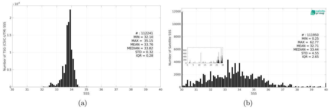
Figure 3: Histograms of SSS from TSG (CSIC-UTM) (a) and SMOS SSS L2Q v331 - No FLAG (CMEMS-CATDS-CPDC) (b) considering all match-up pairs per bins of 0.1 over the Southern Ocean Pi-MEP region and for the full satellite product period.
