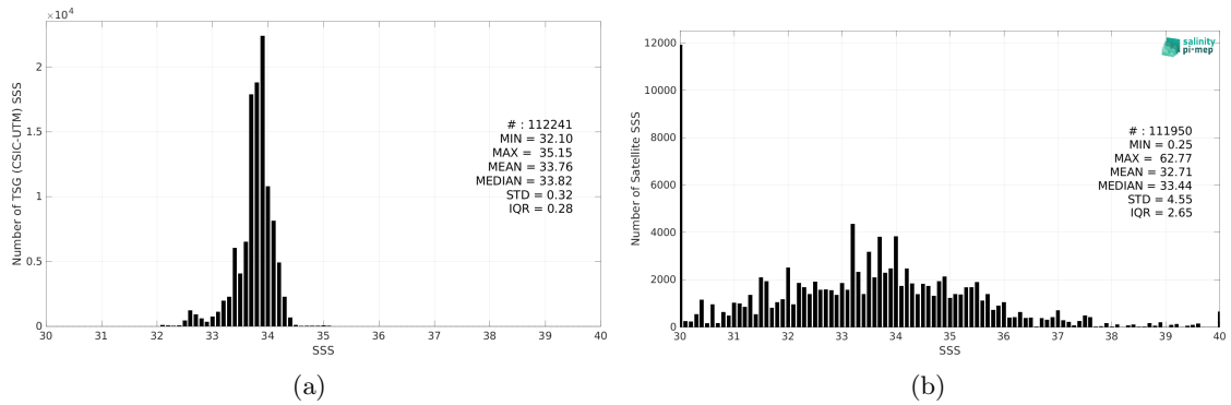
Figure 2: Histograms of SSS from TSG (CSIC-UTM) (a) and SMOS SSS L2Q v331 - No FLAG (CMEMS-CATDS-CPDC) (b) considering all match-up pairs per bins of 0.1 over the Southern Ocean Pi-MEP region and for the full satellite product period.
