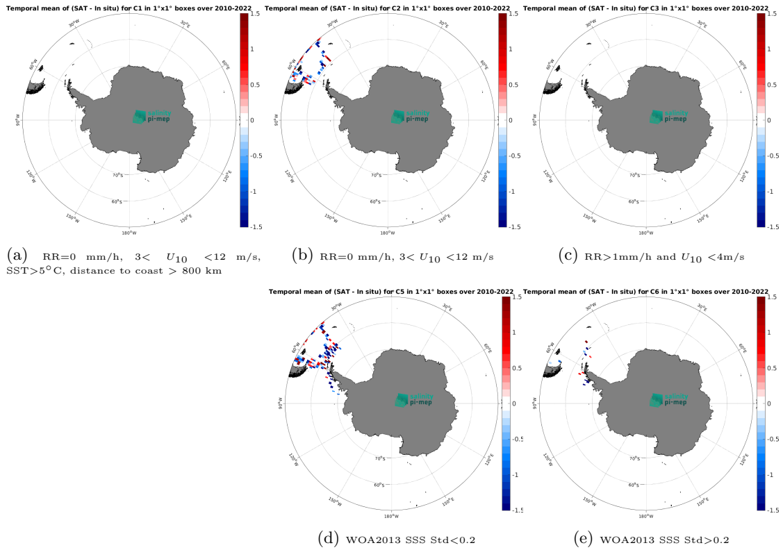
Figure 12: Temporal mean gridded over spatial boxes of size 1^{\circ}\times 1^{\circ} of \Delta\text{SSS} (SMOS SSS L2Q v331 - No FLAG (CMEMS-CATDS-CPDC) - TSG (CSIC-UTM)) for 5 different subdatasets corresponding to:RR=0 mm/h, 3 < U_{10} < 12 m/s, SST >5^{\circ}\text{C} , distance to coast > 800 km (a), RR=0 mm/h, 3 < U_{10} < 12 m/s (b), RR >1 mm/h and U_{10} < 4 m/s (c), WOA2013 SSS Std <0.2 (d), WOA2013 SSS Std >0.2 (e).
