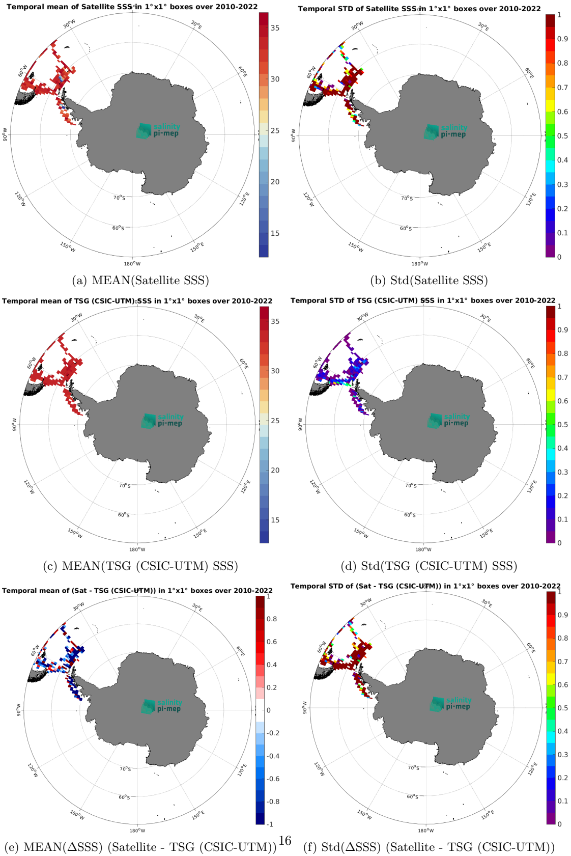
Figure 6: Temporal mean (left) and Std (right) of SSS from SMOS SSS L2Q v331 - No FLAG (CMEMS-CATDS-CPDC) (top), TSG (CSIC-UTM) (middle), and of \Delta SSS (Satellite - TSG (CSIC-UTM)). Only match-up pairs are used to generate these maps.
