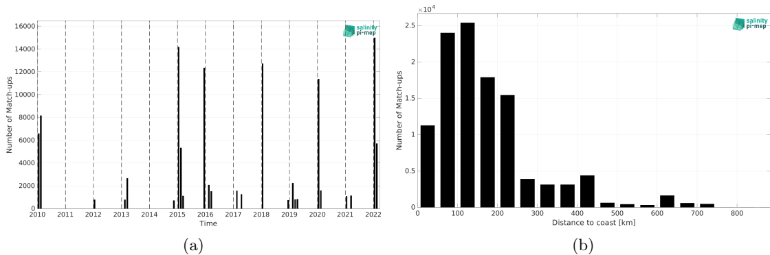
Figure 1: Number of match-ups between TSG (CSIC-UTM) and SMOS SSS L2Q v331 - No FLAG (CMEMS-CATDS-CPDC) SSS as a function of time (a) and as function of the distance to coast (b) over the Southern Ocean Pi-MEP region and for the full satellite product period.
