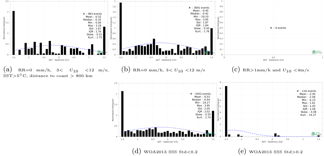
Figure 13: Normalized histogram of \Delta SSS (SMOS SSS L2Q v331 - No FLAG (CMEMS-CATDS-CPDC) - Sairdrone) for 5 different subdatasets corresponding to: RR=0 mm/h, 3 < U_{10} < 12 m/s, SST > 5°C, distance to coast > 800 km (a), RR=0 mm/h, 3 < U_{10} < 12 m/s (b), RR > 1mm/h and U_{10} < 4 m/s (c), WOA2013 SSS Std < 0.2 (d), WOA2013 SSS Std > 0.2 (e).
