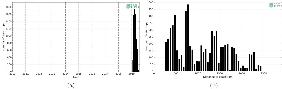
Figure 1: Number of match-ups between Saildrone and SMOS SSS L2Q v331 - No FLAG (CMEMS-CATDS-CPDC) SSS as a function of time (a) and as function of the distance to coast (b) over the Southern Ocean Pi-MEP region and for the full satellite product period.
