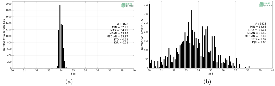
Figure 2: Histograms of SSS from Saildrone (a) and SMOS SSS L2Q v331 - No FLAG (CMEMS-CATDS-CPDC) (b) considering all match-up pairs per bins of 0.1 over the Southern Ocean Pi-MEP region and for the full satellite product period.
