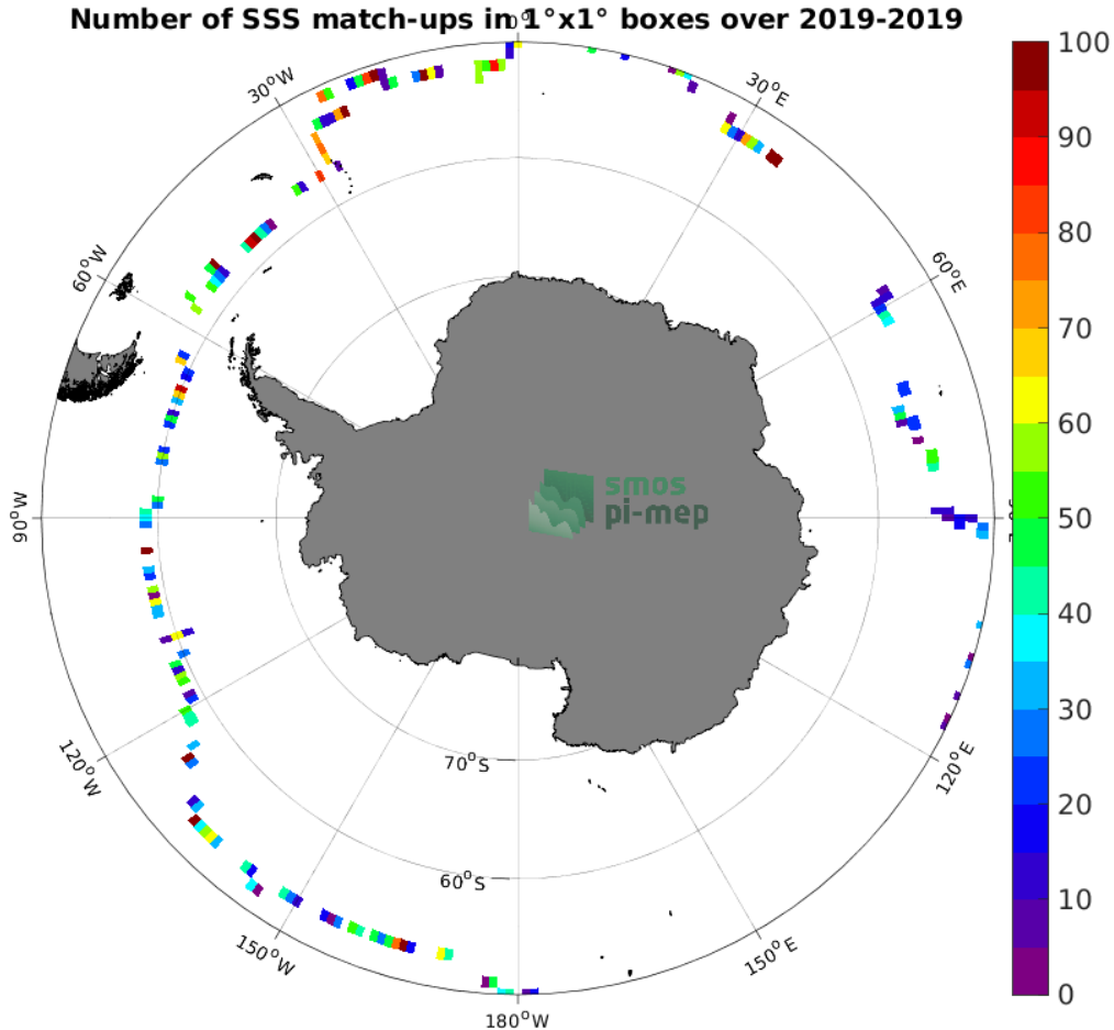
Figure 4: Number of SSS match-ups between Saildrone SSS and the SMOS SSS L2Q v331 - No FLAG (CMEMS-CATDS-CPDC) SSS product for the Southern Ocean Pi-MEP region over 1^\circ \times 1^\circ boxes and for the full satellite product period.
