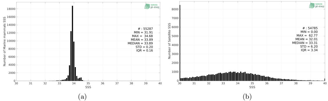
Figure 2: Histograms of SSS from Marine mammals (a) and SMOS SSS L2Q v331 - No FLAG (CMEMS-CATDS-CPDC) (b) considering all match-up pairs per bins of 0.1 over the Southern Ocean Pi-MEP region and for the full satellite product period.
