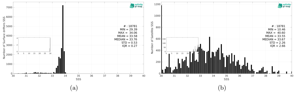
Figure 3: Histograms of SSS from Surface drifters (a) and SMOS SSS L2Q v331 - No FLAG (CMEMS-CATDS-CPDC) (b) considering all match-up pairs per bins of 0.1 over the Southern Ocean Pi-MEP region and for the full satellite product period.
