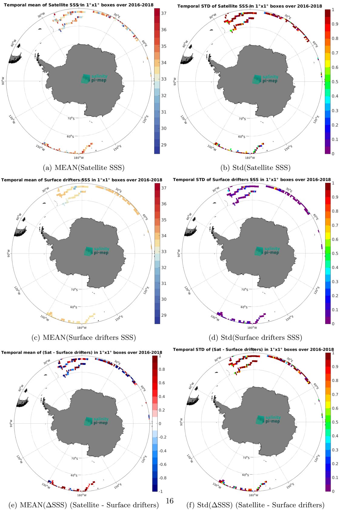
Figure 6: Temporal mean (left) and Std (right) of SSS from SMOS SSS L2Q v331 - No FLAG (CMEMS-CATDS-CPDC) (top), Surface drifters (middle), and of \Delta SSS (Satellite - Surface drifters). Only match-up pairs are used to generate these maps.
