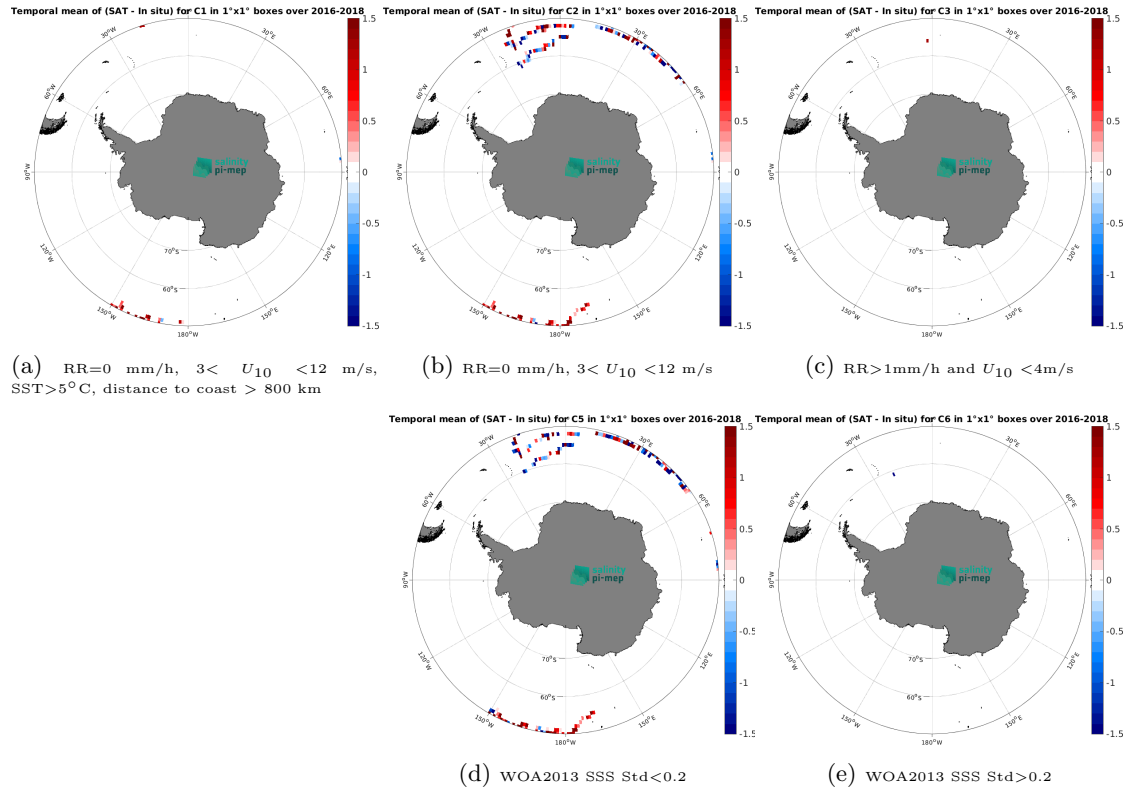
Figure 13: Temporal mean gridded over spatial boxes of size 1^\circ \times 1^\circ of \Delta SSS (SMOS SSS L2Q v331 - No FLAG (CMEMS-CATDS-CPDC) - Surface drifters) for 5 different subdatasets corresponding to:RR=0 mm/h, 3 < U_{10} < 12 m/s, SST >5^\circ C, distance to coast > 800 km (a), RR=0 mm/h, 3 < U_{10} < 12 m/s (b), RR >1 mm/h and U_{10} < 4 m/s (c), WOA2013 SSS Std <0.2 (d), WOA2013 SSS Std >0.2 (e).
