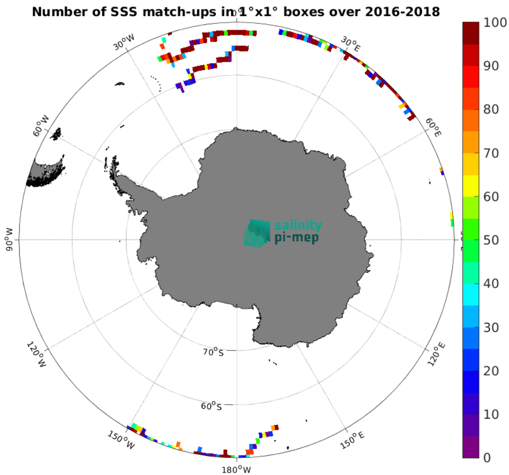
Figure 4: Number of SSS match-ups between Surface drifters SSS and the SMOS SSS L2Q v331 - No FLAG (CMEMS-CATDS-CPDC) SSS product for the Southern Ocean Pi-MEP region over 1^\circ \times 1^\circ boxes and for the full satellite product period.
