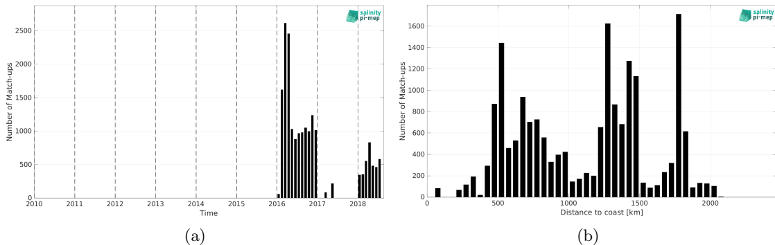
Figure 2: Number of match-ups between Surface drifters and SMOS SSS L2Q v331 - No FLAG (CMEMS-CATDS-CPDC) SSS as a function of time (a) and as function of the distance to coast (b) over the Southern Ocean Pi-MEP region and for the full satellite product period.
