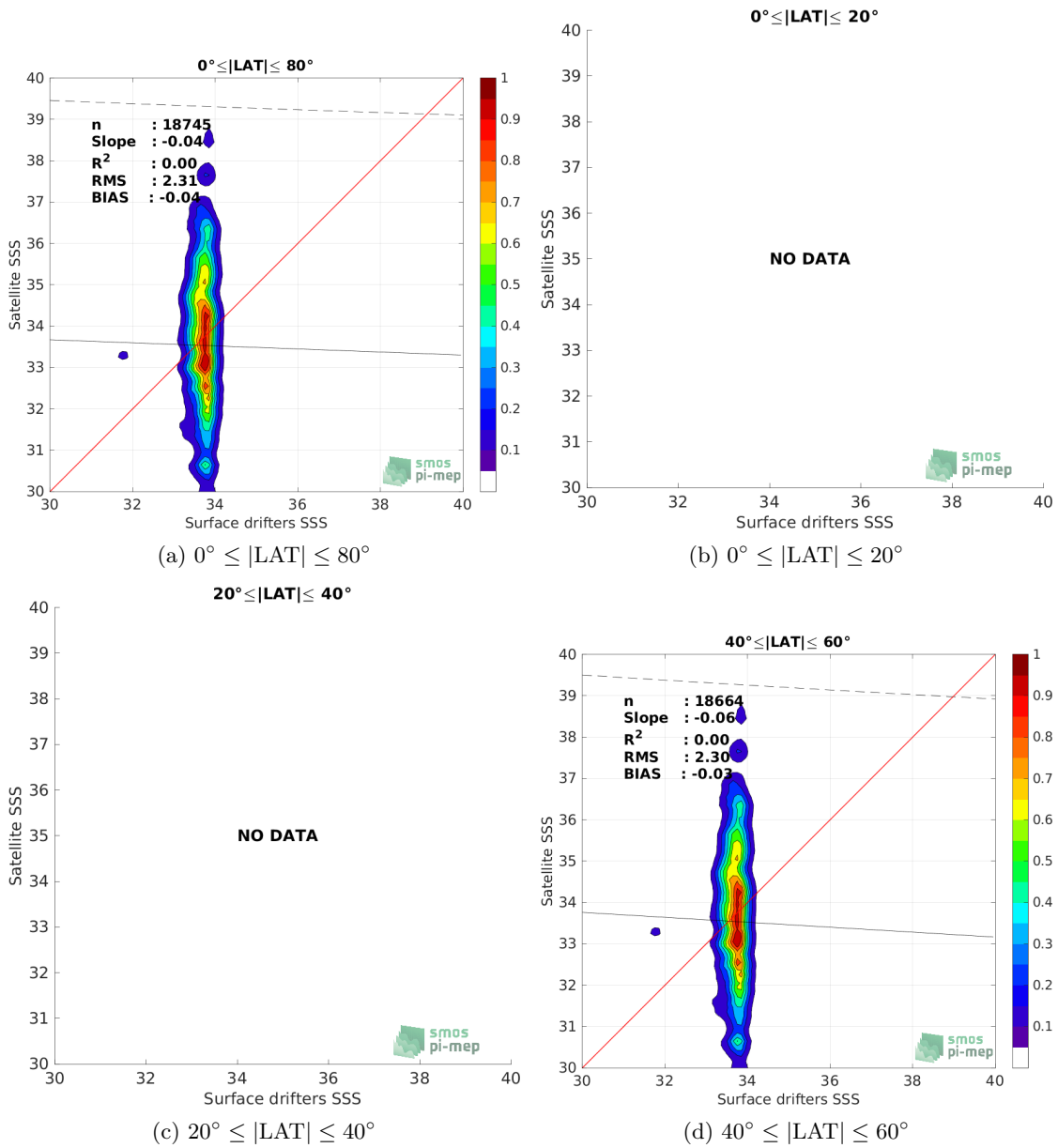
Figure 8: Contour maps of the concentration of SMOS SSS L2Q v331 - No FLAG (CMEMS-CATDS-CPDC) SSS (y-axis) versus Surface drifters SSS (x-axis) at match-up pairs for different latitude bands. For each plot, the red line shows x=y . The black thin and dashed lines indicate a linear fit through the data cloud and the \pm 95\% confidence levels, respectively. The number match-up pairs n , the slope and R^2 coefficient of the linear fit, the root mean square (RMS) and the mean bias between satellite and in situ data are indicated for each latitude band in each plots.
