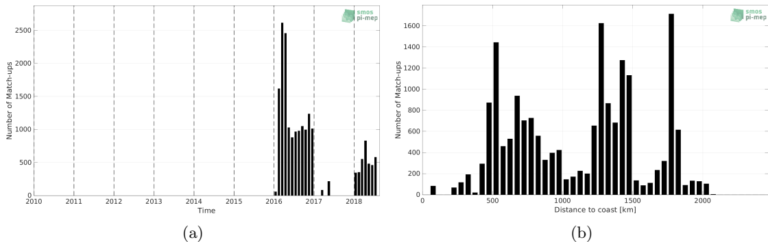
Figure 1: Number of match-ups between Surface drifters and SMOS SSS L2Q v331 - No FLAG (CMEMS-CATDS-CPDC) SSS as a function of time (a) and as function of the distance to coast (b) over the Southern Ocean Pi-MEP region and for the full satellite product period.
