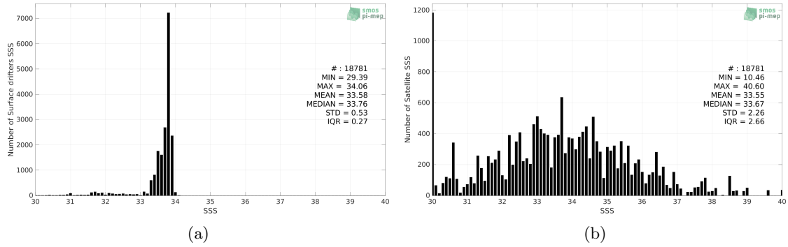
Figure 2: Histograms of SSS from Surface drifters (a) and SMOS SSS L2Q v331 - No FLAG (CMEMS-CATDS-CPDC) (b) considering all match-up pairs per bins of 0.1 over the Southern Ocean Pi-MEP region and for the full satellite product period.
