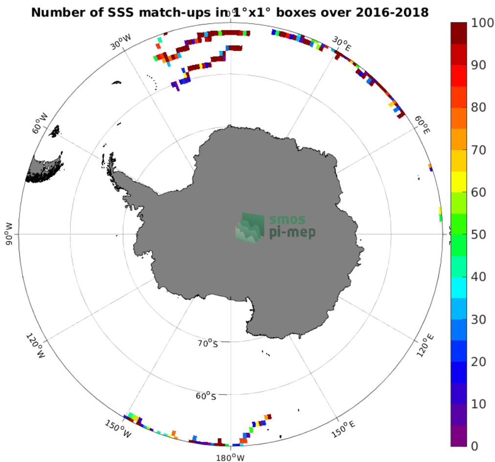
Figure 3: Number of SSS match-ups between Surface drifters SSS and the SMOS SSS L2Q v331 - No FLAG (CMEMS-CATDS-CPDC) SSS product for the Southern Ocean Pi-MEP region over 1^\circ \times 1^\circ boxes and for the full satellite product period.
