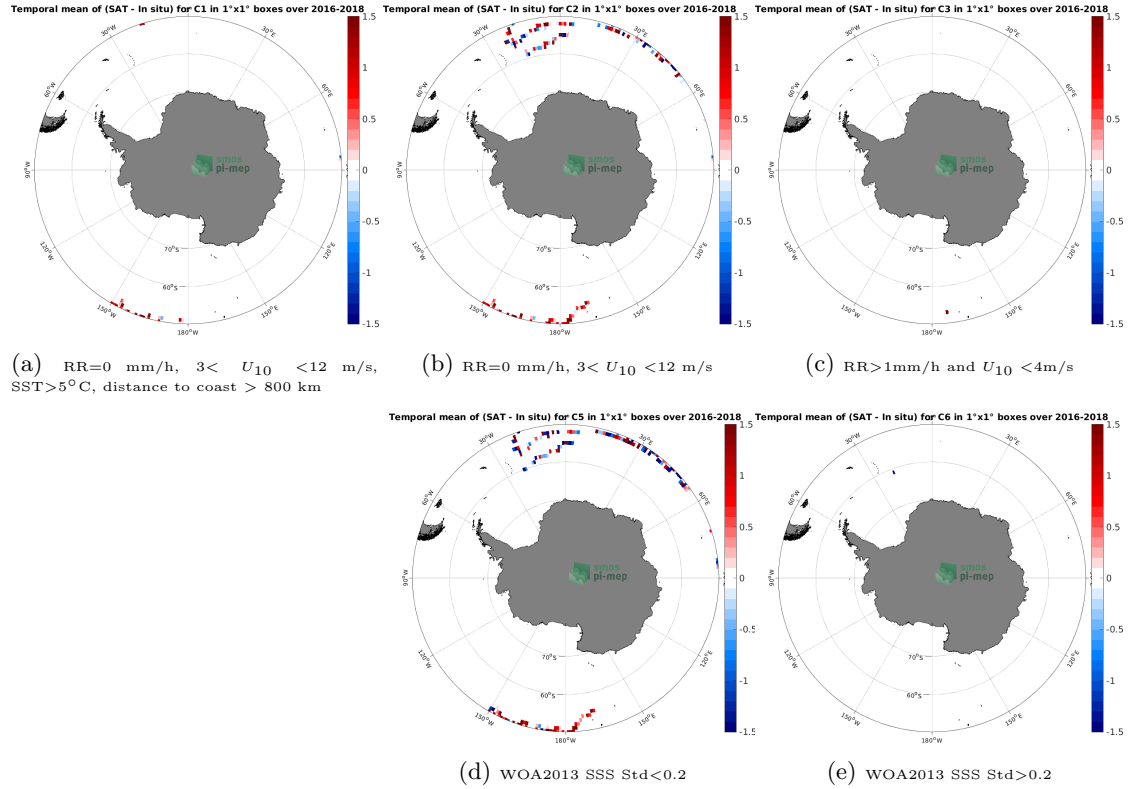
Figure 11: Temporal mean gridded over spatial boxes of size 1^{\circ}\times 1^{\circ} of \Delta\text{SSS} (SMOS SSS L2Q v331 - No FLAG (CMEMS-CATDS-CPDC) - Surface drifters) for 5 different subdatasets corresponding to: \text{RR}=0 mm/h, 3 < U_{10} < 12 m/s, \text{SST}>5^{\circ}\text{C} , distance to coast > 800 km (a), \text{RR}=0 mm/h, 3 < U_{10} < 12 m/s (b), \text{RR}>1 mm/h and U_{10} < 4 m/s (c), WOA2013 SSS Std < 0.2 (d), WOA2013 SSS Std > 0.2 (e).
