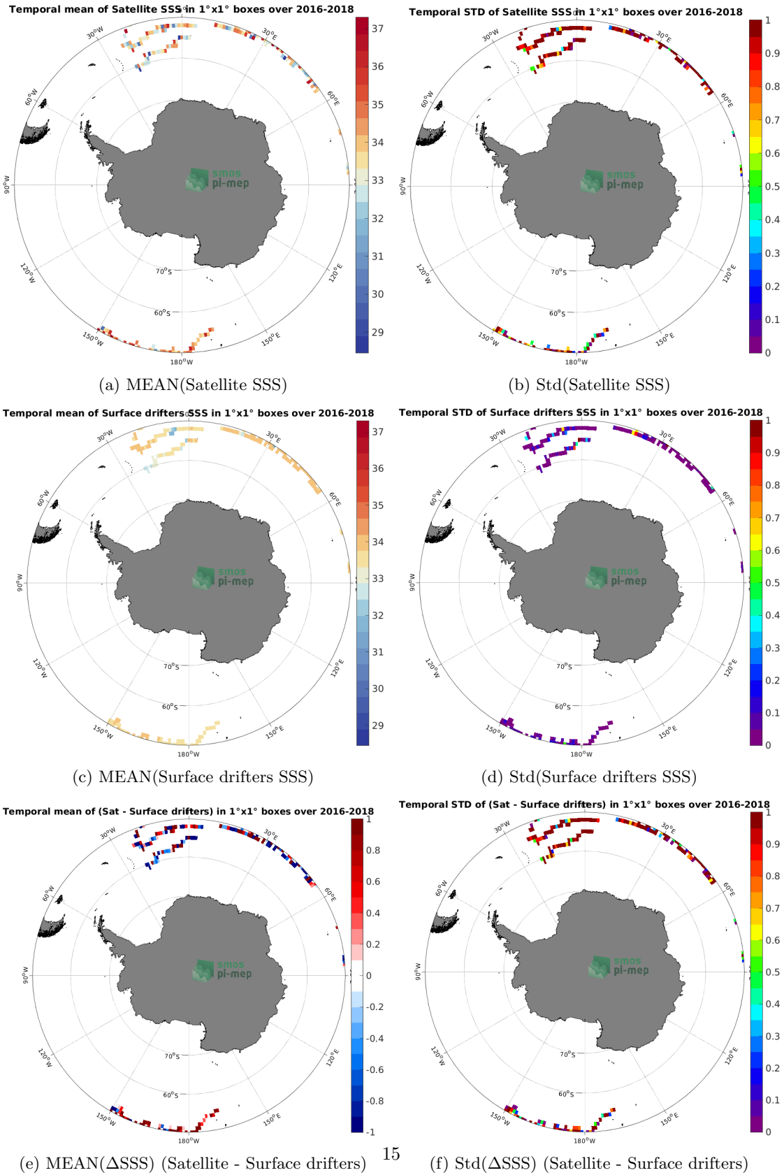
Figure 5: Temporal mean (left) and Std (right) of SSS from SMOS SSS L2Q v331 - No FLAG (CMEMS-CATDS-CPDC) (top), Surface drifters (middle), and of \Delta SSS (Satellite - Surface drifters). Only match-up pairs are used to generate these maps.
