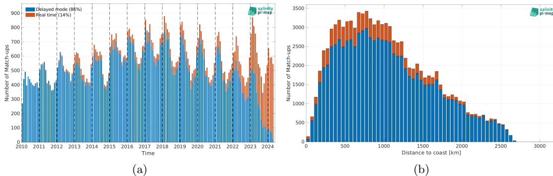
Figure 2: Number of match-ups between Argo and SMOS SSS L2Q v331 - No FLAG (CMEMS-CATDS-CPDC) SSS as a function of time (a) and as function of the distance to coast (b) over the Southern Ocean Pi-MEP region and for the full satellite product period.
