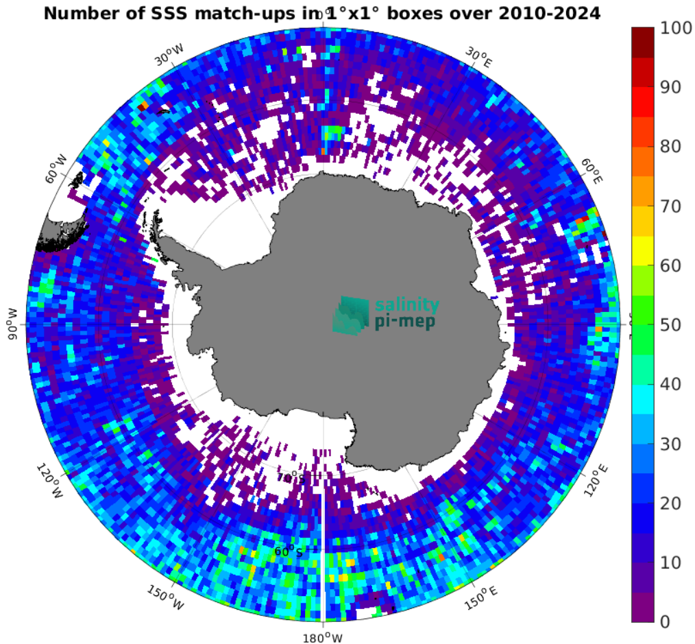
Figure 5: Number of SSS match-ups between Argo SSS and the SMOS SSS L2Q v331 - No FLAG (CMEMS-CATDS-CPDC) SSS product for the Southern Ocean Pi-MEP region over 1^\circ \times 1^\circ boxes and for the full satellite product period.
