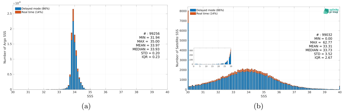
Figure 3: Histograms of SSS from Argo (a) and SMOS SSS L2Q v331 - No FLAG (CMEMS-CATDS-CPDC) (b) considering all match-up pairs per bins of 0.1 over the Southern Ocean Pi-MEP region and for the full satellite product period.
