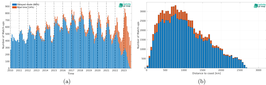
Figure 1: Number of match-ups between Argo and SMOS SSS L2Q v331 - No FLAG (CMEMS-CATDS-CPDC) SSS as a function of time (a) and as function of the distance to coast (b) over the Southern Ocean Pi-MEP region and for the full satellite product period.
