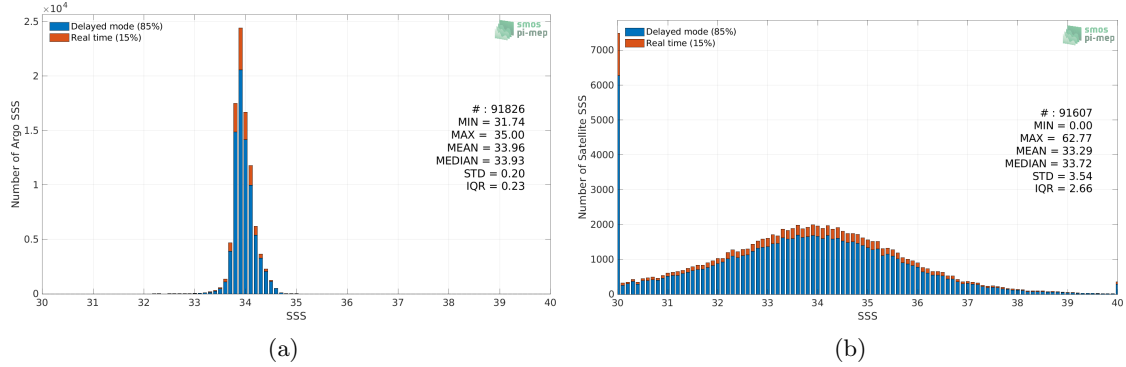
Figure 2: Histograms of SSS from Argo (a) and SMOS SSS L2Q v331 - No FLAG (CMEMS-CATDS-CPDC) (b) considering all match-up pairs per bins of 0.1 over the Southern Ocean Pi-MEP region and for the full satellite product period.
