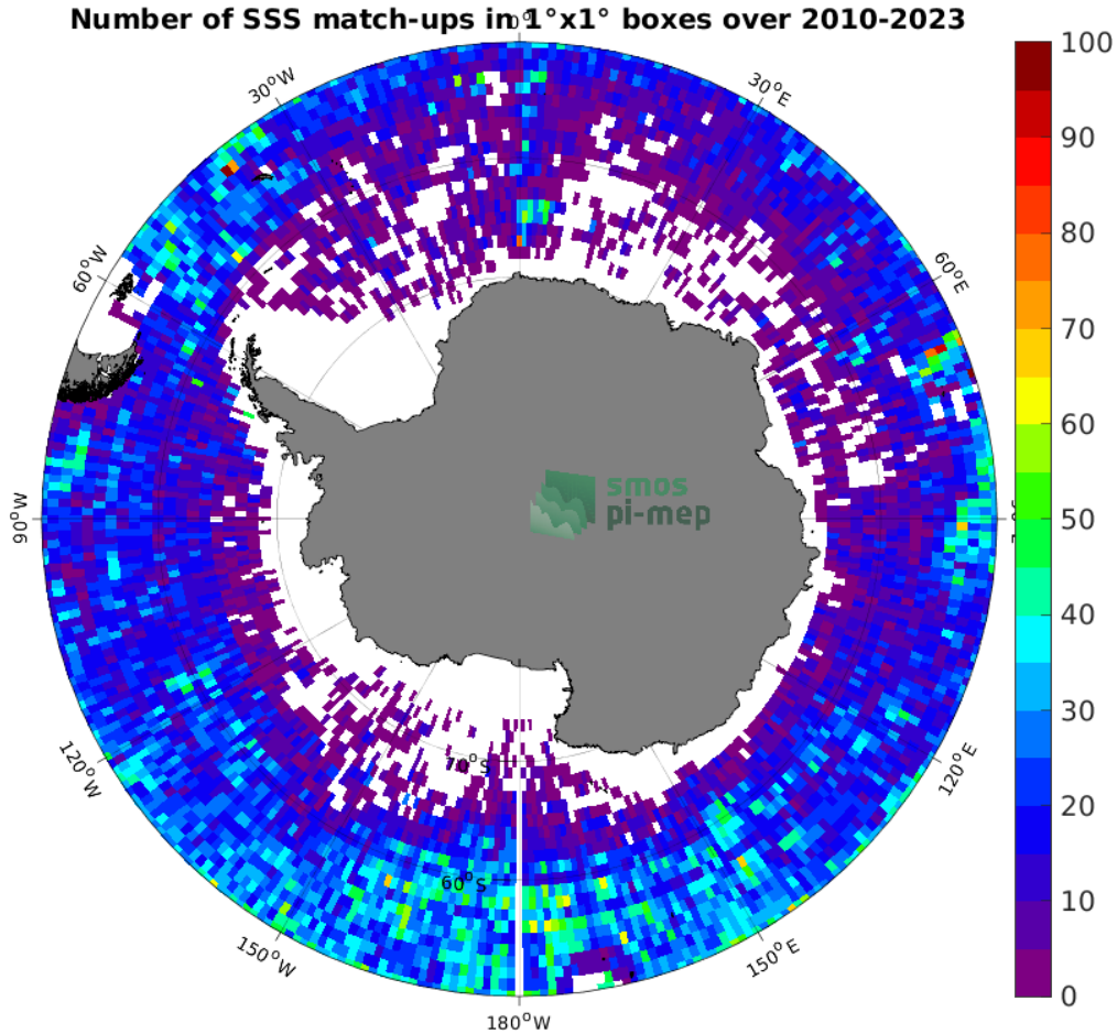
Figure 4: Number of SSS match-ups between Argo SSS and the SMOS SSS L2Q v331 - No FLAG (CMEMS-CATDS-CPDC) SSS product for the Southern Ocean Pi-MEP region over 1^\circ \times 1^\circ boxes and for the full satellite product period.
