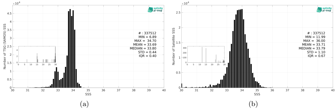
Figure 2: Histograms of SSS from TSG (SAMOS) (a) and SMOS SSS L3 v9 - 9 Days (CATDS-CEC-LOCEAN) (b) considering all match-up pairs per bins of 0.1 over the Southern Ocean Pi-MEP region and for the full satellite product period.
