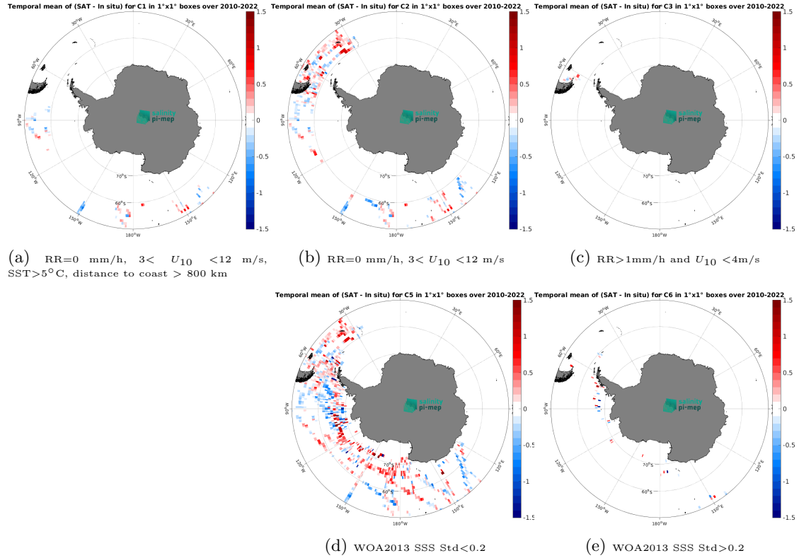
Figure 12: Temporal mean gridded over spatial boxes of size 1^{\circ}\times 1^{\circ} of \Delta\text{SSS} (SMOS SSS L3 v9 - 9 Days (CATDS-CEC-LOCEAN) - TSG (SAMOS)) for 5 different subdatasets corresponding to:RR=0 mm/h, 3 < U_{10} < 12 m/s, SST >5^{\circ}\text{C} , distance to coast > 800 km (a), RR=0 mm/h, 3 < U_{10} < 12 m/s (b), RR >1 mm/h and U_{10} < 4 m/s (c), WOA2013 SSS Std <0.2 (d), WOA2013 SSS Std >0.2 (e).
