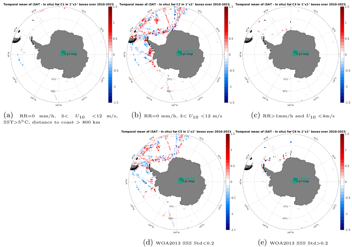
Figure 14: Temporal mean gridded over spatial boxes of size 1^\circ \times 1^\circ of \Delta\text{SSS} (SMOS SSS L3 v9 - 9 Days (CATDS-CEC-LOCEAN) - TSG (Polarstern)) for 5 different subdatasets corresponding to:RR=0 mm/h, 3 < U_{10} < 12 m/s, SST > 5^\circ\text{C} , distance to coast > 800 km (a), RR=0 mm/h, 3 < U_{10} < 12 m/s (b), RR > 1 mm/h and U_{10} < 4 m/s (c), WOA2013 SSS Std < 0.2 (d), WOA2013 SSS Std > 0.2 (e).
