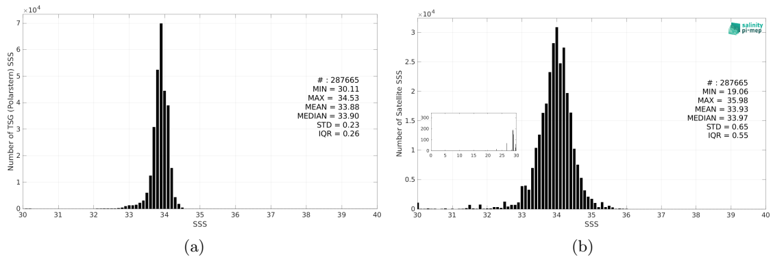
Figure 3: Histograms of SSS from TSG (Polarstern) (a) and SMOS SSS L3 v9 - 9 Days (CATDS-CEC-LOCEAN) (b) considering all match-up pairs per bins of 0.1 over the Southern Ocean Pi-MEP region and for the full satellite product period.
