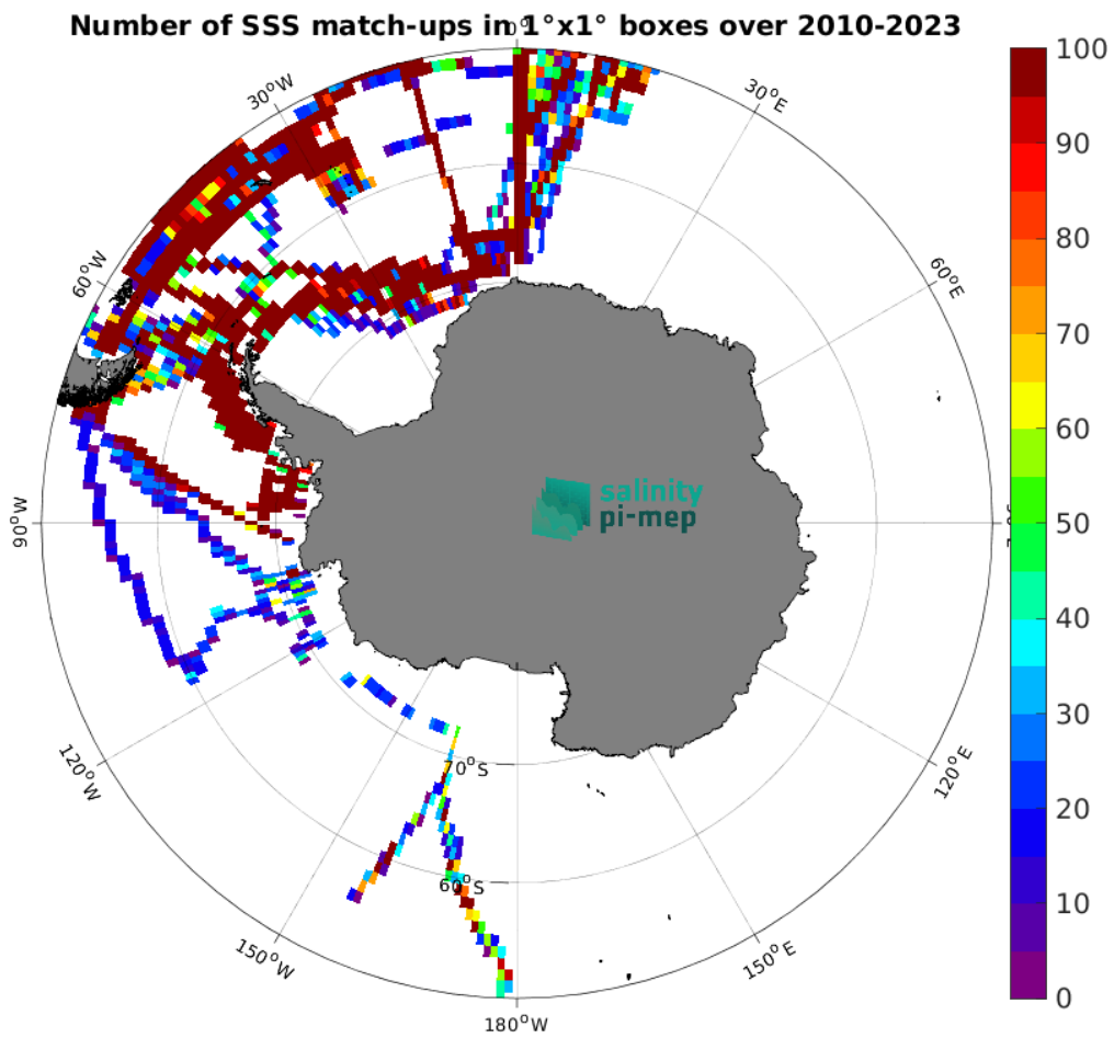
Figure 5: Number of SSS match-ups between TSG (Polarstern) SSS and the SMOS SSS L3 v9 - 9 Days (CATDS-CEC-LOCEAN) SSS product for the Southern Ocean Pi-MEP region over 1^\circ \times 1^\circ boxes and for the full satellite product period.
