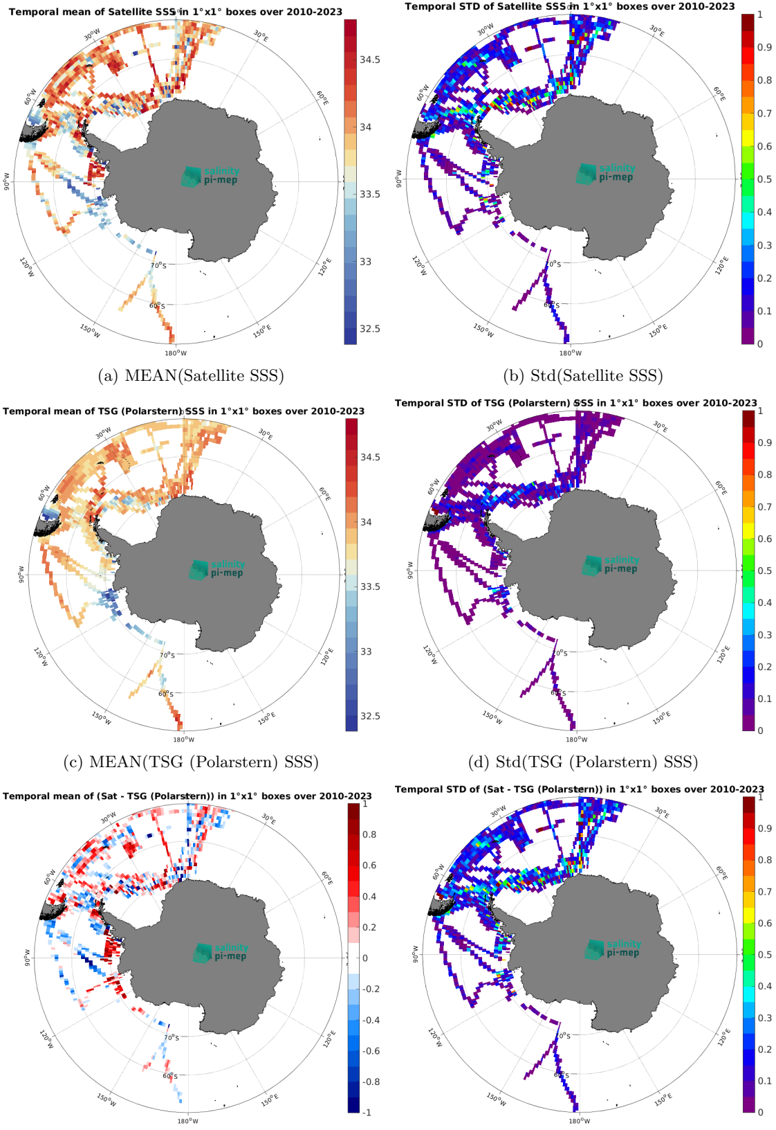
Figure 7: Temporal mean (left) and Std (right) of SSS from SMOS SSS L3 v9 - 9 Days (CATDS-CEC-LOCEAN) (top), TSG (Polarstern) (middle), and of \Delta SSS (Satellite - TSG (Polarstern)). Only match-up pairs are used to generate these maps.
