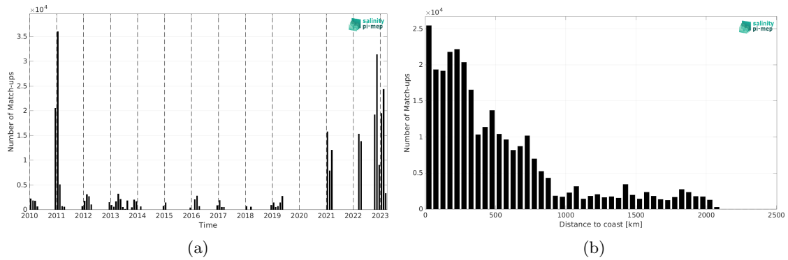
Figure 2: Number of match-ups between TSG (Polarstern) and SMOS SSS L3 v9 - 9 Days (CATDS-CEC-LOCEAN) SSS as a function of time (a) and as function of the distance to coast (b) over the Southern Ocean Pi-MEP region and for the full satellite product period.
