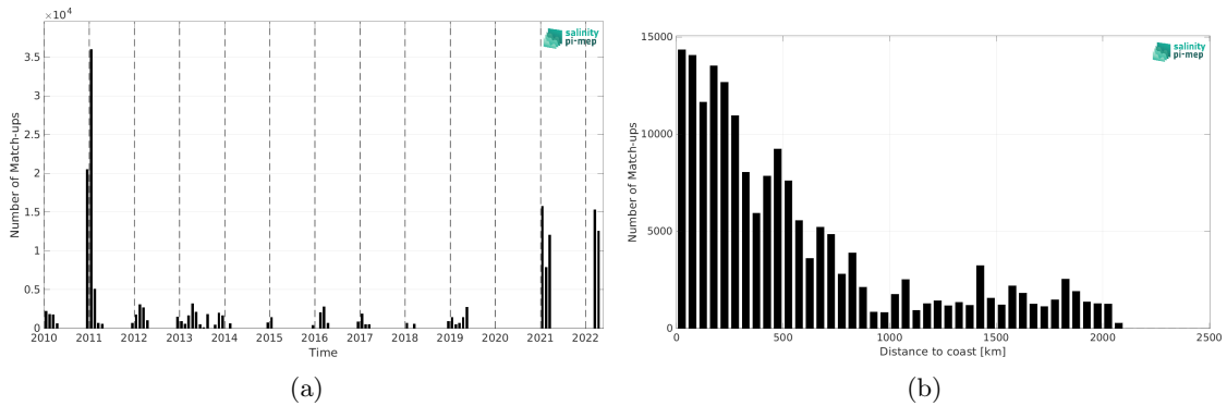
Figure 1: Number of match-ups between TSG (Polarstern) and SMOS SSS L3 v9 - 9 Days (CATDS-CEC-LOCEAN) SSS as a function of time (a) and as function of the distance to coast (b) over the Southern Ocean Pi-MEP region and for the full satellite product period.
