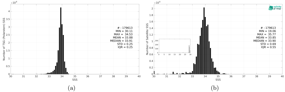
Figure 2: Histograms of SSS from TSG (Polarstern) (a) and SMOS SSS L3 v9 - 9 Days (CATDS-CEC-LOCEAN) (b) considering all match-up pairs per bins of 0.1 over the Southern Ocean Pi-MEP region and for the full satellite product period.
