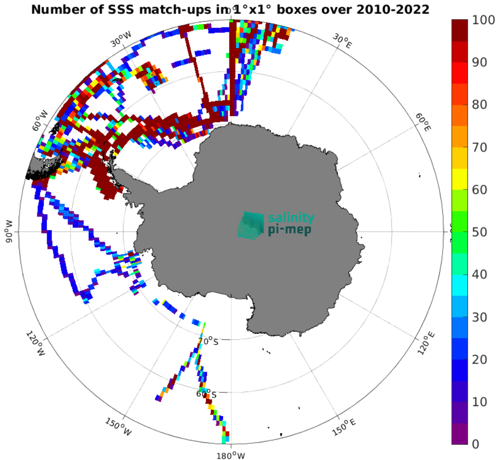
Figure 4: Number of SSS match-ups between TSG (Polarstern) SSS and the SMOS SSS L3 v9 - 9 Days (CATDS-CEC-LOCEAN) SSS product for the Southern Ocean Pi-MEP region over 1^\circ \times 1^\circ boxes and for the full satellite product period.
