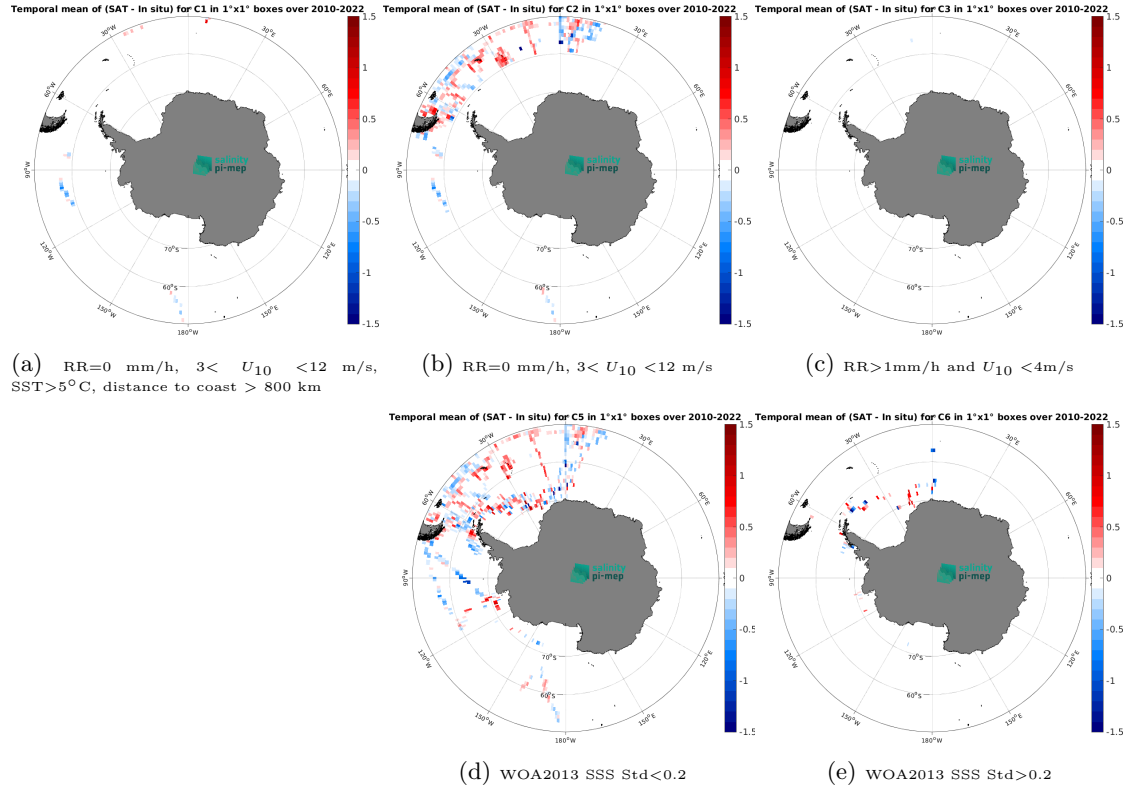
Figure 12: Temporal mean gridded over spatial boxes of size 1^{\circ}\times 1^{\circ} of \Delta\text{SSS} (SMOS SSS L3 v9 - 9 Days (CATDS-CEC-LOCEAN) - TSG (Polarstern)) for 5 different subdatasets corresponding to:RR=0 mm/h, 3 < U_{10} < 12 m/s, SST >5^{\circ}\text{C} , distance to coast > 800 km (a), RR=0 mm/h, 3 < U_{10} < 12 m/s (b), RR >1 mm/h and U_{10} < 4 m/s (c), WOA2013 SSS Std <0.2 (d), WOA2013 SSS Std >0.2 (e).
