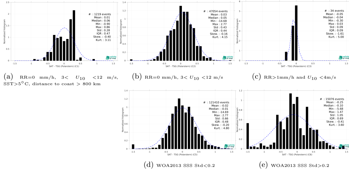
Figure 13: Normalized histogram of \Delta SSS (SMOS SSS L3 v9 - 9 Days (CATDS-CEC-LOCEAN) - TSG (Polarstern)) for 5 different subdatasets corresponding to: RR=0 mm/h, 3 < U_{10} < 12 m/s, SST > 5°C, distance to coast > 800 km (a), RR=0 mm/h, 3 < U_{10} < 12 m/s (b), RR > 1mm/h and U_{10} < 4 m/s (c), WOA2013 SSS Std < 0.2 (d), WOA2013 SSS Std > 0.2 (e).
