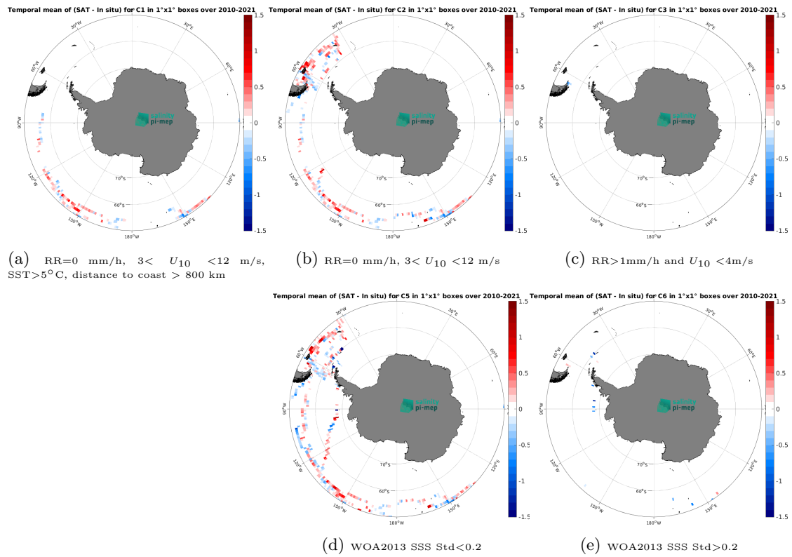
Figure 12: Temporal mean gridded over spatial boxes of size 1^\circ \times 1^\circ of \Delta\text{SSS} (SMOS SSS L3 v9 - 9 Days (CATDS-CEC-LOCEAN) - TSG (GOSUD-Sailing-ship)) for 5 different subdatasets corresponding to: RR=0 mm/h, 3 < U_{10} < 12 m/s, SST > 5^\circ\text{C} , distance to coast > 800 km (a), RR=0 mm/h, 3 < U_{10} < 12 m/s (b), RR > 1 mm/h and U_{10} < 4 m/s (c), WOA2013 SSS Std < 0.2 (d), WOA2013 SSS Std > 0.2 (e).
