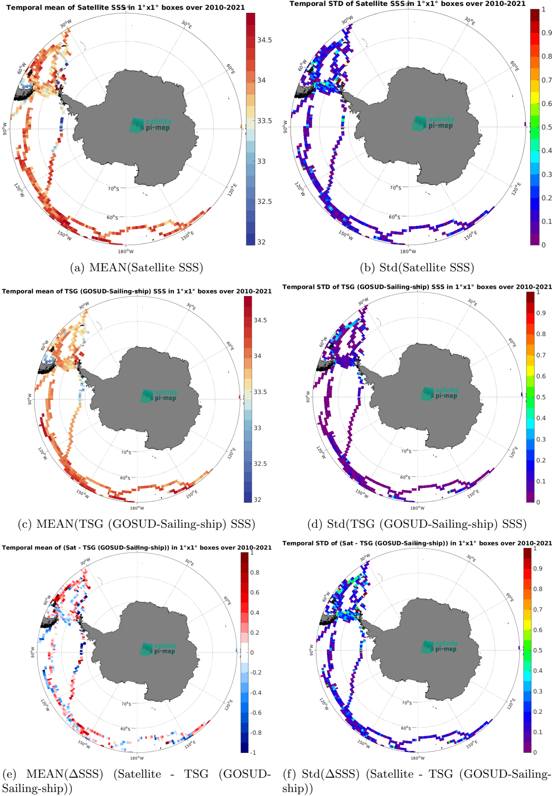
Figure 6: Temporal mean (left) and Std (right) of SSS from SMOS SSS L3 v9 - 9 Days (CATDS-CEC-LOCEAN) (top), TSG (GOSUD-Sailing-ship) (middle), and of \Delta SSS (Satellite - TSG (GOSUD-Sailing-ship)). Only match-up pairs are used to generate these maps.
