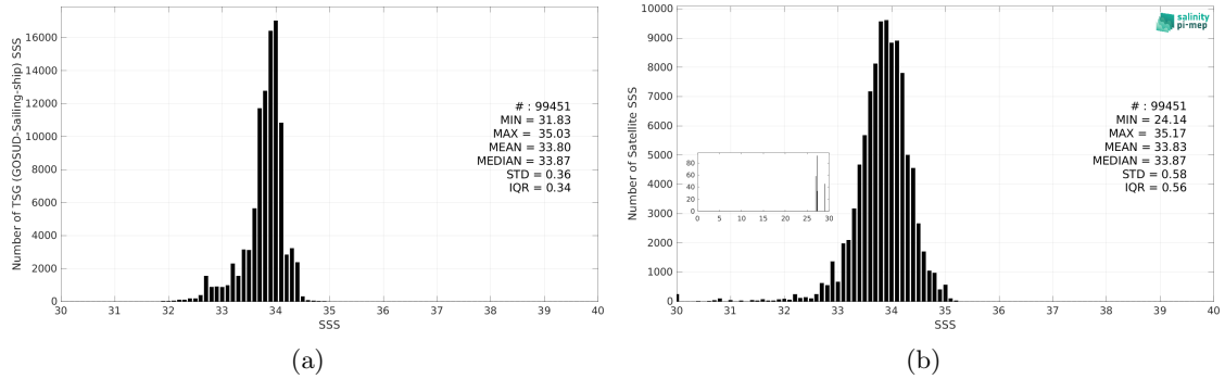
Figure 2: Histograms of SSS from TSG (GOSUD-Sailing-ship) (a) and SMOS SSS L3 v9 - 9 Days (CATDS-CEC-LOCEAN) (b) considering all match-up pairs per bins of 0.1 over the Southern Ocean Pi-MEP region and for the full satellite product period.
