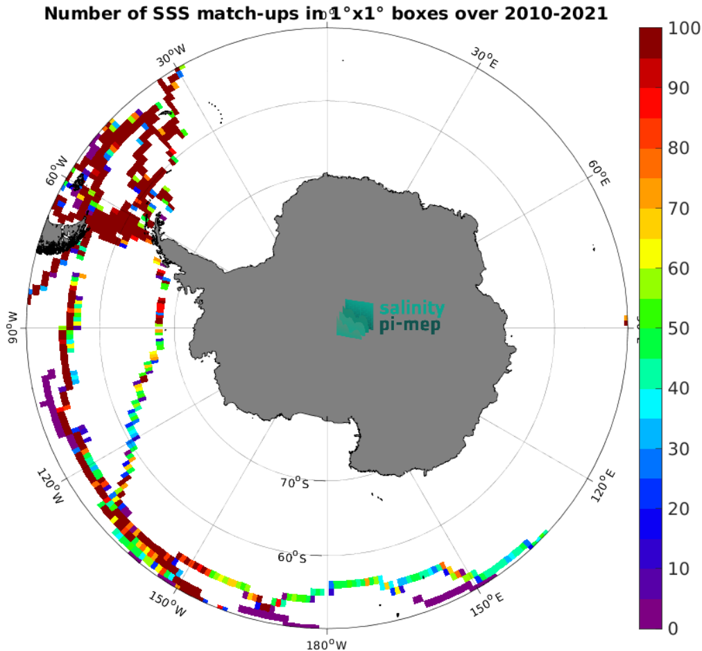
Figure 4: Number of SSS match-ups between TSG (GOSUD-Sailing-ship) SSS and the SMOS SSS L3 v9 - 9 Days (CATDS-CEC-LOCEAN) SSS product for the Southern Ocean Pi-MEP region over 1^\circ \times 1^\circ boxes and for the full satellite product period.
