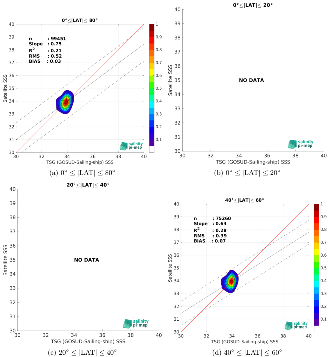
Figure 9: Contour maps of the concentration of SMOS SSS L3 v9 - 9 Days (CATDS-CEC-LOCEAN) SSS (y-axis) versus TSG (GOSUD-Sailing-ship) SSS (x-axis) at match-up pairs for different latitude bands. For each plot, the red line shows x=y . The black thin and dashed lines indicate a linear fit through the data cloud and the \pm 95\% confidence levels, respectively. The number of match-up pairs n , the slope and R^2 coefficient of the linear fit, the root mean square (RMS) and the mean bias between satellite and in situ data are indicated for each latitude band in each plot.
