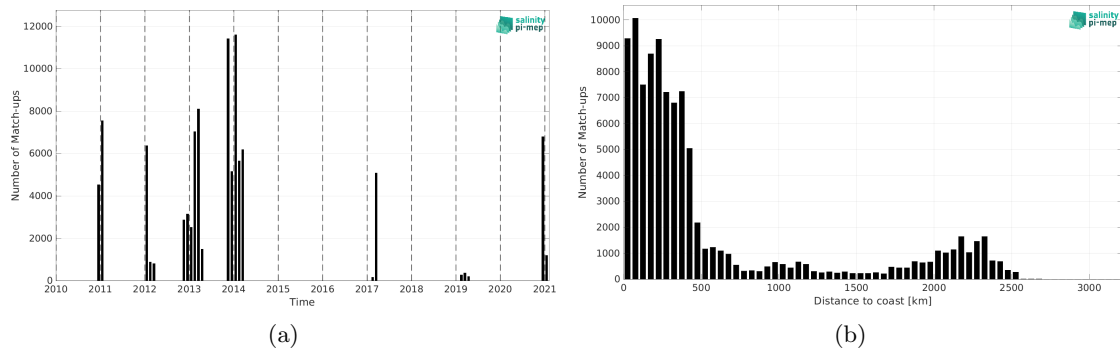
Figure 1: Number of match-ups between TSG (GOSUD-Sailing-ship) and SMOS SSS L3 v9 - 9 Days (CATDS-CEC-LOCEAN) SSS as a function of time (a) and as function of the distance to coast (b) over the Southern Ocean Pi-MEP region and for the full satellite product period.
