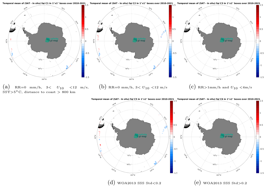
Figure 14: Temporal mean gridded over spatial boxes of size 1^\circ \times 1^\circ of \Delta\text{SSS} (SMOS SSS L3 v9 - 9 Days (CATDS-CEC-LOCEAN) - TSG (GOSUD-Research-vessel)) for 5 different subdatasets corresponding to:RR=0 mm/h, 3 < U_{10} < 12 m/s, SST >5^\circ\text{C} , distance to coast > 800 km (a), RR=0 mm/h, 3 < U_{10} < 12 m/s (b), RR >1 mm/h and U_{10} < 4 m/s (c), WOA2013 SSS Std <0.2 (d), WOA2013 SSS Std >0.2 (e).
