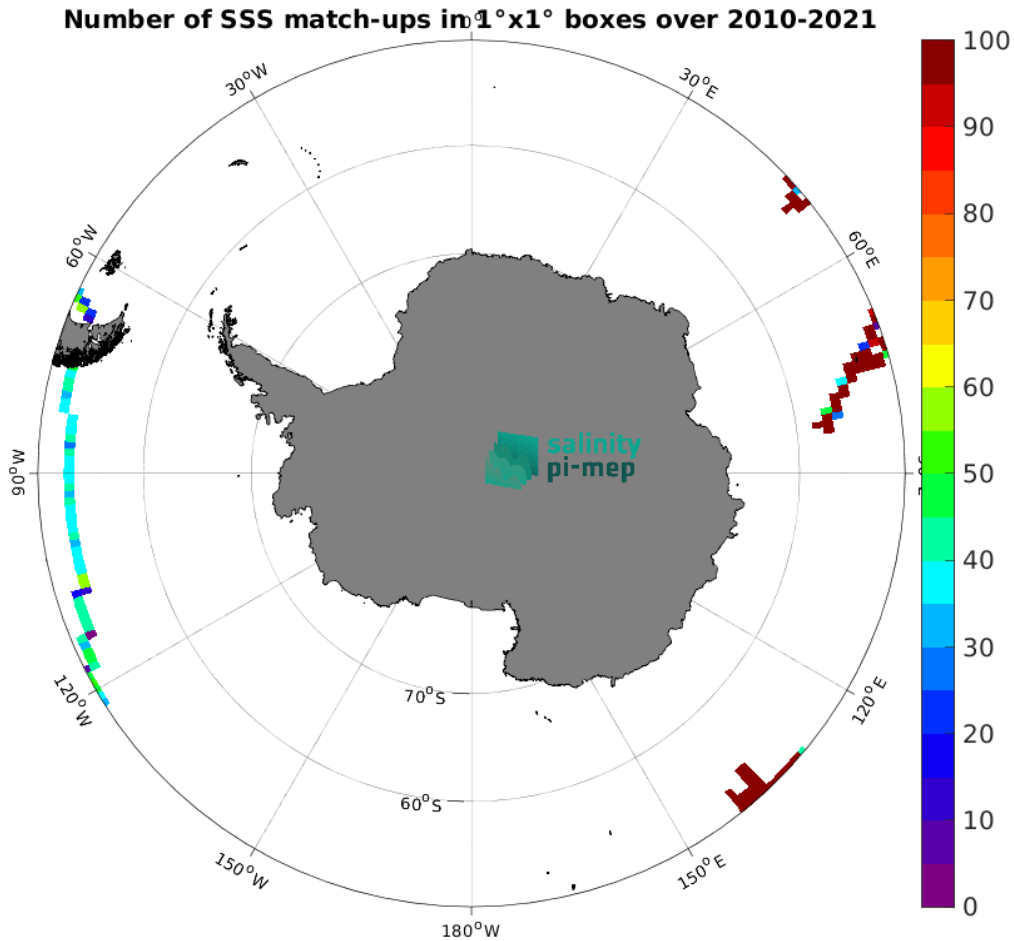
Figure 5: Number of SSS match-ups between TSG (GOSUD-Research-vessel) SSS and the SMOS SSS L3 v9 - 9 Days (CATDS-CEC-LOCEAN) SSS product for the Southern Ocean Pi-MEP region over 1^\circ \times 1^\circ boxes and for the full satellite product period.
