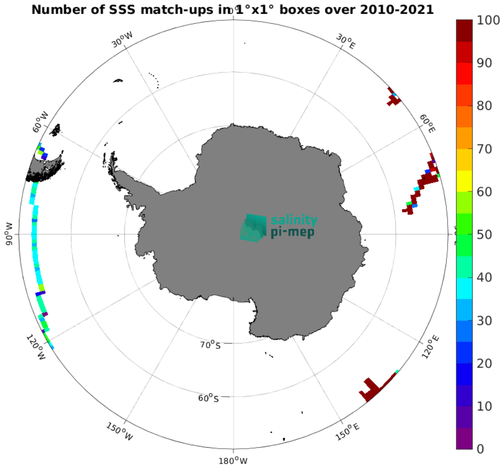
Figure 5: Number of SSS match-ups between TSG (GOSUD-Research-vessel) SSS and the SMOS SSS L3 v9 - 9 Days (CATDS-CEC-LOCEAN) SSS product for the Southern Ocean Pi-MEP region over 1^\circ \times 1^\circ boxes and for the full satellite product period.
