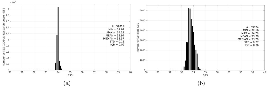
Figure 3: Histograms of SSS from TSG (GOSUD-Research-vessel) (a) and SMOS SSS L3 v9 - 9 Days (CATDS-CEC-LOCEAN) (b) considering all match-up pairs per bins of 0.1 over the Southern Ocean Pi-MEP region and for the full satellite product period.
