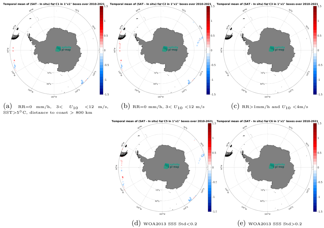
Figure 12: Temporal mean gridded over spatial boxes of size 1^\circ \times 1^\circ of \Delta\text{SSS} (SMOS SSS L3 v9 - 9 Days (CATDS-CEC-LOCEAN) - TSG (GOSUD-Research-vessel)) for 5 different subdatasets corresponding to: RR=0 mm/h, 3 < U_{10} < 12 m/s, SST > 5^\circ\text{C} , distance to coast > 800 km (a), RR=0 mm/h, 3 < U_{10} < 12 m/s (b), RR > 1 mm/h and U_{10} < 4 m/s (c), WOA2013 SSS Std < 0.2 (d), WOA2013 SSS Std > 0.2 (e).
