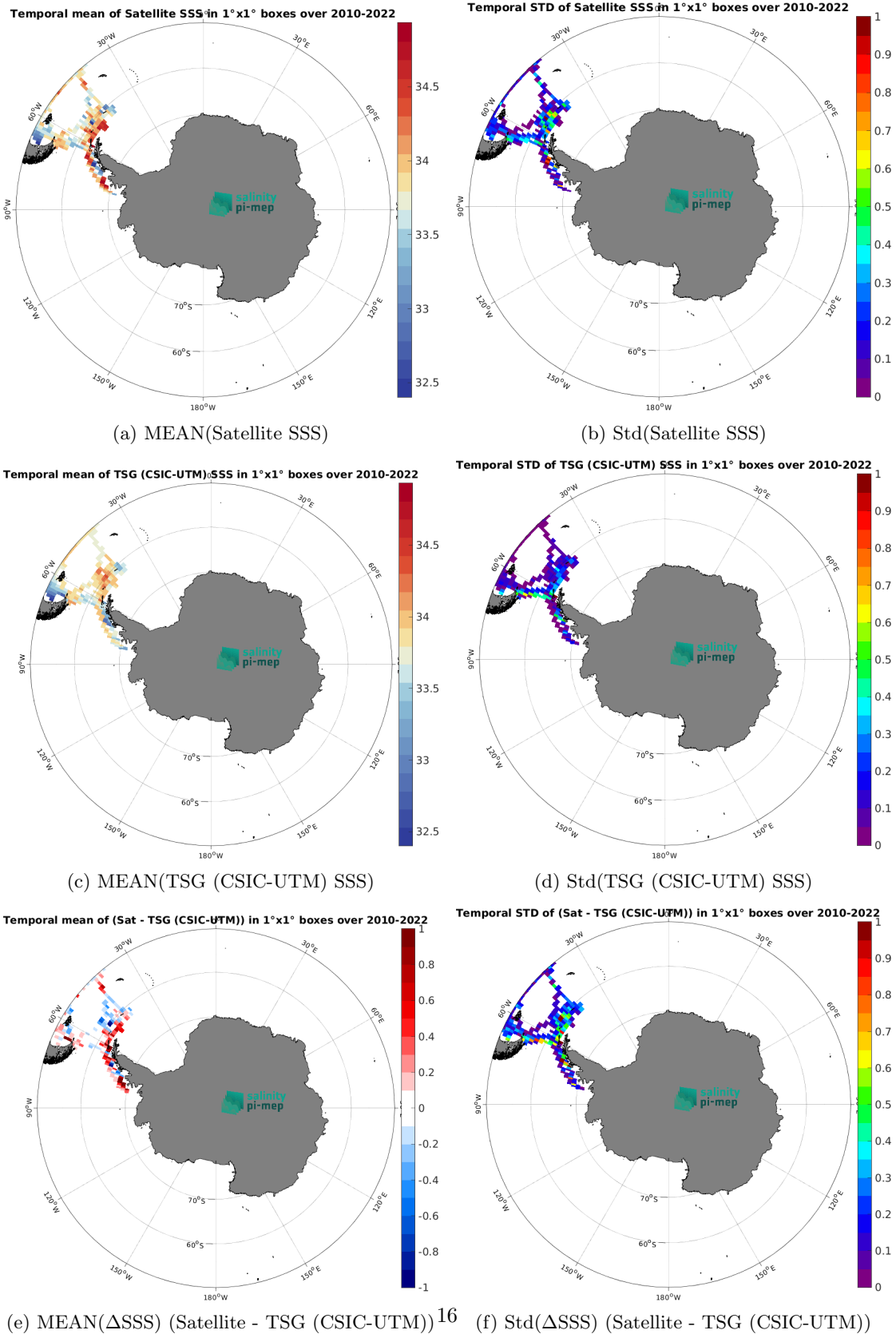
Figure 7: Temporal mean (left) and Std (right) of SSS from SMOS SSS L3 v9 - 9 Days (CATDS-CEC-LOCEAN) (top), TSG (CSIC-UTM) (middle), and of \Delta SSS (Satellite - TSG (CSIC-UTM)). Only match-up pairs are used to generate these maps.
