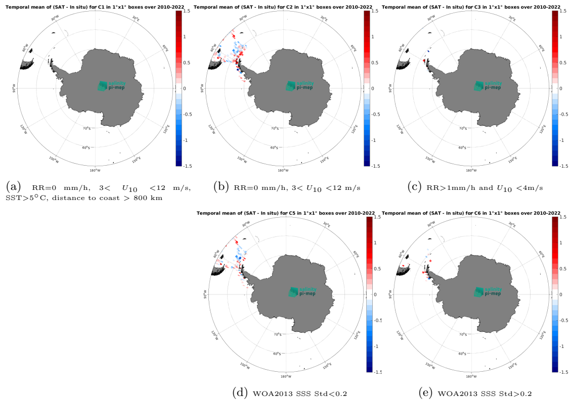
Figure 14: Temporal mean gridded over spatial boxes of size 1^\circ \times 1^\circ of \Delta\text{SSS} (SMOS SSS L3 v9 - 9 Days (CATDS-CEC-LOCEAN) - TSG (CSIC-UTM)) for 5 different subdatasets corresponding to:RR=0 mm/h, 3 < U_{10} < 12 m/s, SST >5^\circ\text{C} , distance to coast > 800 km (a), RR=0 mm/h, 3 < U_{10} < 12 m/s (b), RR >1 mm/h and U_{10} < 4 m/s (c), WOA2013 SSS Std <0.2 (d), WOA2013 SSS Std >0.2 (e).
