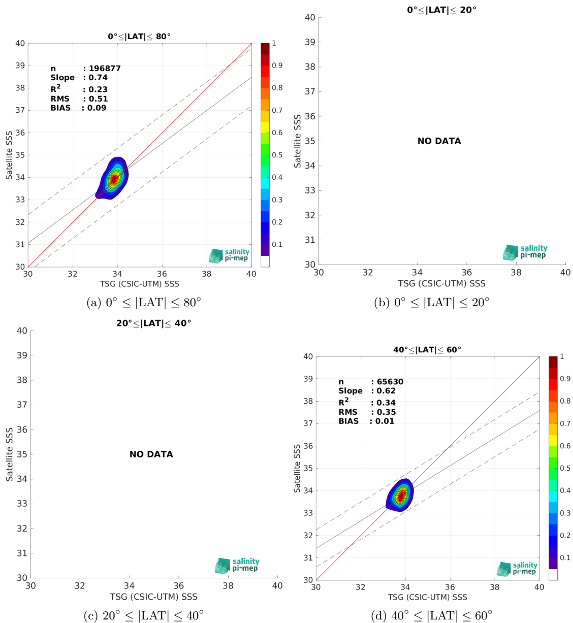
Figure 9: Contour maps of the concentration of SMOS SSS L3 v9 - 9 Days (CATDS-CEC-LOCEAN) SSS (y-axis) versus TSG (CSIC-UTM) SSS (x-axis) at match-up pairs for different latitude bands. For each plot, the red line shows x=y . The black thin and dashed lines indicate a linear fit through the data cloud and the \pm 95\% confidence levels, respectively. The number match-up pairs n , the slope and R^2 coefficient of the linear fit, the root mean square (RMS) and the mean bias between satellite and in situ data are indicated for each latitude band in each plots.
