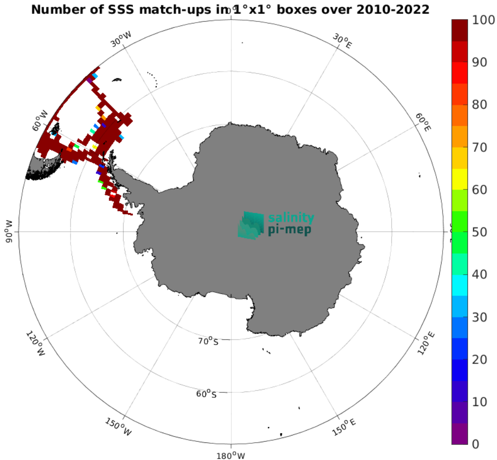
Figure 4: Number of SSS match-ups between TSG (CSIC-UTM) SSS and the SMOS SSS L3 v9 - 9 Days (CATDS-CEC-LOCEAN) SSS product for the Southern Ocean Pi-MEP region over 1^\circ \times 1^\circ boxes and for the full satellite product period.
