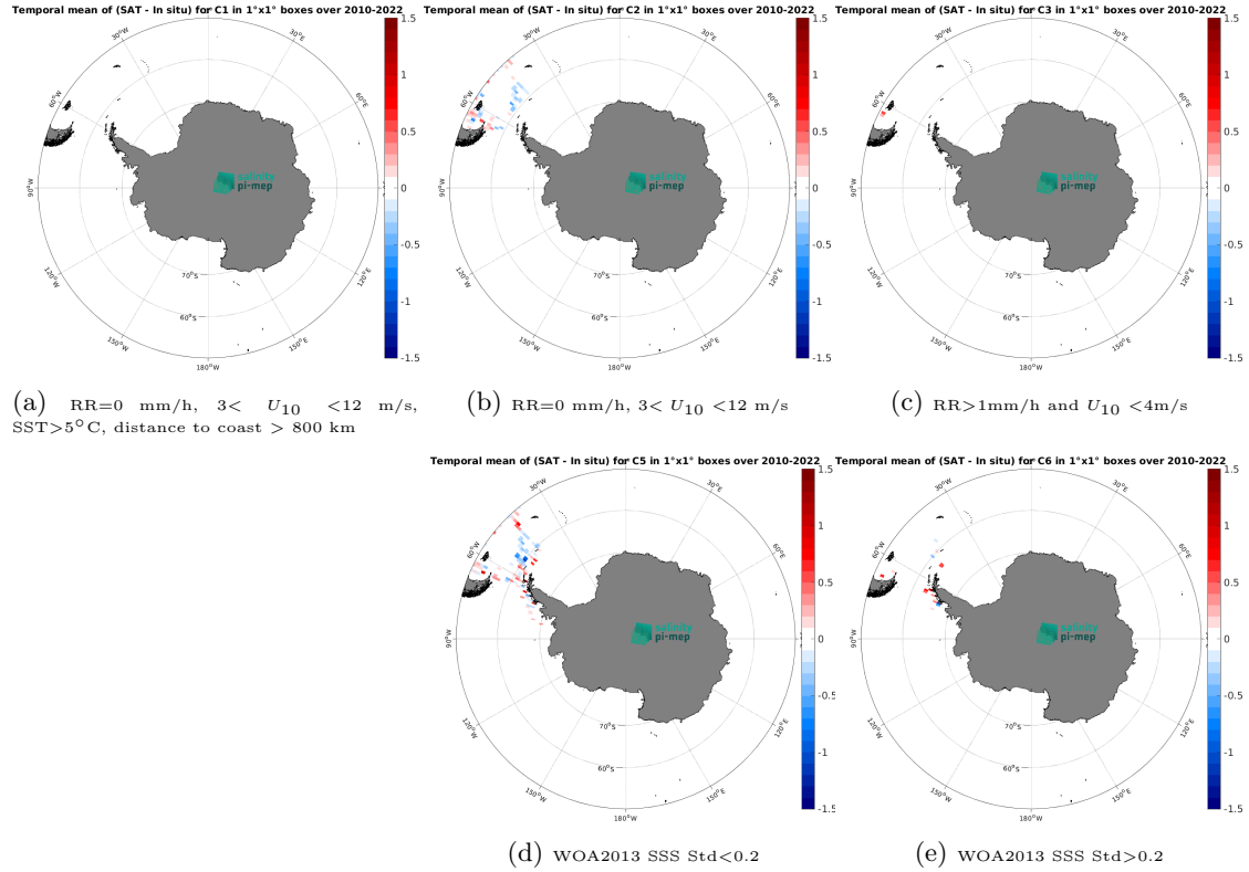
Figure 12: Temporal mean gridded over spatial boxes of size 1^{\circ}\times 1^{\circ} of \Delta\text{SSS} (SMOS SSS L3 v9 - 9 Days (CATDS-CEC-LOCEAN) - TSG (CSIC-UTM)) for 5 different subdatasets corresponding to:RR=0 mm/h, 3 < U_{10} < 12 m/s, SST >5^{\circ}\text{C} , distance to coast > 800 km (a), RR=0 mm/h, 3 < U_{10} < 12 m/s (b), RR >1 mm/h and U_{10} < 4 m/s (c), WOA2013 SSS Std <0.2 (d), WOA2013 SSS Std >0.2 (e).
