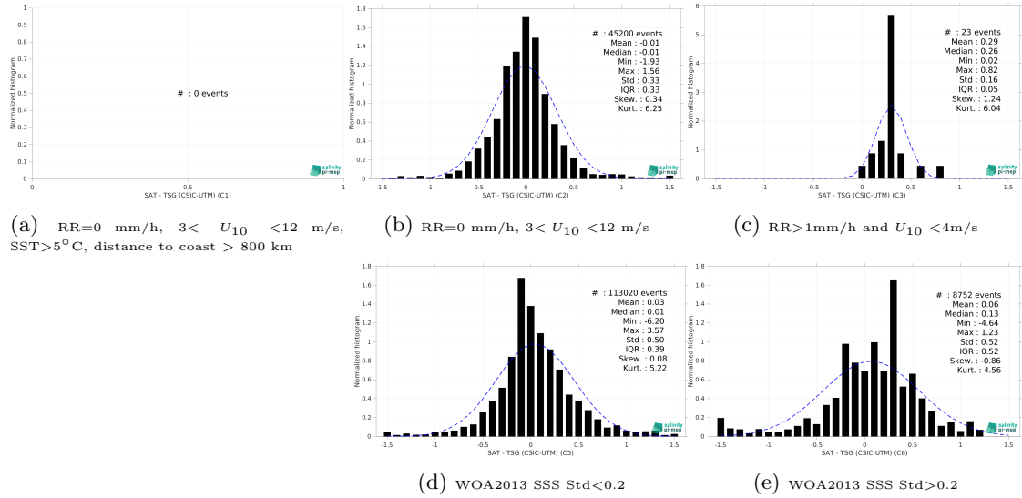
Figure 13: Normalized histogram of \Delta\text{SSS} (SMOS SSS L3 v9 - 9 Days (CATDS-CEC-LOCEAN) - TSG (CSIC-UTM)) for 5 different subdatasets corresponding to: \text{RR}=0 mm/h, 3 < U_{10} < 12 m/s, \text{SST} > 5^\circ\text{C} , distance to coast > 800 km (a), \text{RR}=0 mm/h, 3 < U_{10} < 12 m/s (b), \text{RR} > 1 mm/h and U_{10} < 4 m/s (c), WOA2013 SSS Std < 0.2 (d), WOA2013 SSS Std > 0.2 (e).
