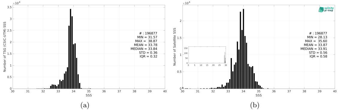
Figure 2: Histograms of SSS from TSG (CSIC-UTM) (a) and SMOS SSS L3 v9 - 9 Days (CATDS-CEC-LOCEAN) (b) considering all match-up pairs per bins of 0.1 over the Southern Ocean Pi-MEP region and for the full satellite product period.
