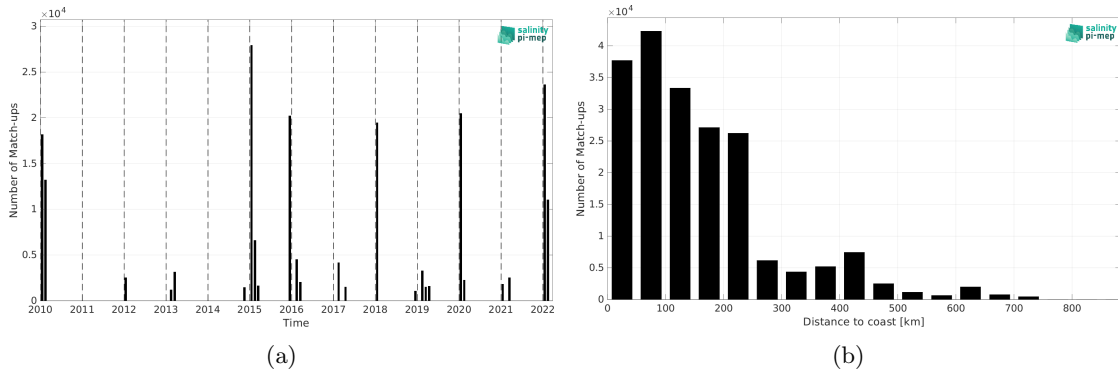
Figure 1: Number of match-ups between TSG (CSIC-UTM) and SMOS SSS L3 v9 - 9 Days (CATDS-CEC-LOCEAN) SSS as a function of time (a) and as function of the distance to coast (b) over the Southern Ocean Pi-MEP region and for the full satellite product period.
