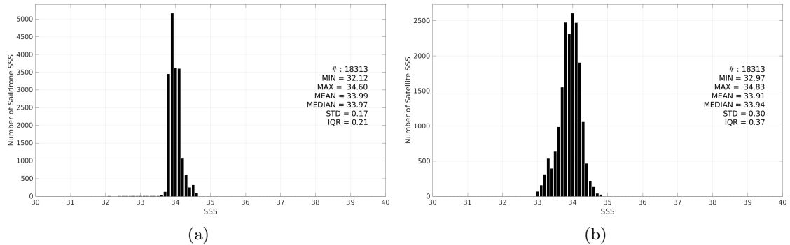
Figure 3: Histograms of SSS from Sairdrone (a) and SMOS SSS L3 v9 - 9 Days (CATDS-CEC-LOCEAN) (b) considering all match-up pairs per bins of 0.1 over the Southern Ocean Pi-MEP region and for the full satellite product period.
