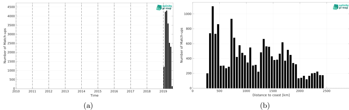
Figure 2: Number of match-ups between Saildrone and SMOS SSS L3 v9 - 9 Days (CATDS-CEC-LOCEAN) SSS as a function of time (a) and as function of the distance to coast (b) over the Southern Ocean Pi-MEP region and for the full satellite product period.
