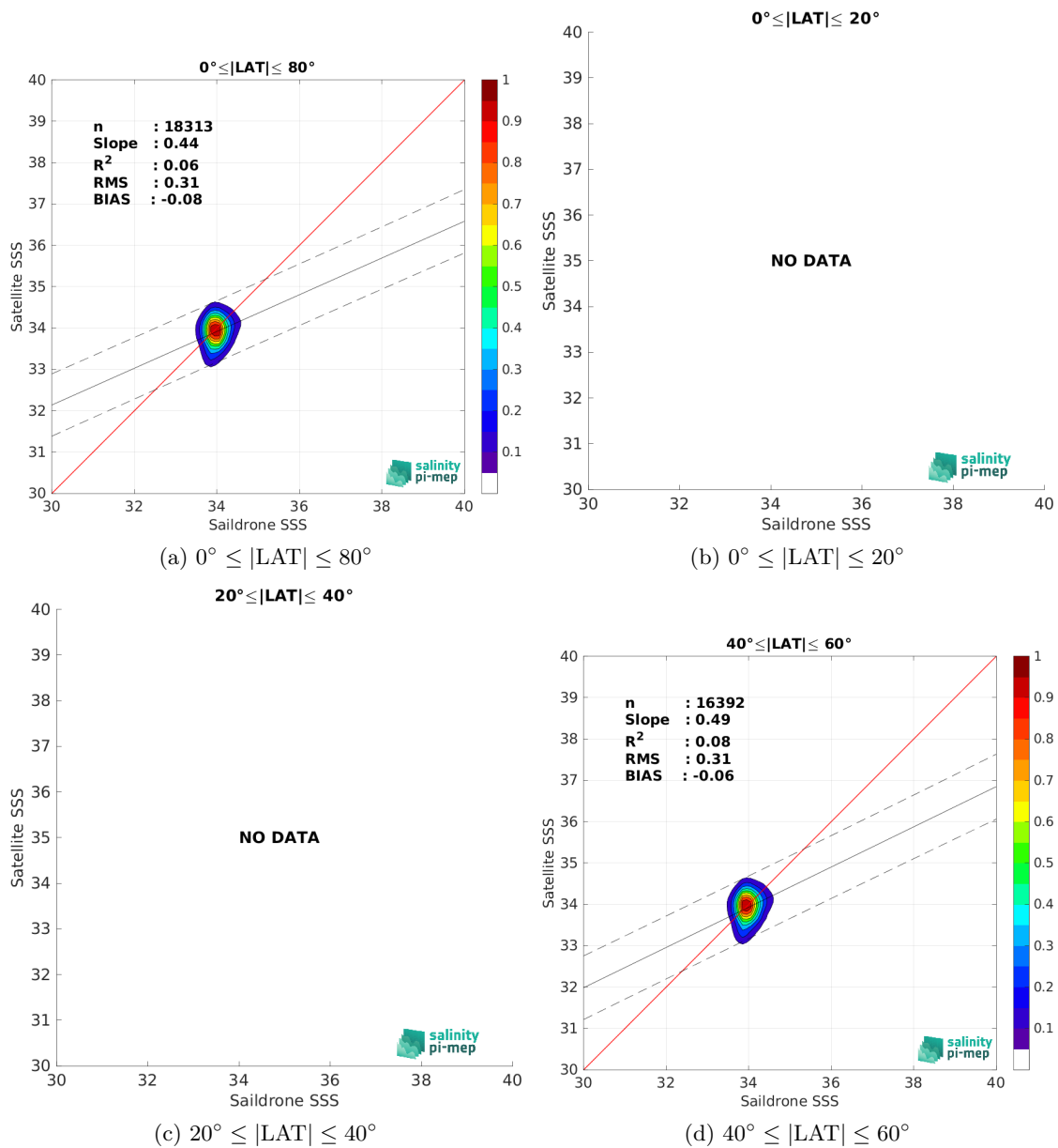
Figure 10: Contour maps of the concentration of SMOS SSS L3 v9 - 9 Days (CATDS-CEC-LOCEAN) SSS (y-axis) versus Sairdron SSS (x-axis) at match-up pairs for different latitude bands. For each plot, the red line shows x=y . The black thin and dashed lines indicate a linear fit through the data cloud and the \pm 95\% confidence levels, respectively. The number match-up pairs n , the slope and R^2 coefficient of the linear fit, the root mean square (RMS) and the mean bias between satellite and in situ data are indicated for each latitude band in each plots.
