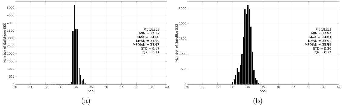
Figure 2: Histograms of SSS from Sairdrone (a) and SMOS SSS L3 v9 - 9 Days (CATDS-CEC-LOCEAN) (b) considering all match-up pairs per bins of 0.1 over the Southern Ocean Pi-MEP region and for the full satellite product period.
