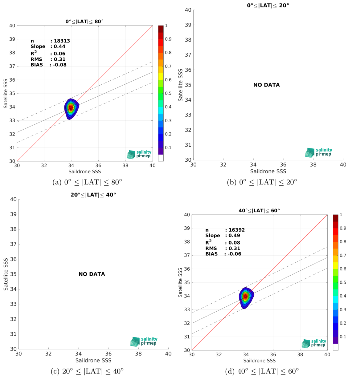
Figure 9: Contour maps of the concentration of SMOS SSS L3 v9 - 9 Days (CATDS-CEC-LOCEAN) SSS (y-axis) versus Saildrone SSS (x-axis) at match-up pairs for different latitude bands. For each plot, the red line shows x=y . The black thin and dashed lines indicate a linear fit through the data cloud and the \pm 95\% confidence levels, respectively. The number match-up pairs n , the slope and R^2 coefficient of the linear fit, the root mean square (RMS) and the mean bias between satellite and in situ data are indicated for each latitude band in each plots.
