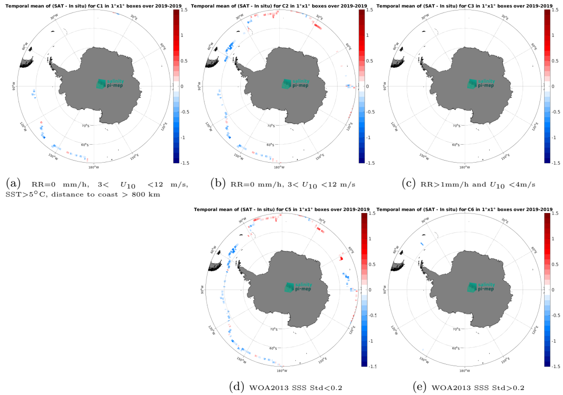
Figure 12: Temporal mean gridded over spatial boxes of size 1^{\circ}\times 1^{\circ} of \Delta\text{SSS} (SMOS SSS L3 v9 - 9 Days (CATDS-CEC-LOCEAN) - Saildrone) for 5 different subdatasets corresponding to:RR=0 mm/h, 3 < U_{10} < 12 m/s, SST >5^{\circ}\text{C} , distance to coast > 800 km (a), RR=0 mm/h, 3 < U_{10} < 12 m/s (b), RR >1 mm/h and U_{10} < 4 m/s (c), WOA2013 SSS Std <0.2 (d), WOA2013 SSS Std >0.2 (e).
