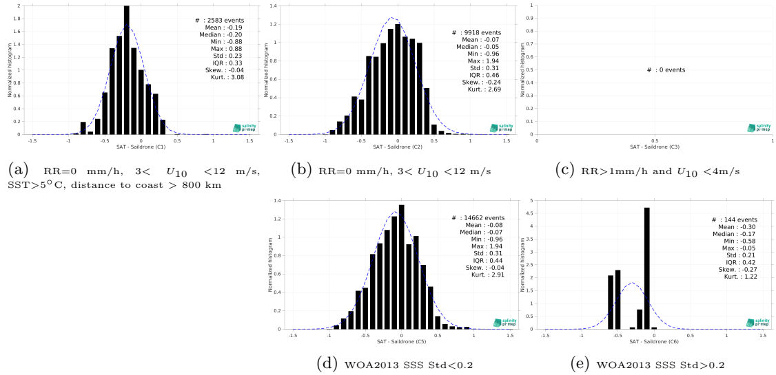
Figure 13: Normalized histogram of \Delta SSS (SMOS SSS L3 v9 - 9 Days (CATDS-CEC-LOCEAN) - Saildrone) for 5 different subdatasets corresponding to: RR=0 mm/h, 3 < U_{10} < 12 m/s, SST > 5°C, distance to coast > 800 km (a), RR=0 mm/h, 3 < U_{10} < 12 m/s (b), RR > 1mm/h and U_{10} < 4 m/s (c), WOA2013 SSS Std < 0.2 (d), WOA2013 SSS Std > 0.2 (e).
