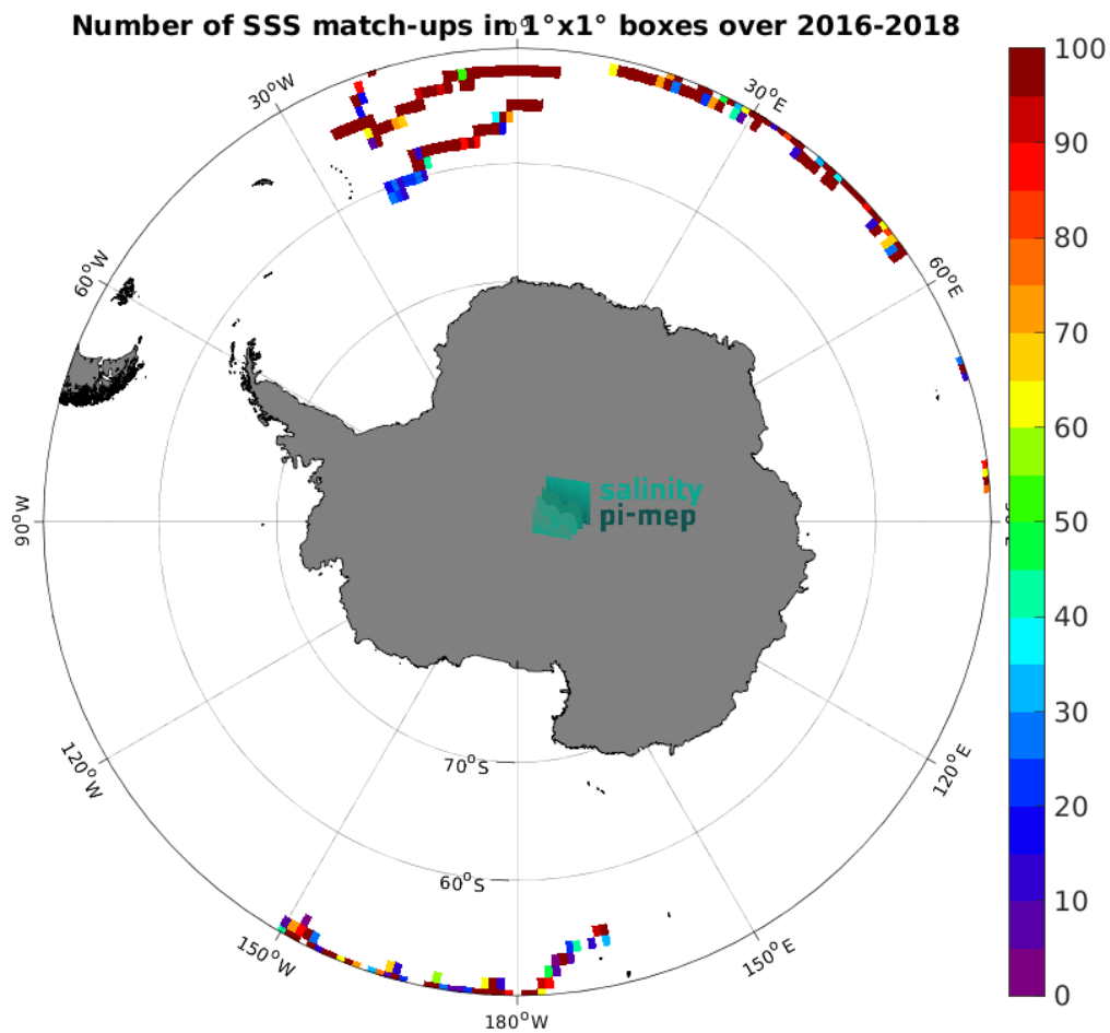
Figure 4: Number of SSS match-ups between Surface drifters SSS and the SMOS SSS L3 v9 - 9 Days (CATDS-CEC-LOCEAN) SSS product for the Southern Ocean Pi-MEP region over 1^\circ \times 1^\circ boxes and for the full satellite product period.
