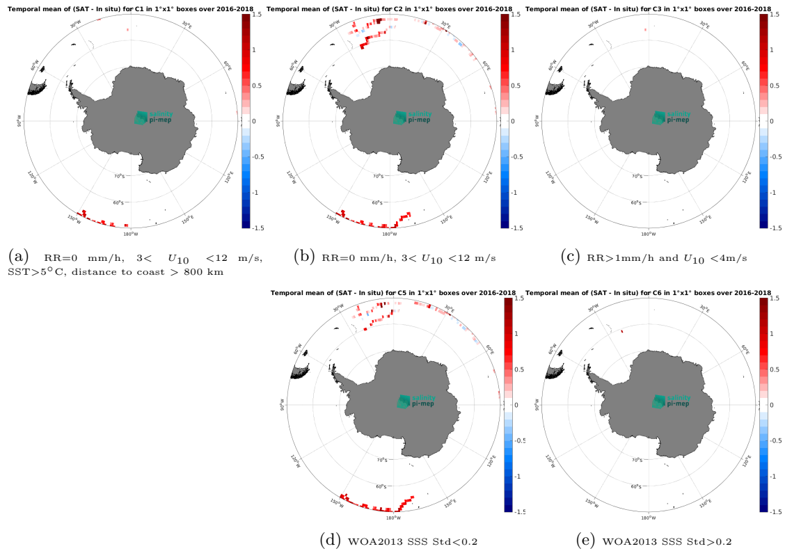
Figure 13: Temporal mean gridded over spatial boxes of size 1^\circ \times 1^\circ of \Delta SSS (SMOS SSS L3 v9 - 9 Days (CATDS-CEC-LOCEAN) - Surface drifters) for 5 different subdatasets corresponding to: RR=0 mm/h, 3 < U_{10} < 12 m/s, SST >5^\circ C, distance to coast > 800 km (a), RR=0 mm/h, 3 < U_{10} < 12 m/s (b), RR >1 mm/h and U_{10} < 4 m/s (c), WOA2013 SSS Std <0.2 (d), WOA2013 SSS Std >0.2 (e).
