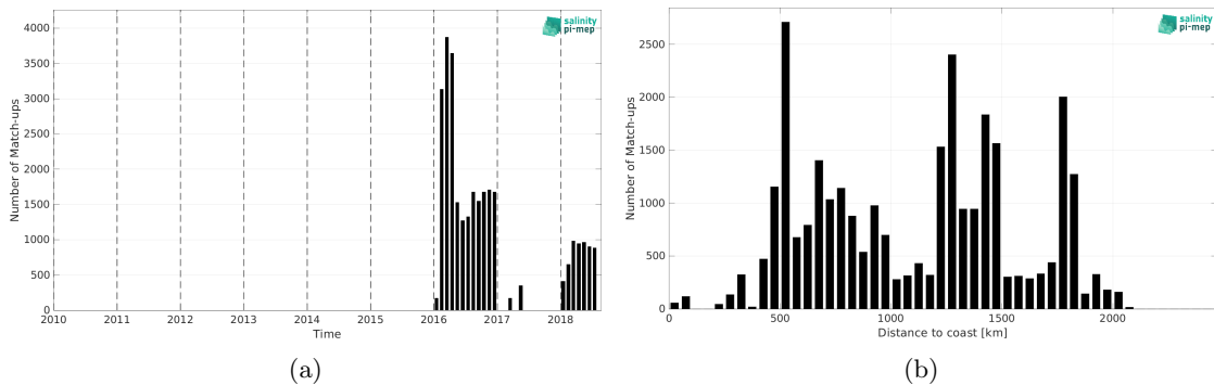
Figure 1: Number of match-ups between Surface drifters and SMOS SSS L3 v9 - 9 Days (CATDS-CEC-LOCEAN) SSS as a function of time (a) and as function of the distance to coast (b) over the Southern Ocean Pi-MEP region and for the full satellite product period.
