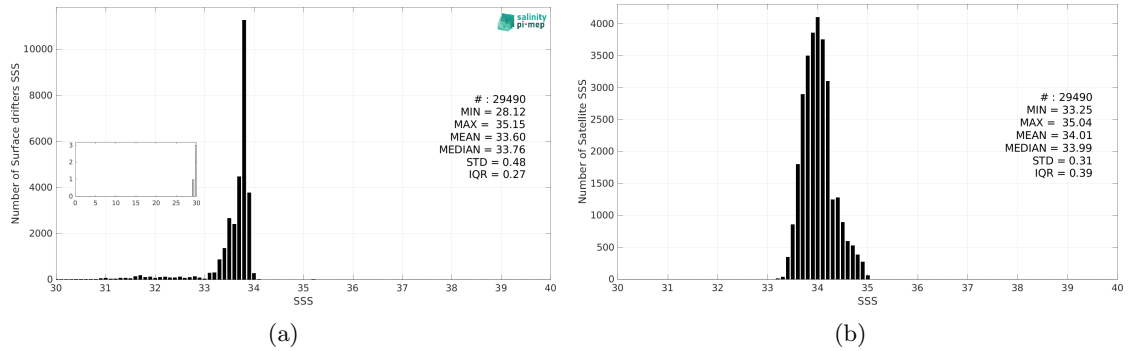
Figure 2: Histograms of SSS from Surface drifters (a) and SMOS SSS L3 v9 - 9 Days (CATDS-CEC-LOCEAN) (b) considering all match-up pairs per bins of 0.1 over the Southern Ocean Pi-MEP region and for the full satellite product period.
