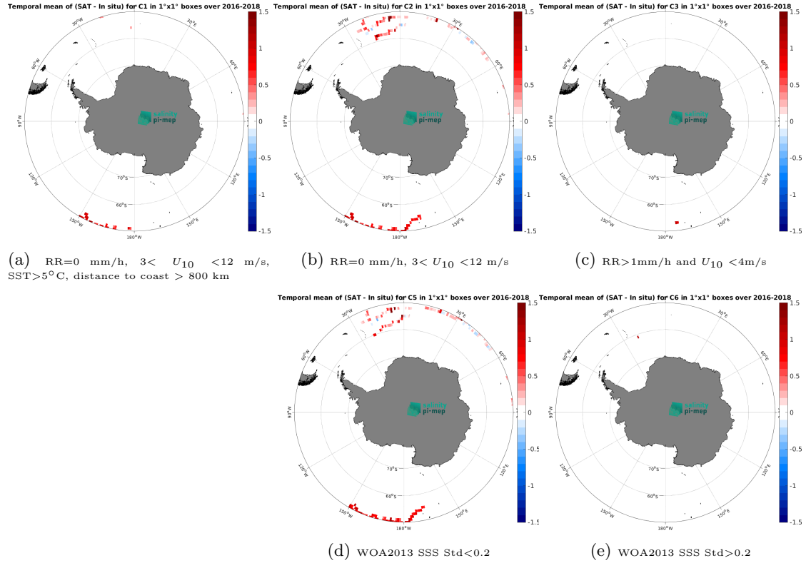
Figure 11: Temporal mean gridded over spatial boxes of size 1^{\circ}\times 1^{\circ} of \Delta\text{SSS} (SMOS SSS L3 v9 - 9 Days (CATDS-CEC-LOCEAN) - Surface drifters) for 5 different subdatasets corresponding to:RR=0 mm/h, 3 < U_{10} < 12 m/s, SST >5^{\circ}\text{C} , distance to coast > 800 km (a), RR=0 mm/h, 3 < U_{10} < 12 m/s (b), RR >1 mm/h and U_{10} < 4 m/s (c), WOA2013 SSS Std <0.2 (d), WOA2013 SSS Std >0.2 (e).
